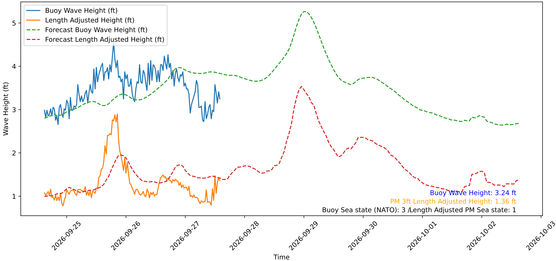
Wave Heights over Time for Green Beach at 2026-09-27 14:51:15
