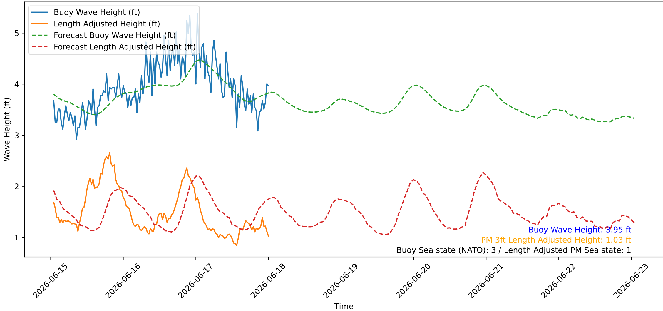
Wave Heights over Time for Red Beach at 2026-06-18 00:50:48
