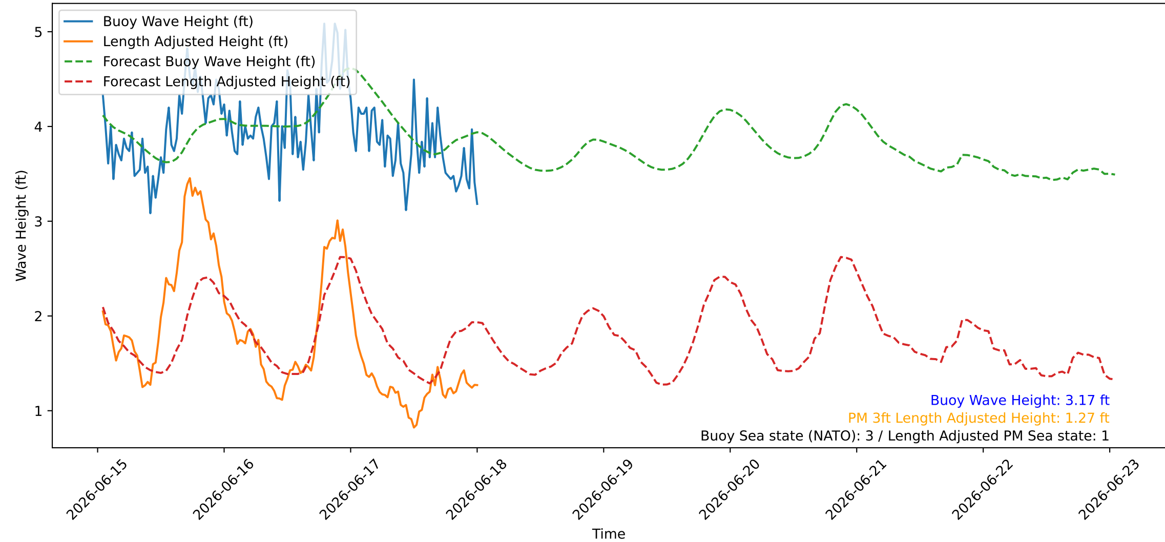
Wave Heights over Time for Green Beach at 2026-06-18 00:51:10
