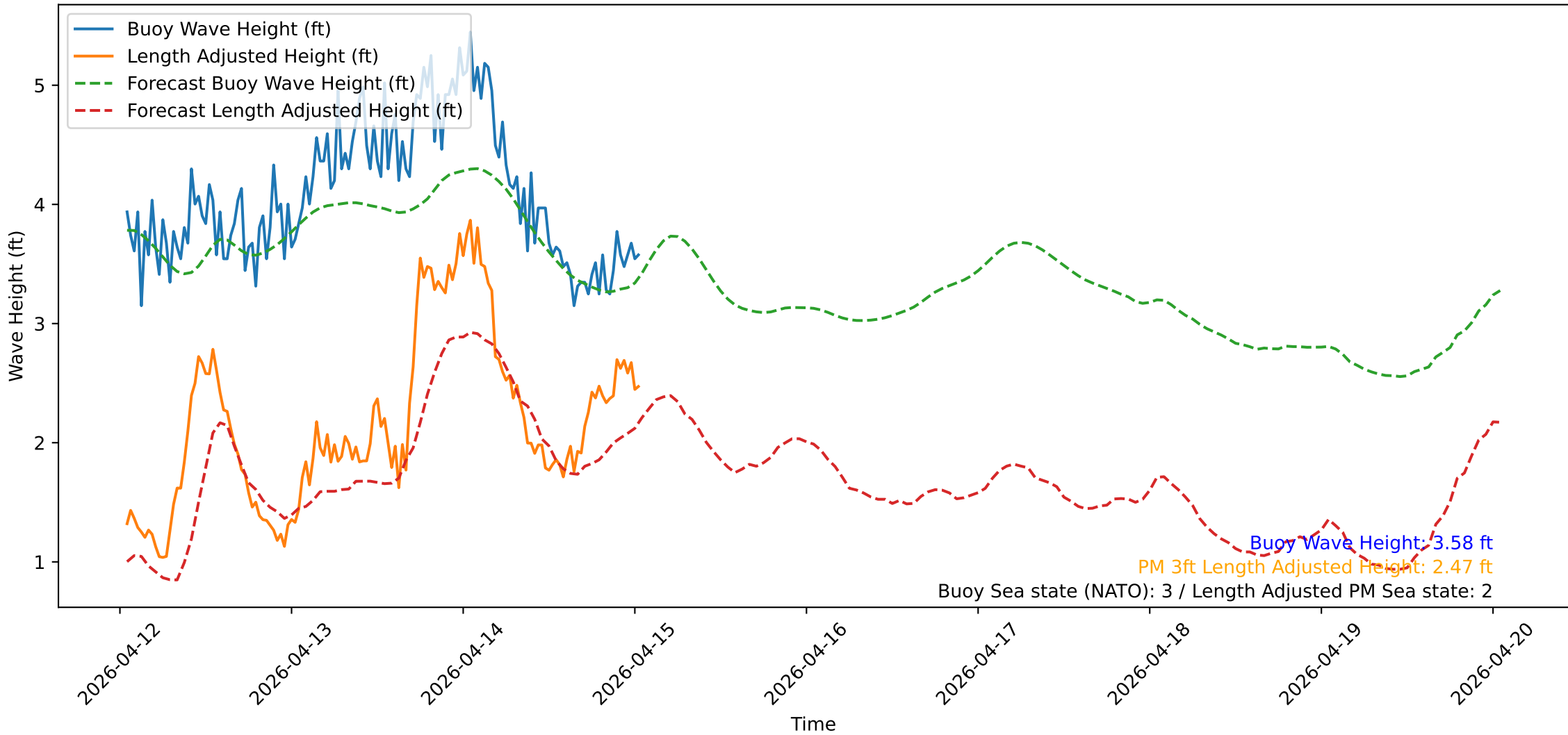
Wave Heights over Time for Oceanside Harbor at 2026-04-15 01:00:31
