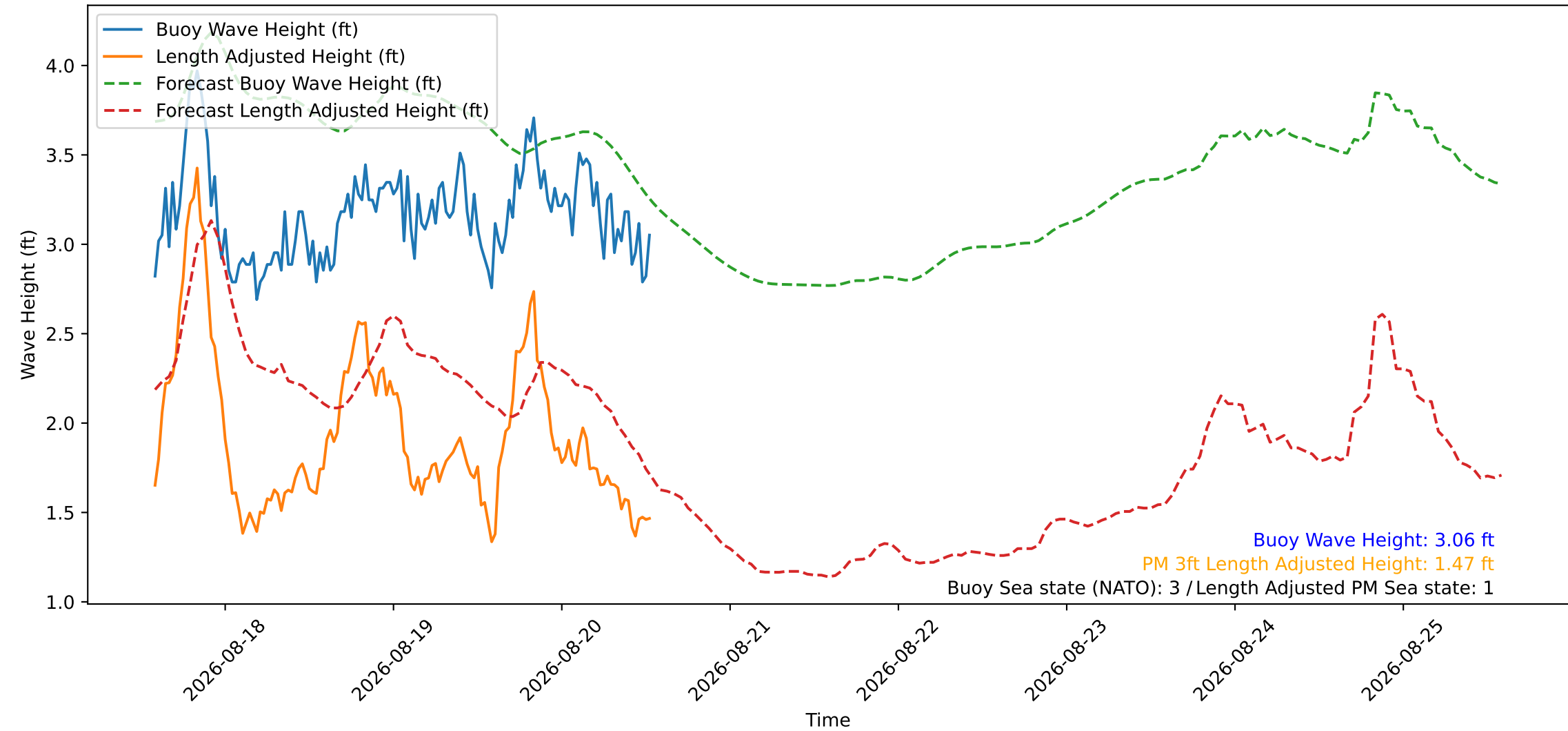
Wave Heights over Time for Green Beach at 2026-08-20 13:31:08
