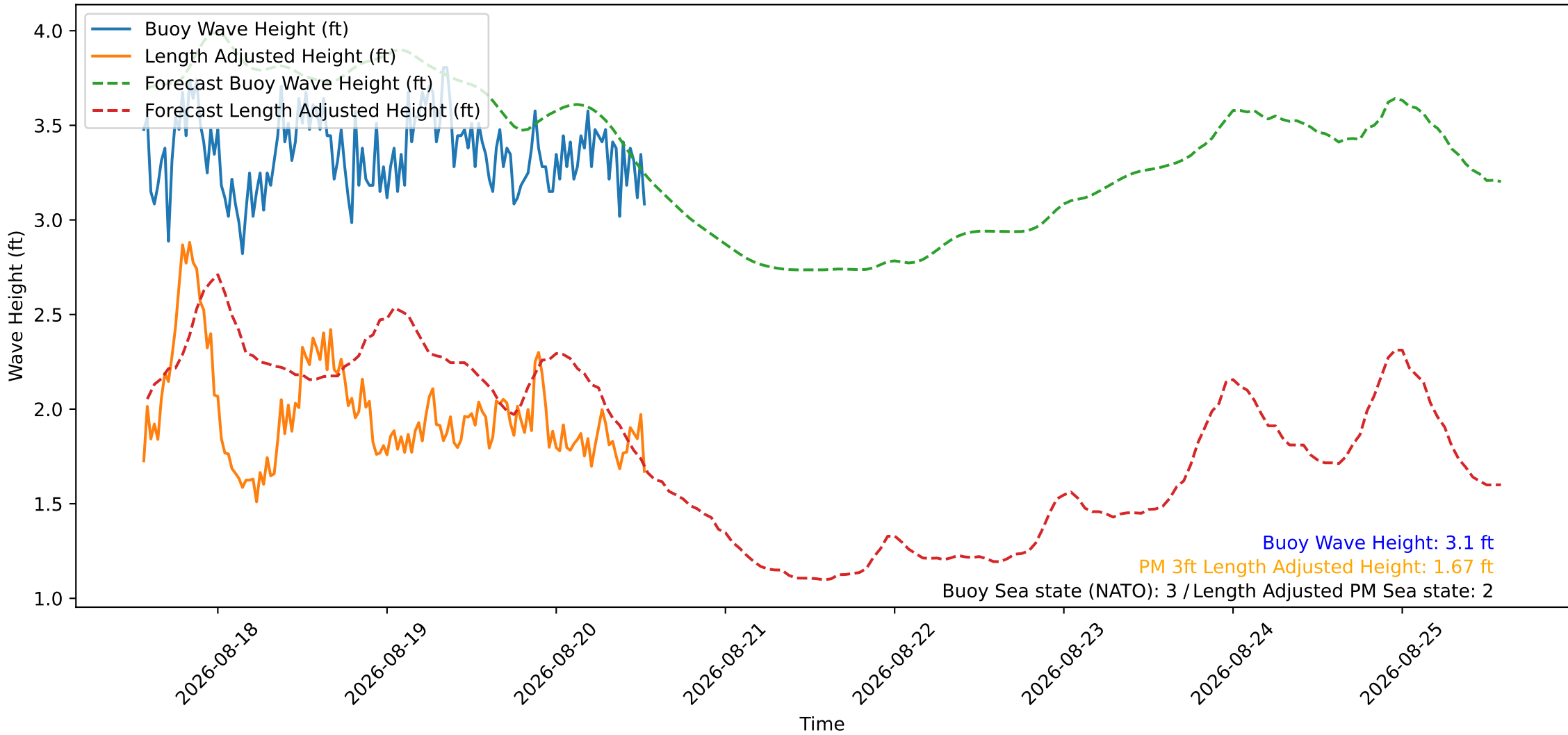
Wave Heights over Time for Oceanside Harbor at 2026-08-20 13:30:26
