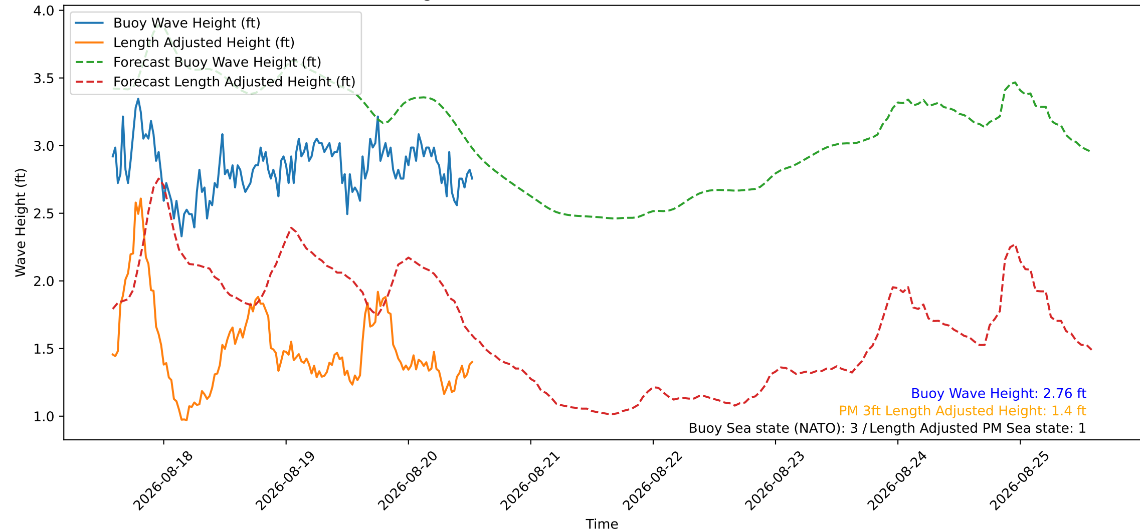
Wave Heights over Time for Red Beach at 2026-08-20 13:30:46
