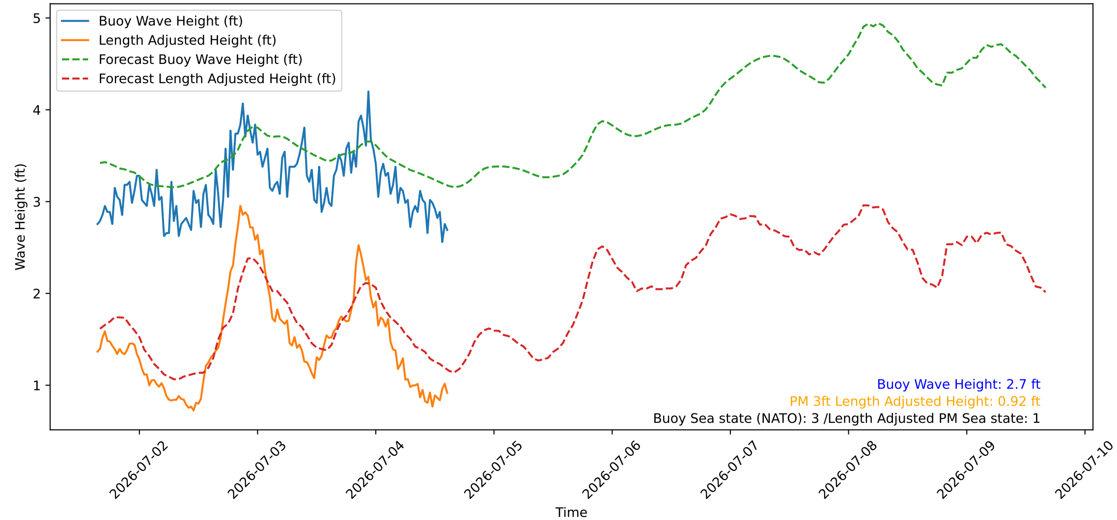
Wave Heights over Time for Green Beach at 2026-07-04 15:31:08
