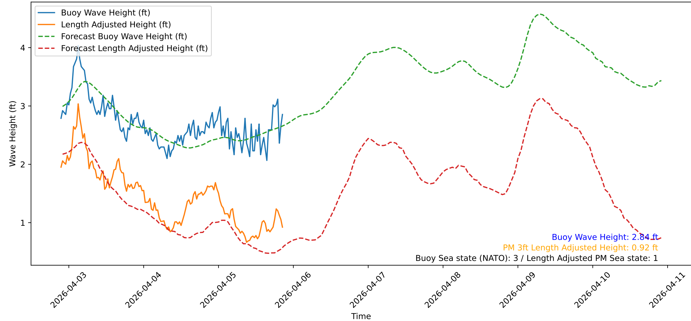
Wave Heights over Time for Oceanside Harbor at 2026-04-05 21:30:39
