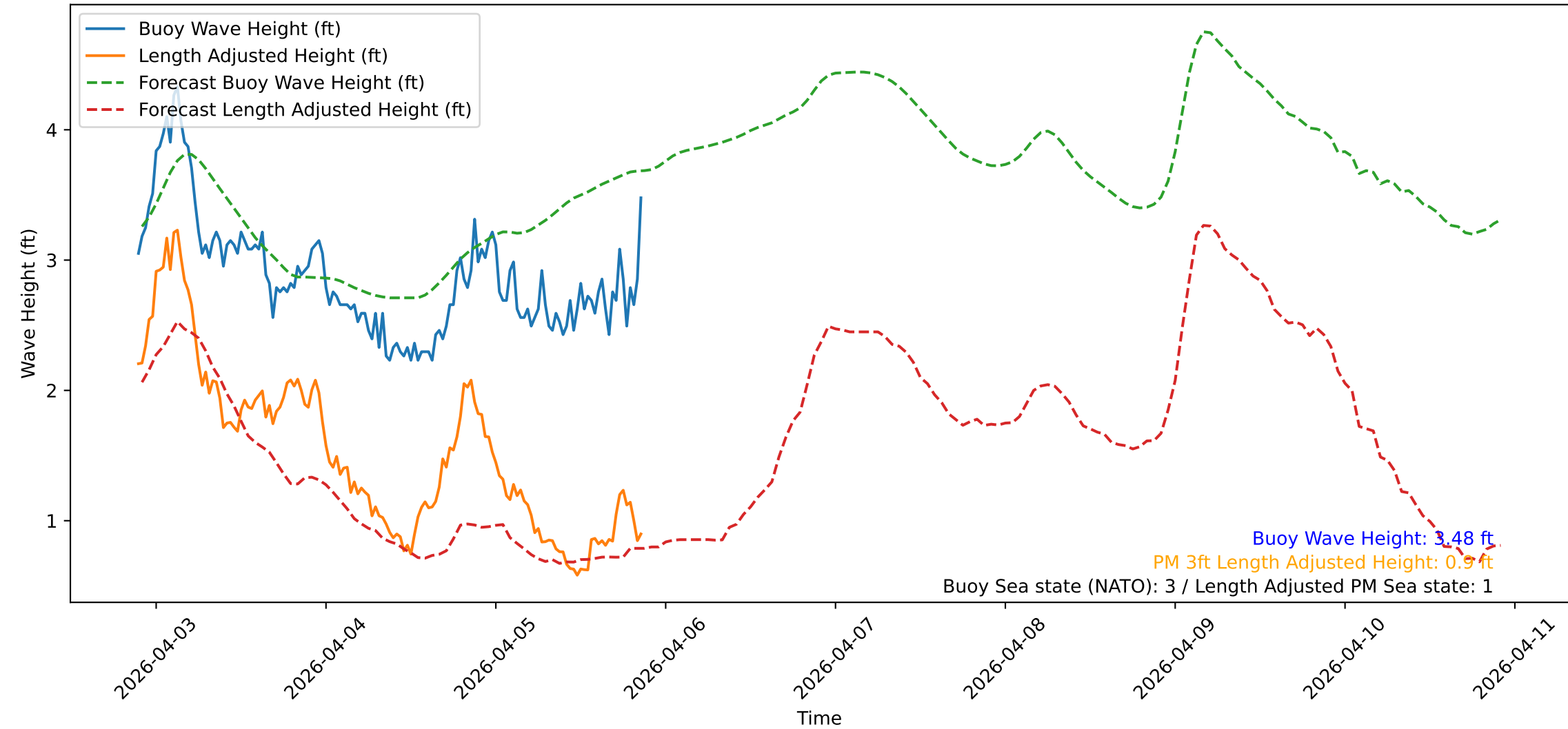
Wave Heights over Time for Green Beach at 2026-04-05 21:31:31
