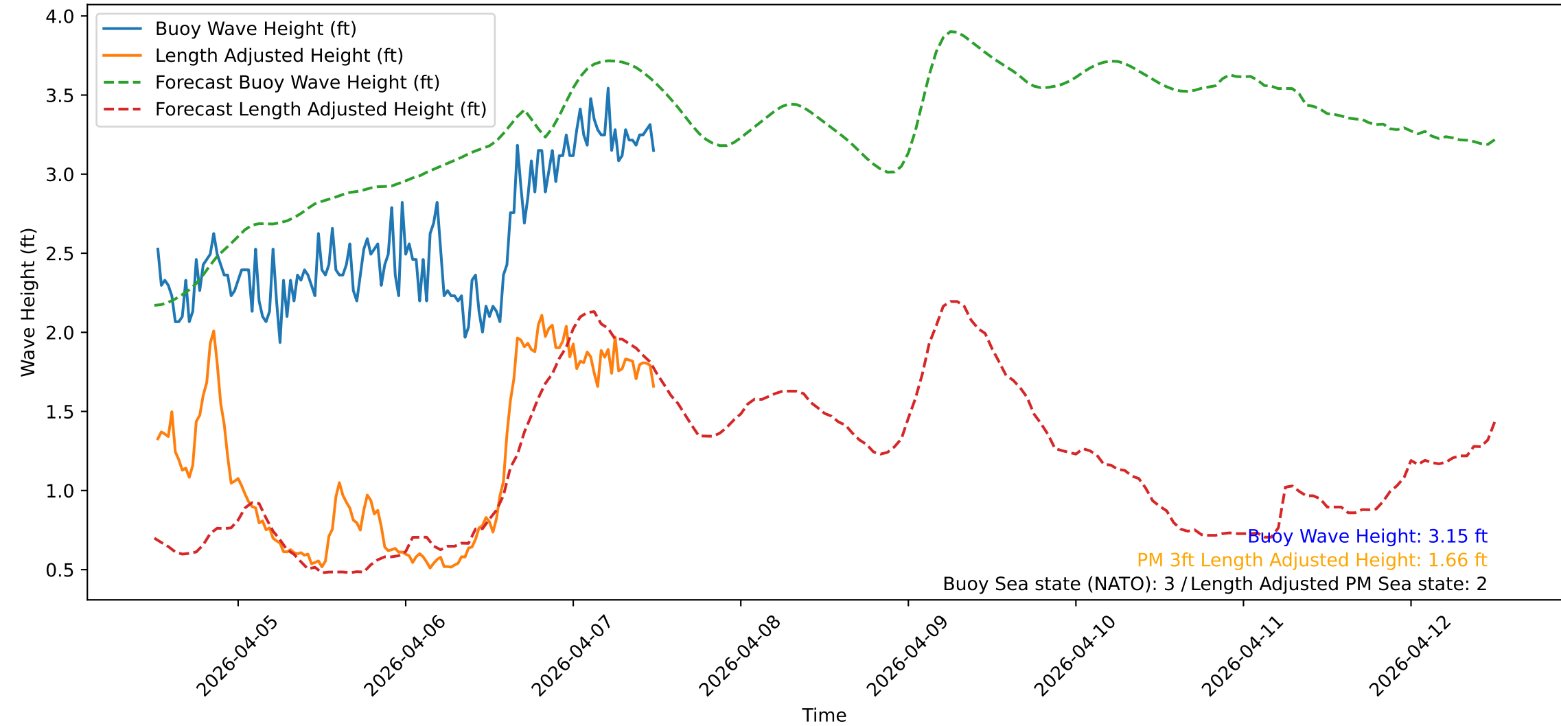
Wave Heights over Time for Red Beach at 2026-04-07 12:10:48
