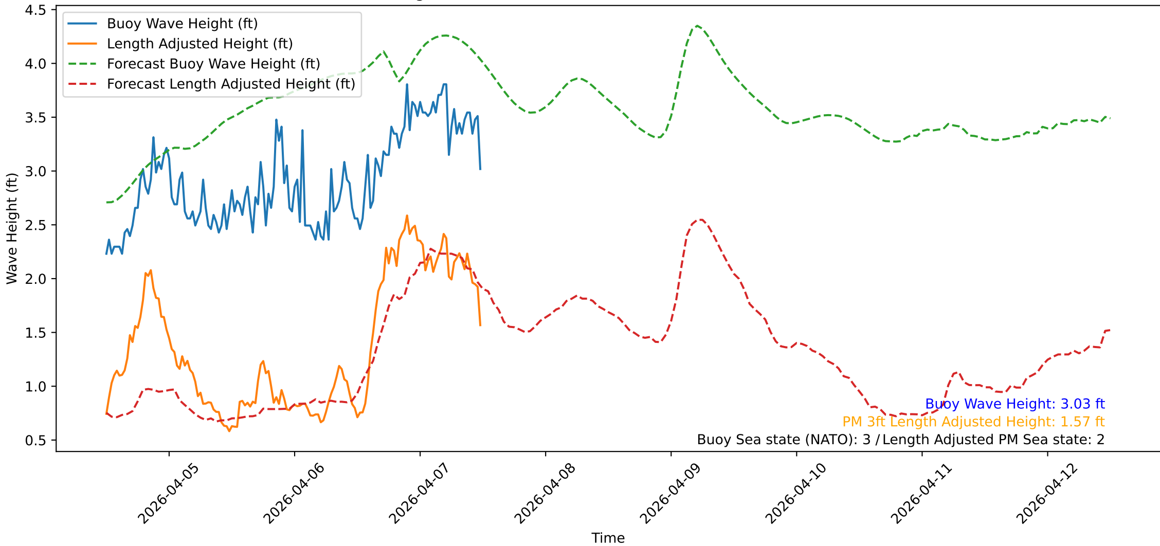
Wave Heights over Time for Green Beach at 2026-04-07 12:11:11
