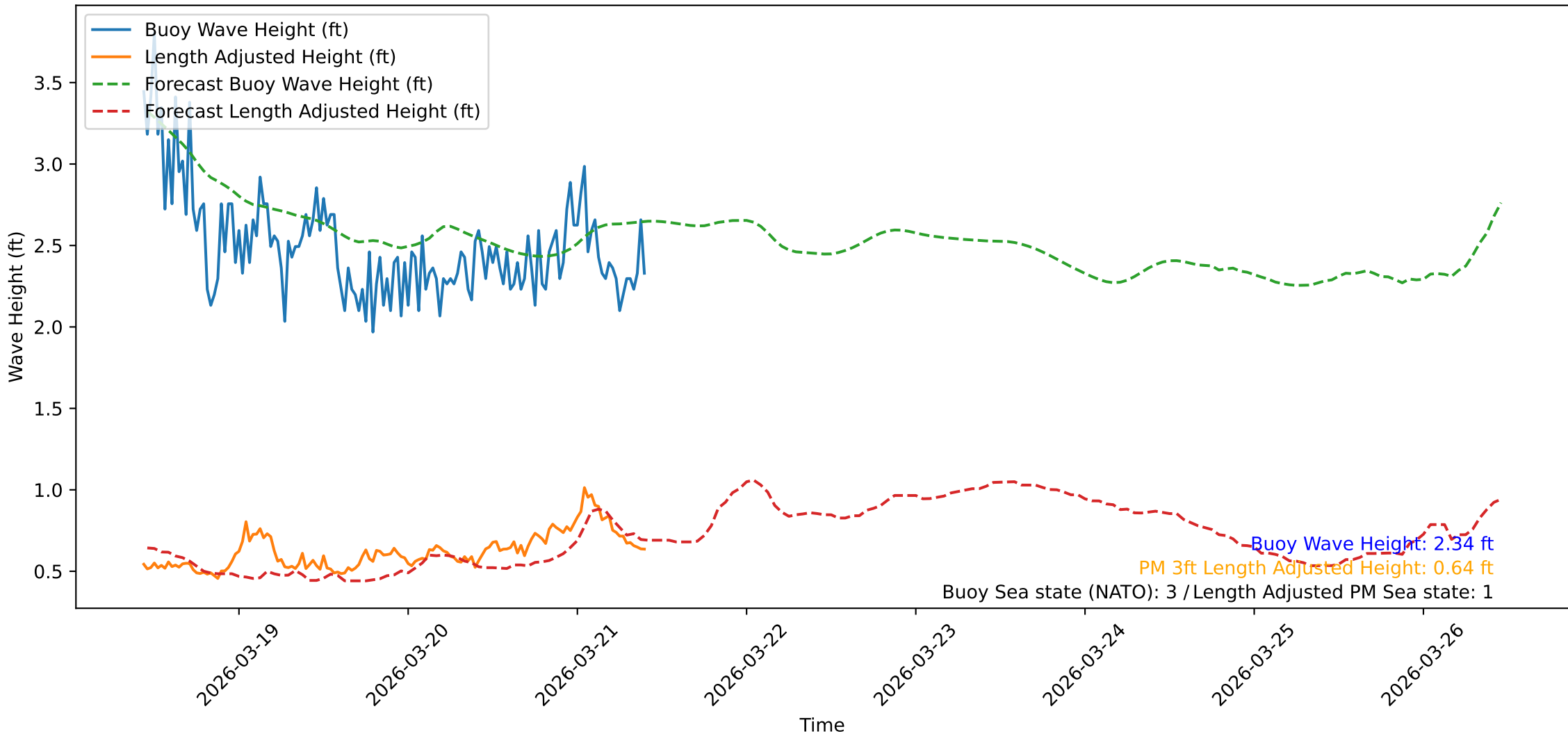
Wave Heights over Time for Oceanside Harbor at 2026-03-21 10:30:32
