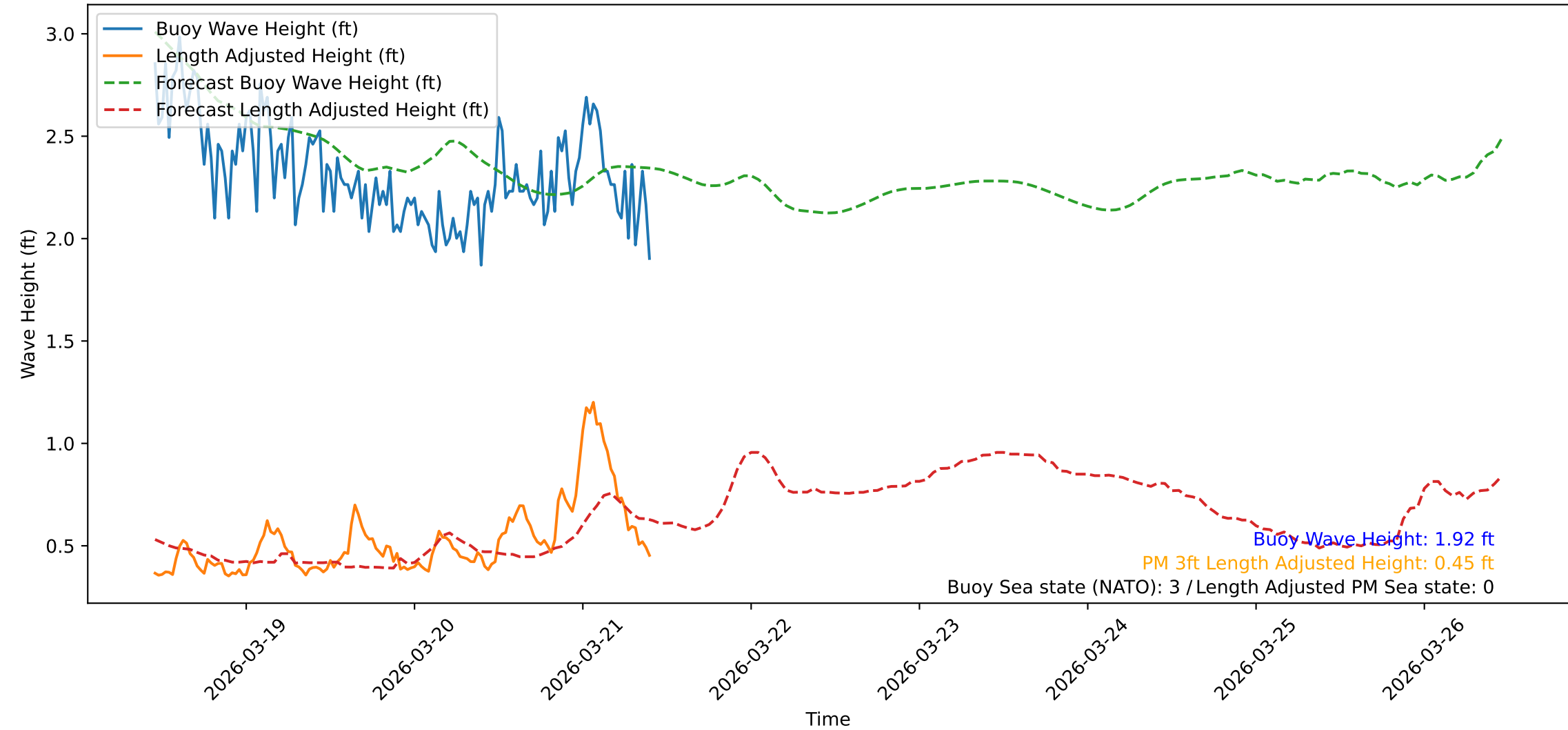
Wave Heights over Time for Red Beach at 2026-03-21 10:30:48
