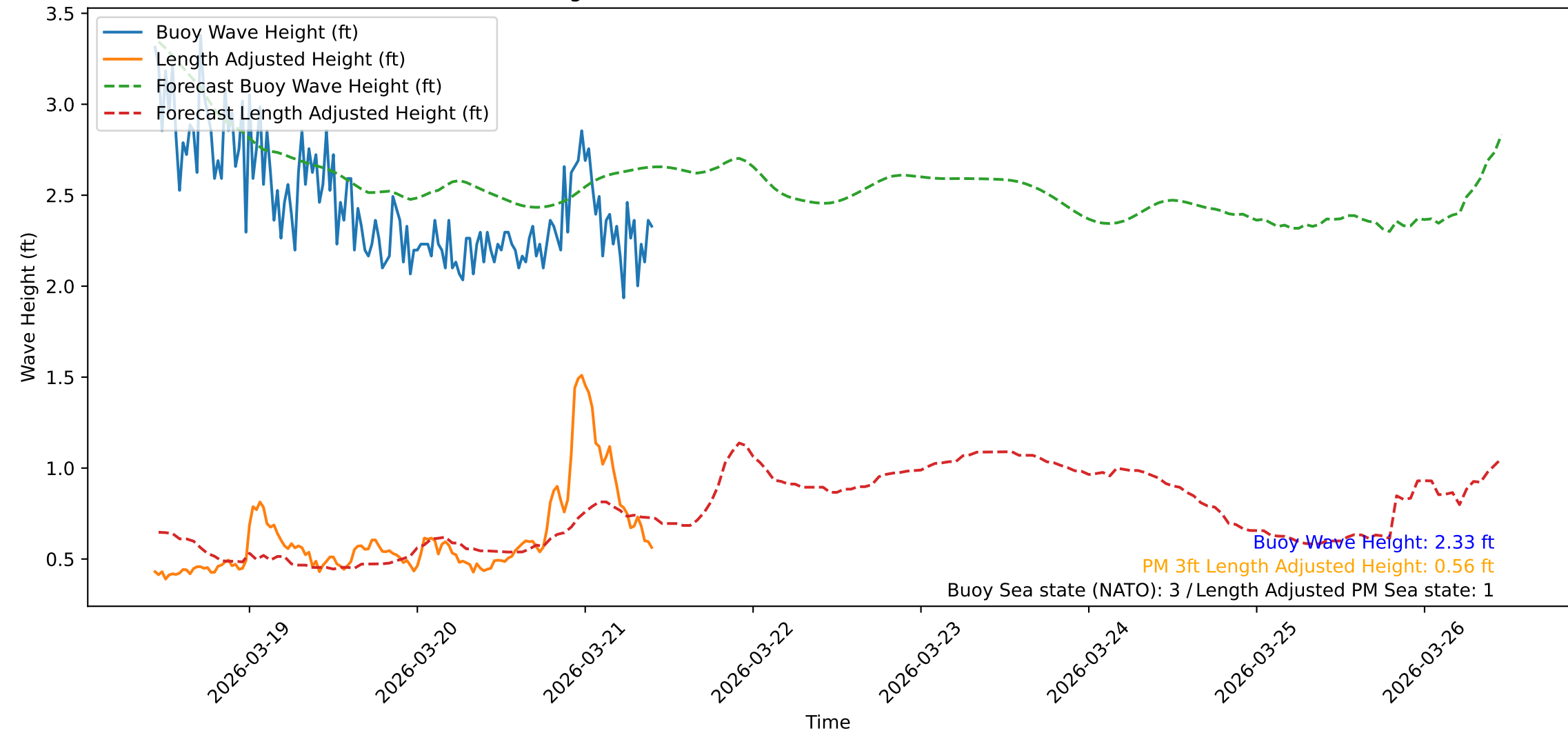
Wave Heights over Time for Green Beach at 2026-03-21 10:31:10
