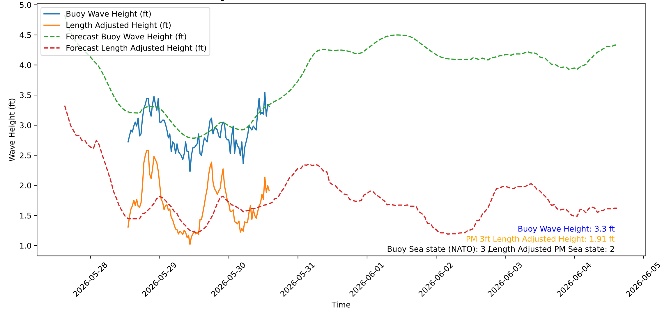
Wave Heights over Time for Oceanside Harbor at 2026-05-30 14:40:24
