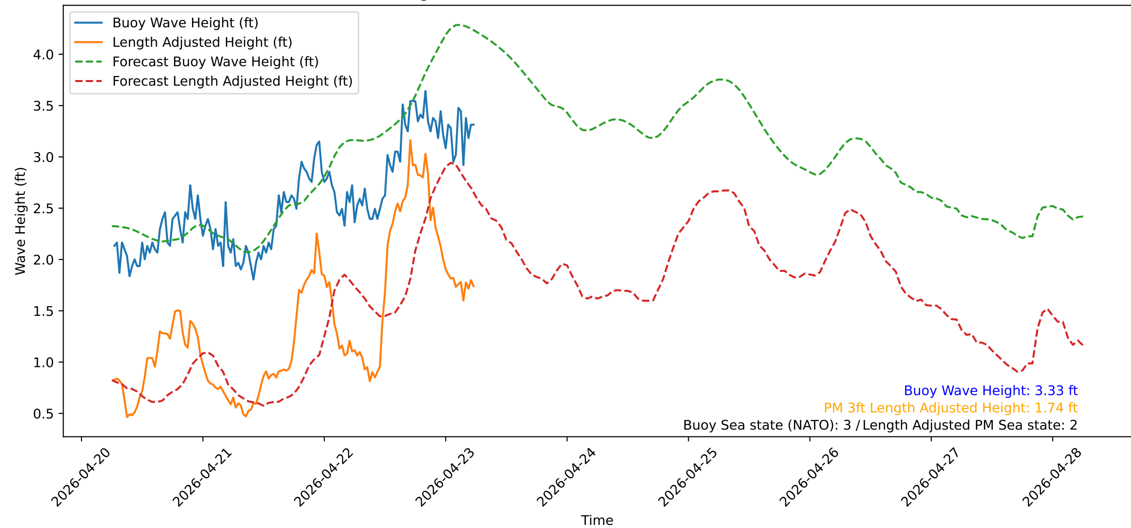
Wave Heights over Time for Red Beach at 2026-04-23 06:20:51
