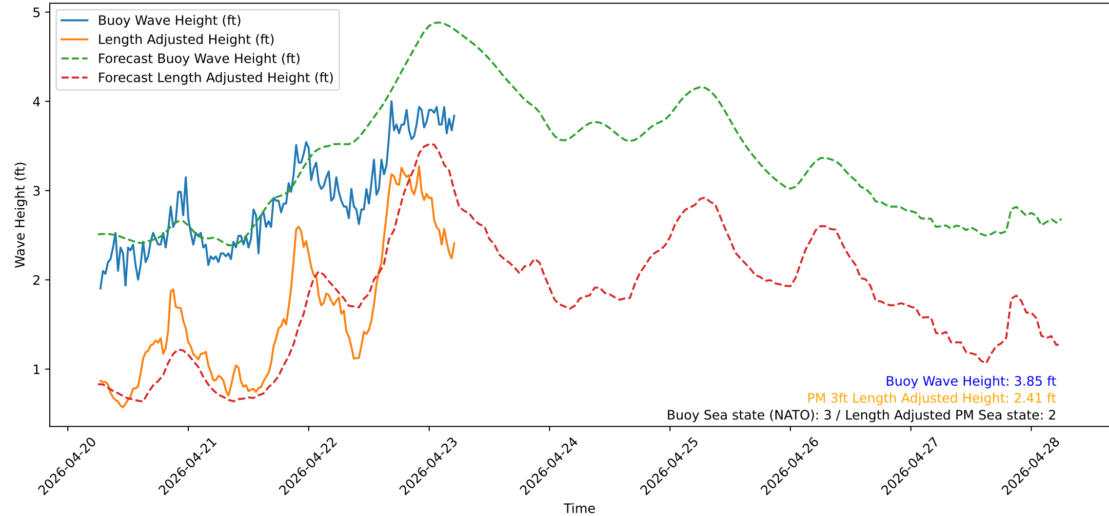
Wave Heights over Time for Green Beach at 2026-04-23 06:21:12
