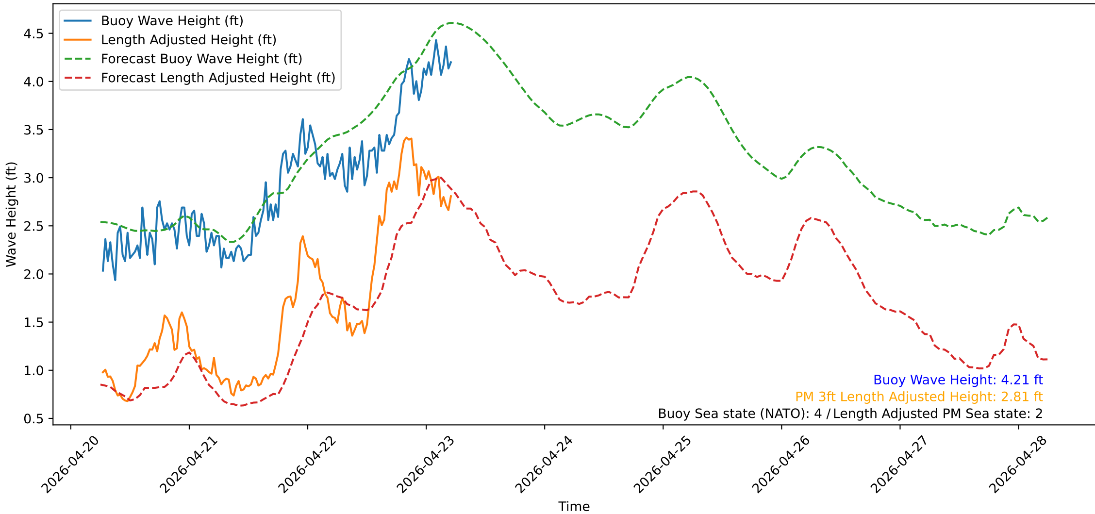
Wave Heights over Time for Oceanside Harbor at 2026-04-23 06:20:31
