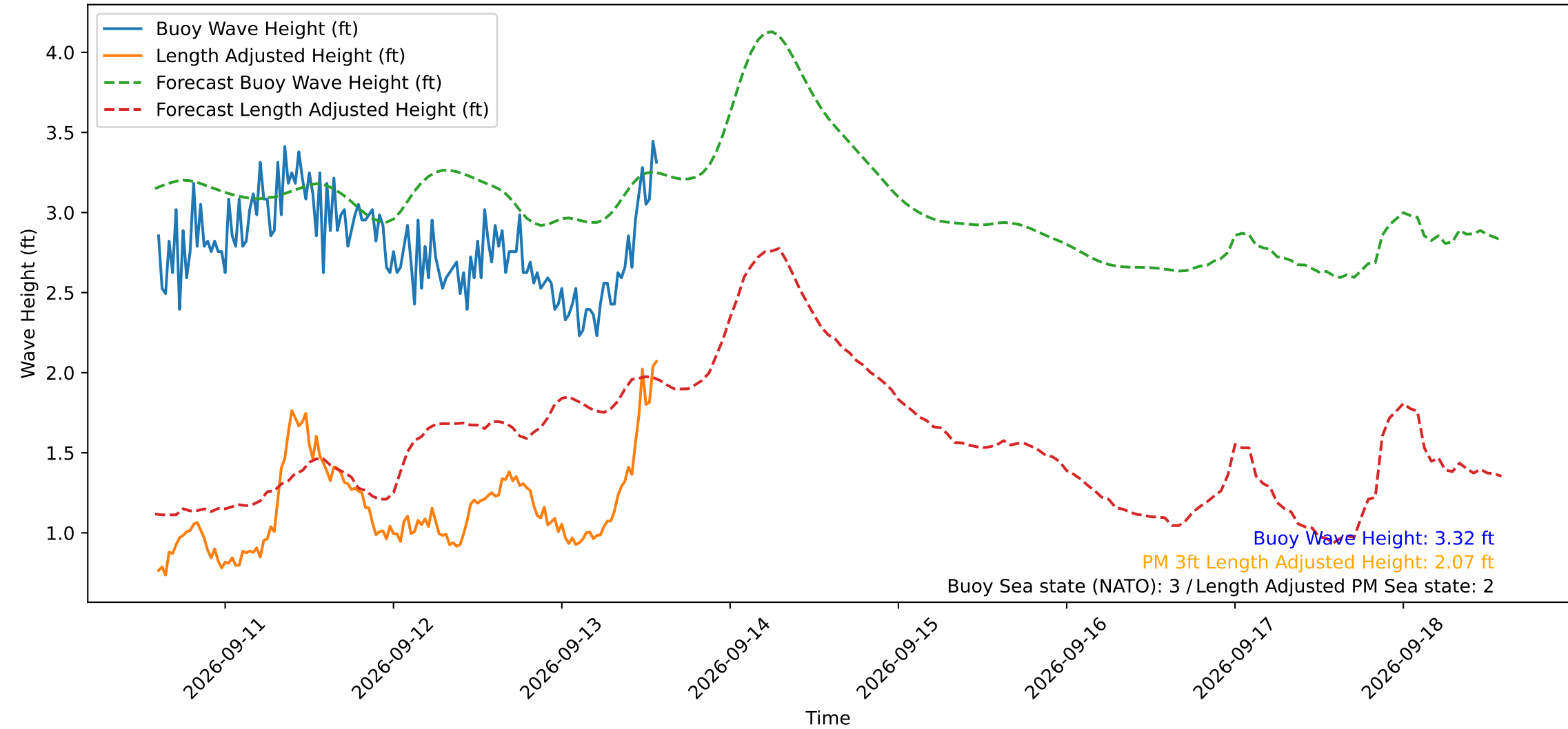
Wave Heights over Time for Red Beach at 2026-09-13 14:10:50
