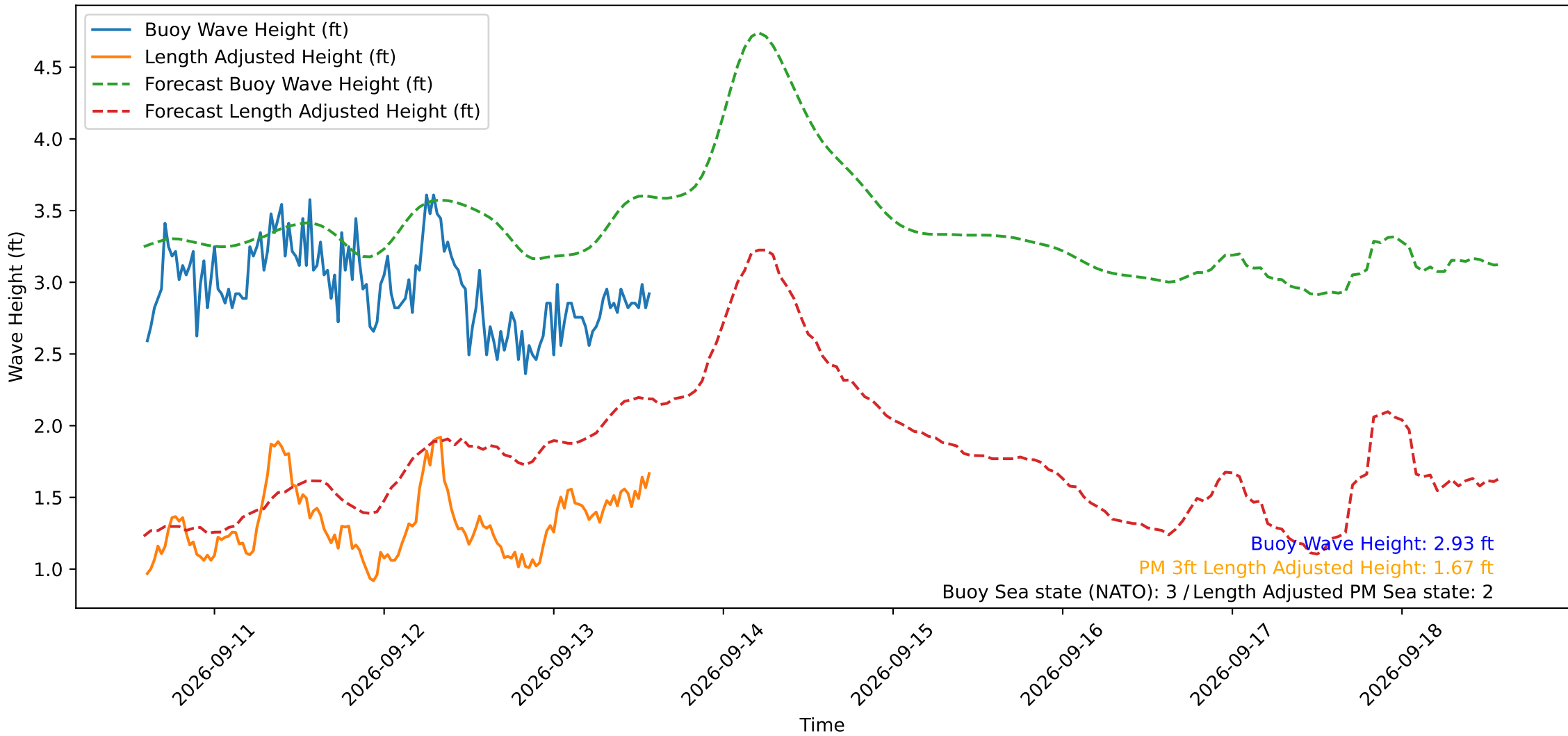
Wave Heights over Time for Green Beach at 2026-09-13 14:11:12
