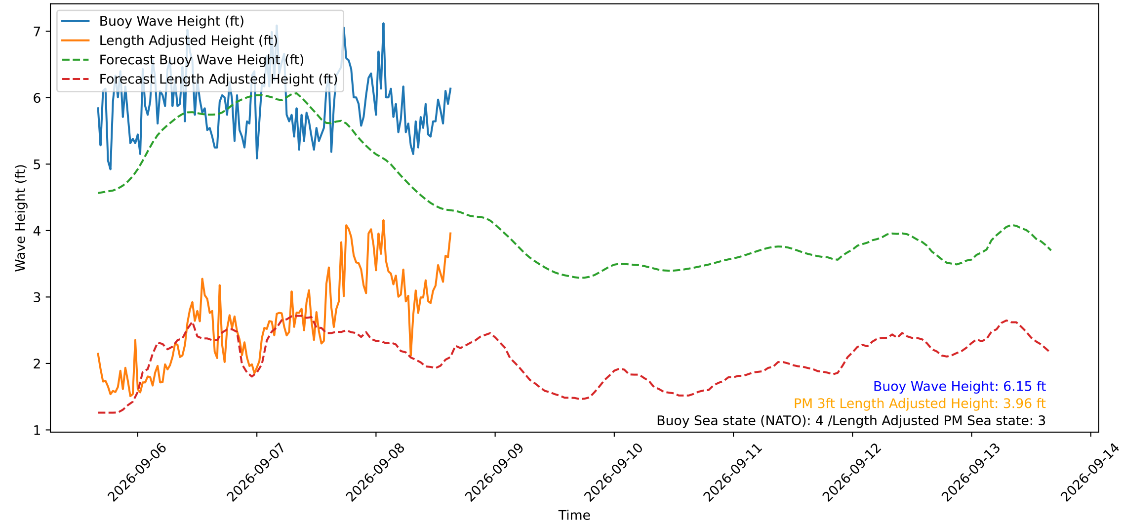
Wave Heights over Time for Oceanside Harbor at 2026-09-08 15:50:30
