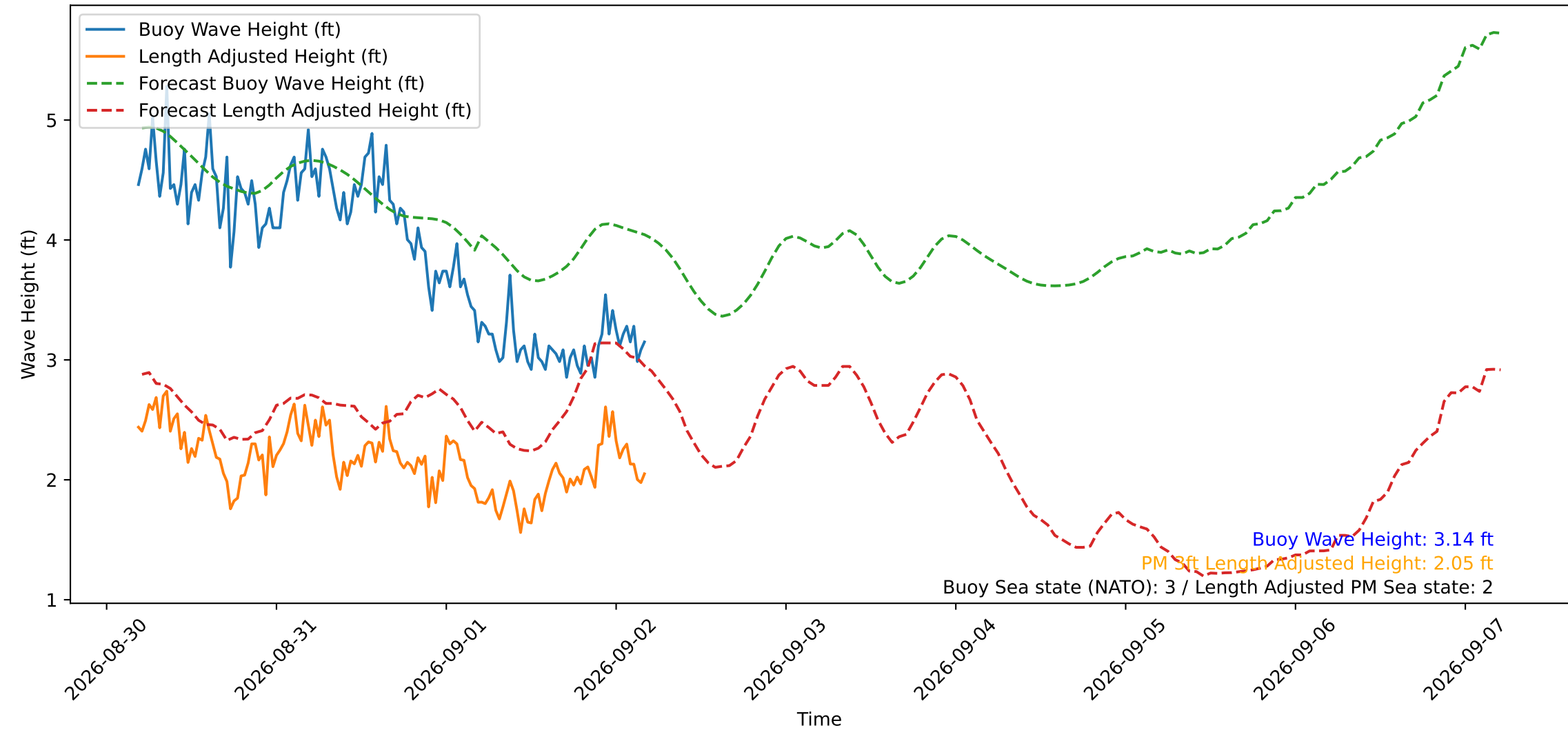
Wave Heights over Time for Oceanside Harbor at 2026-09-02 04:40:29
