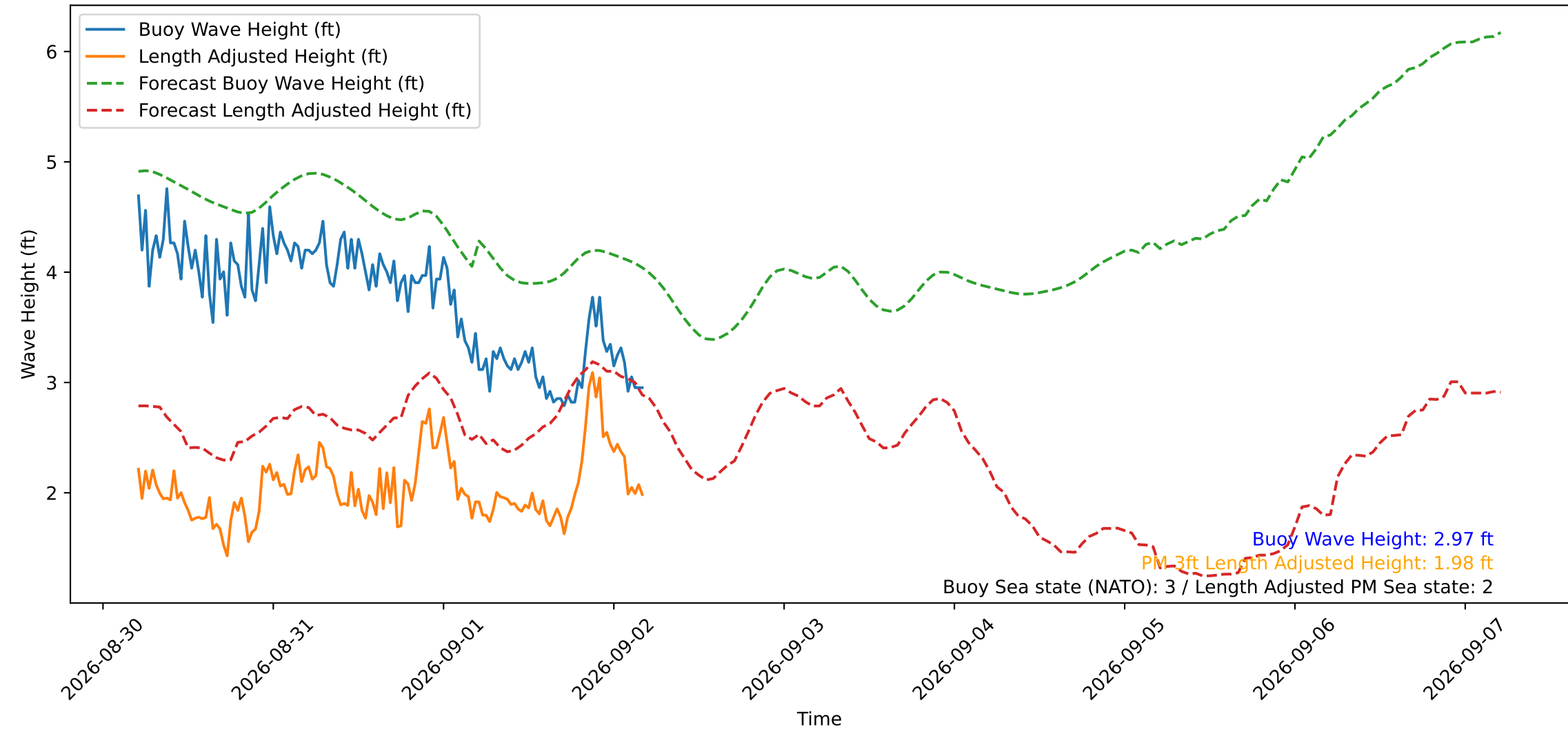
Wave Heights over Time for Green Beach at 2026-09-02 04:41:13
