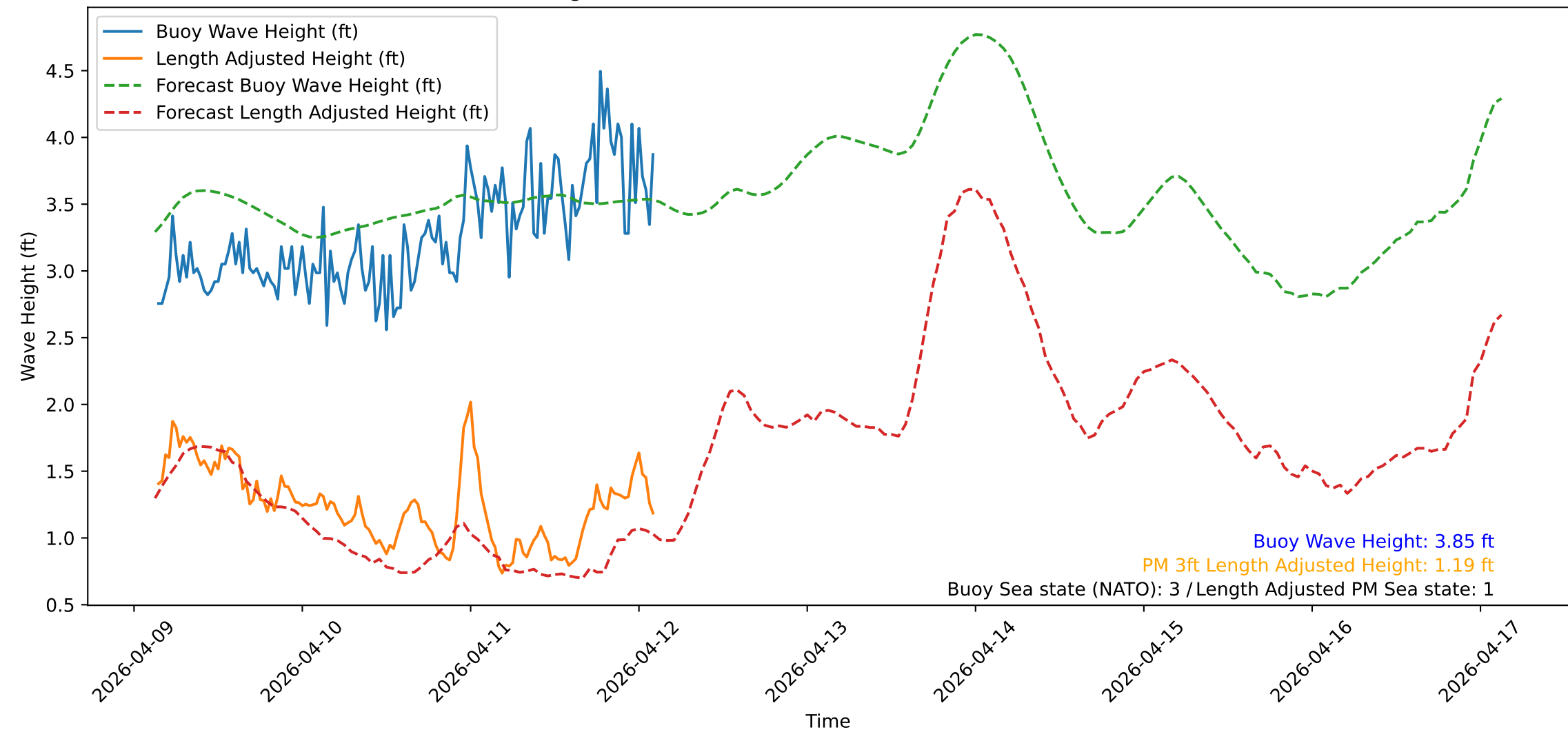
Wave Heights over Time for Green Beach at 2026-04-12 03:21:15
