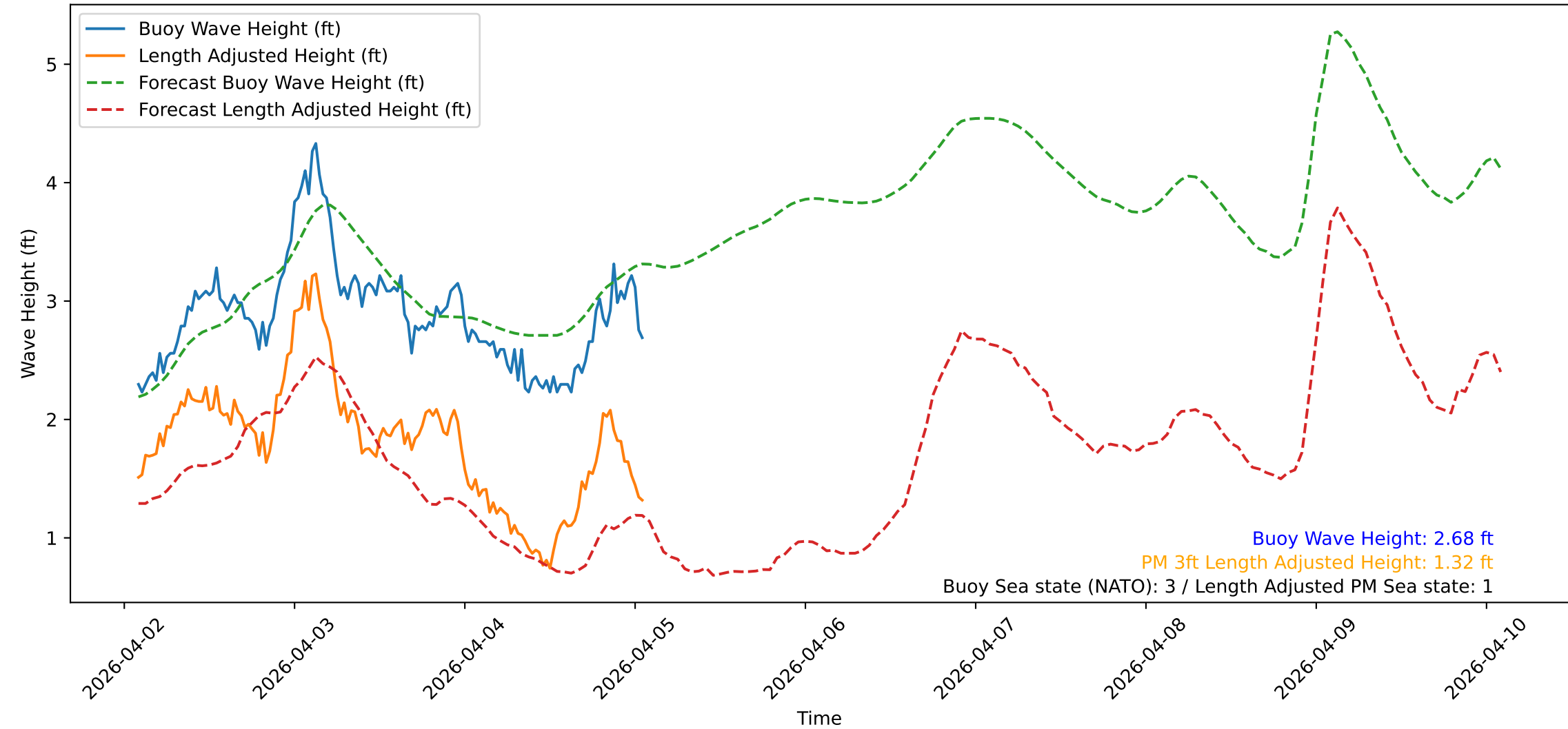
Wave Heights over Time for Green Beach at 2026-04-05 02:01:10
