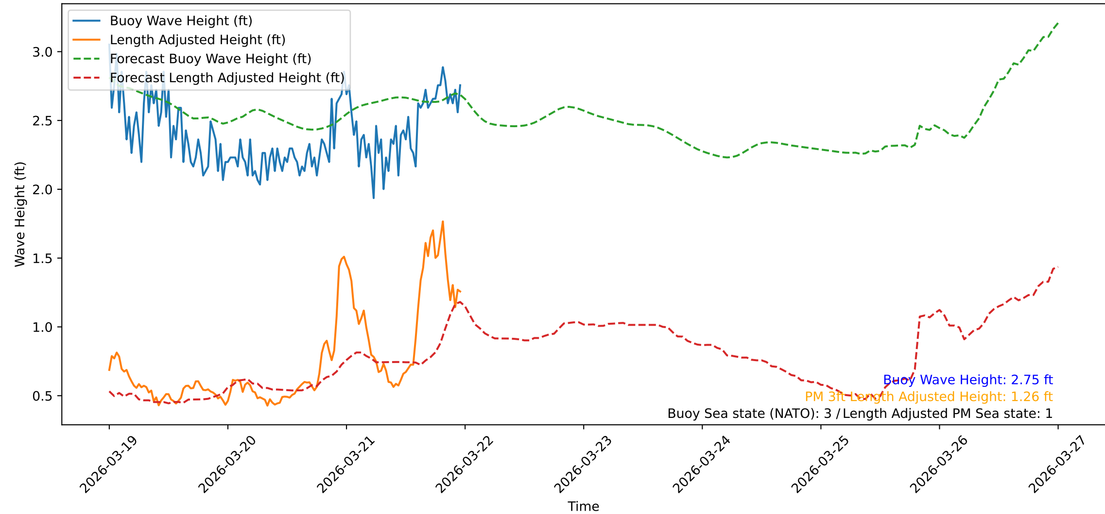
Wave Heights over Time for Green Beach at 2026-03-22 00:01:10
