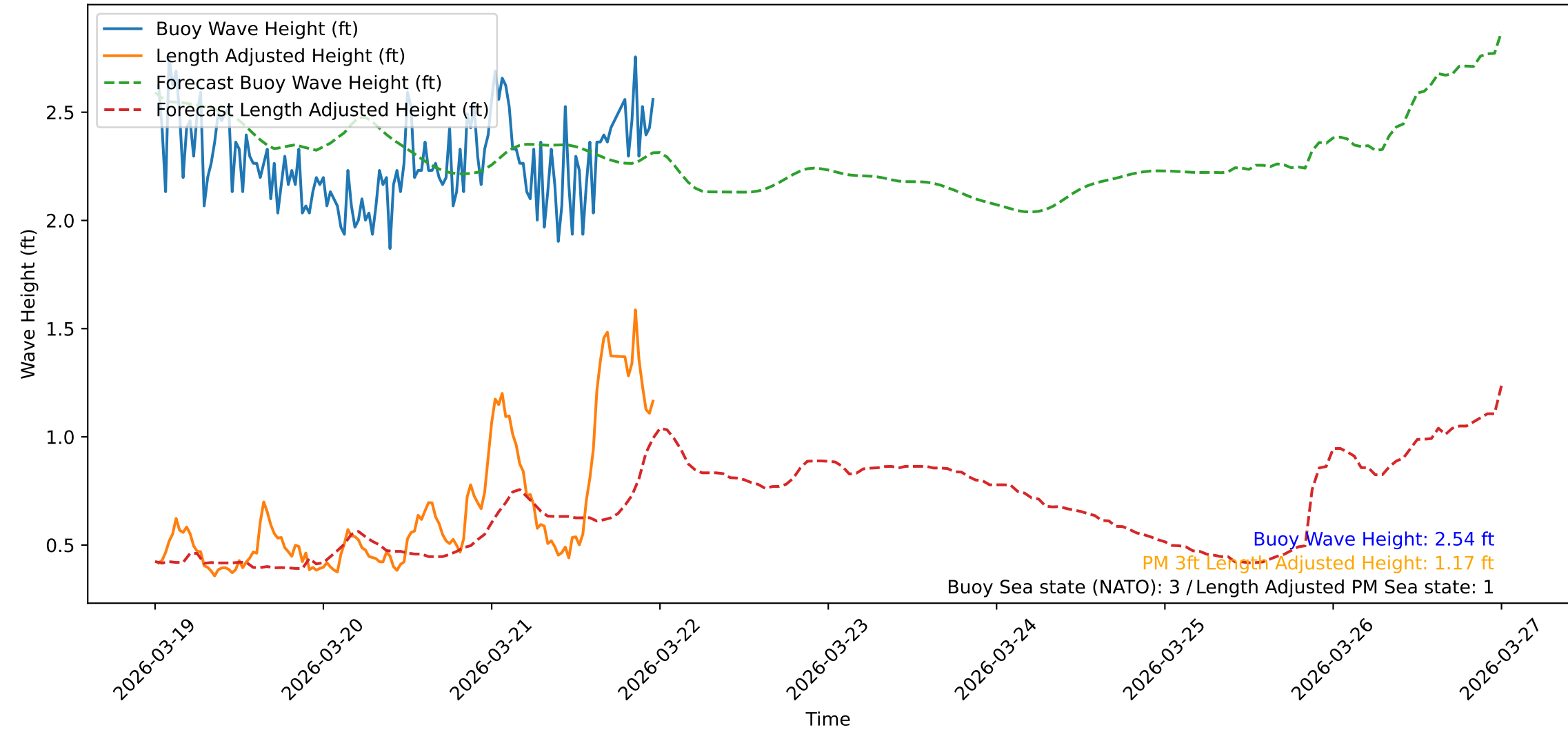
Wave Heights over Time for Red Beach at 2026-03-22 00:00:47
