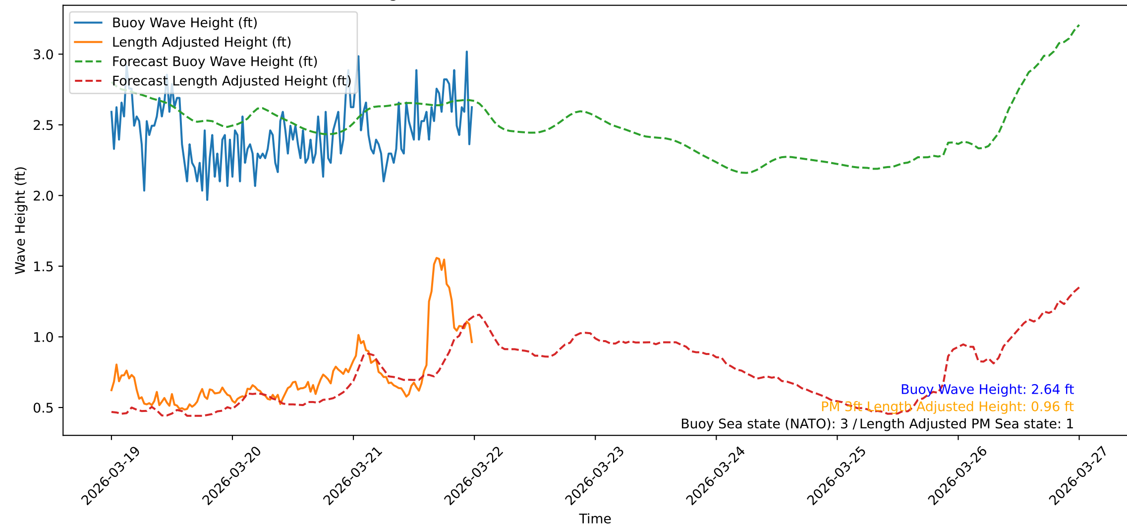
Wave Heights over Time for Oceanside Harbor at 2026-03-22 00:00:31
