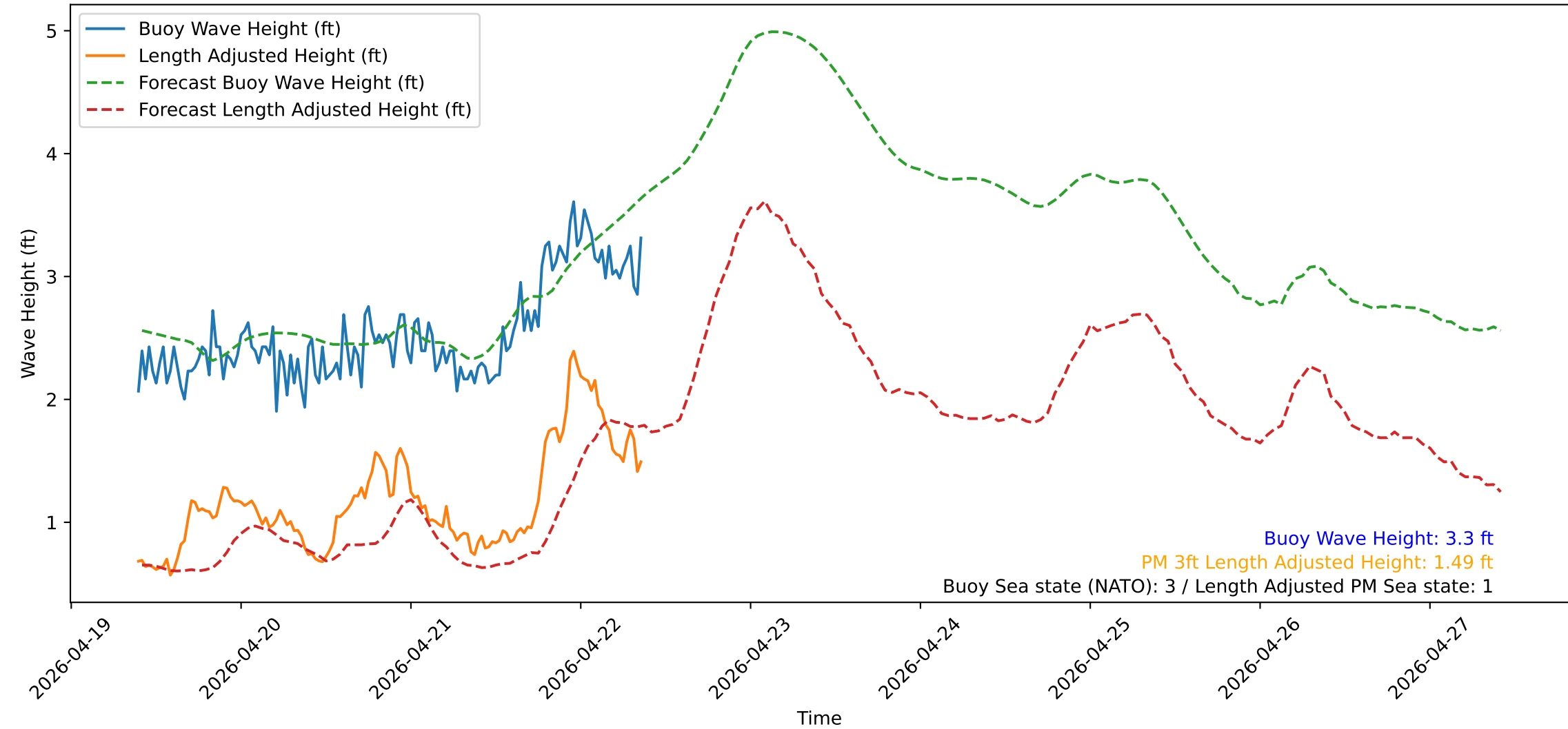
Wave Heights over Time for Oceanside Harbor at 2026-04-22 09:30:32
