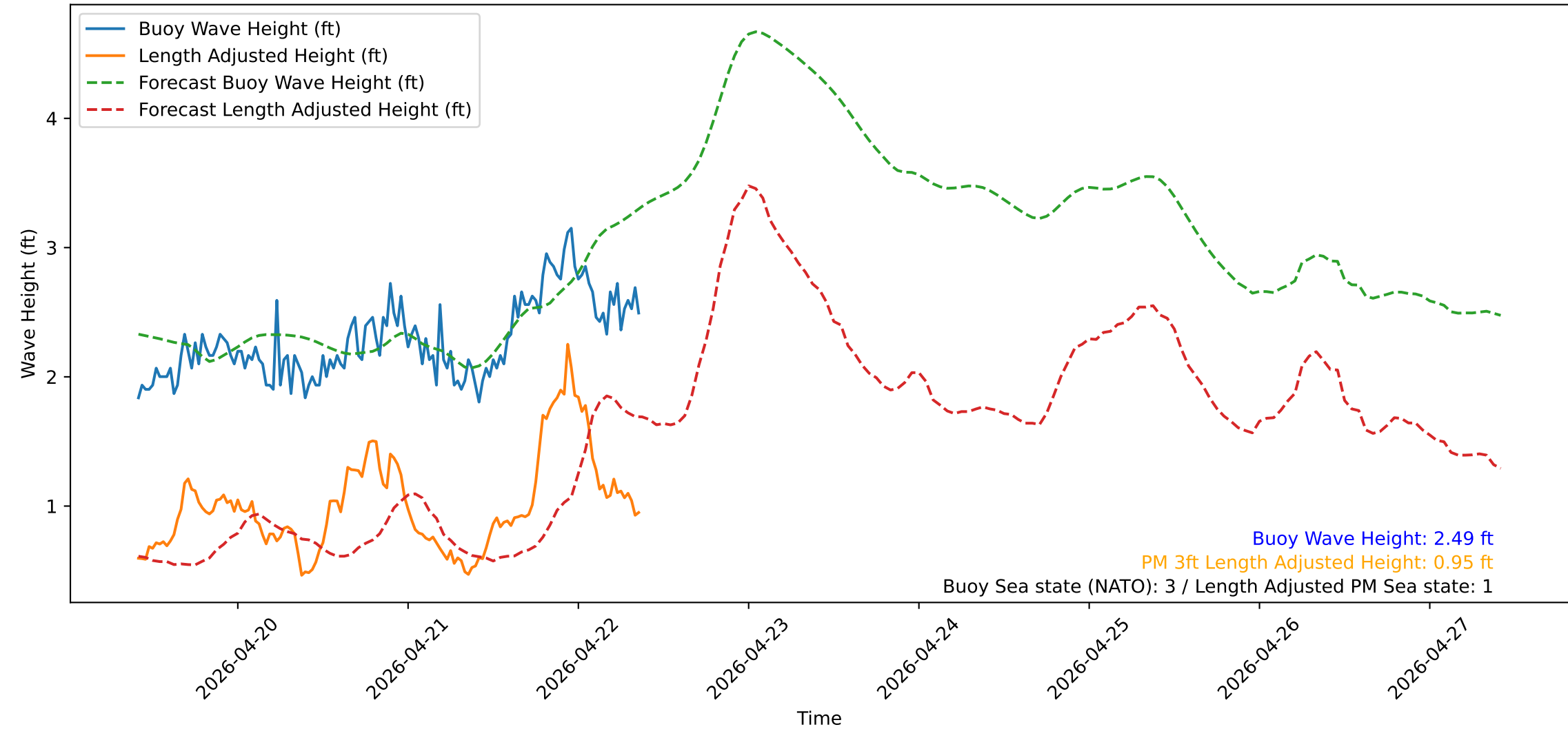
Wave Heights over Time for Red Beach at 2026-04-22 09:30:51
