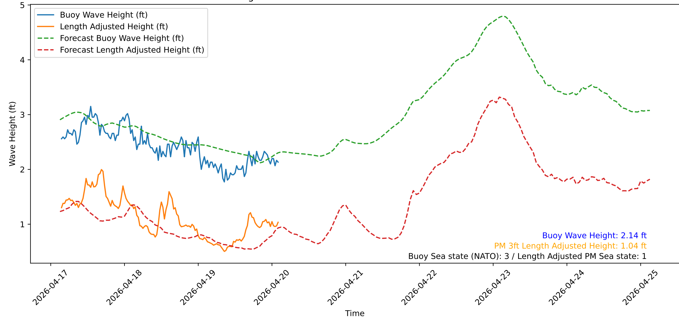
Wave Heights over Time for Red Beach at 2026-04-20 03:00:51
