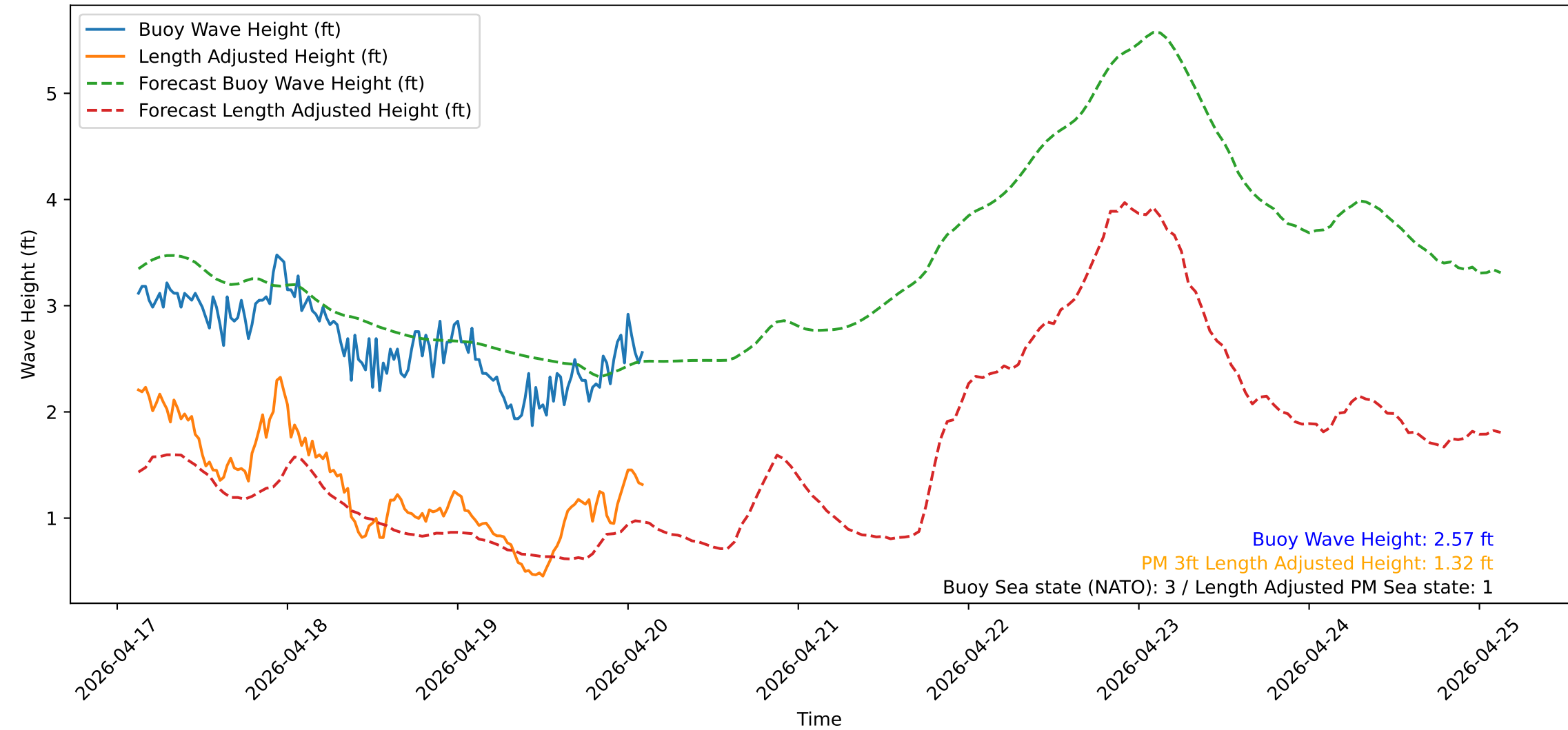
Wave Heights over Time for Green Beach at 2026-04-20 03:01:13
