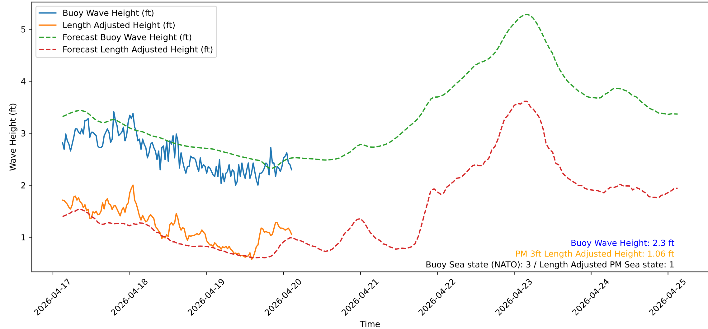
Wave Heights over Time for Oceanside Harbor at 2026-04-20 03:00:32
