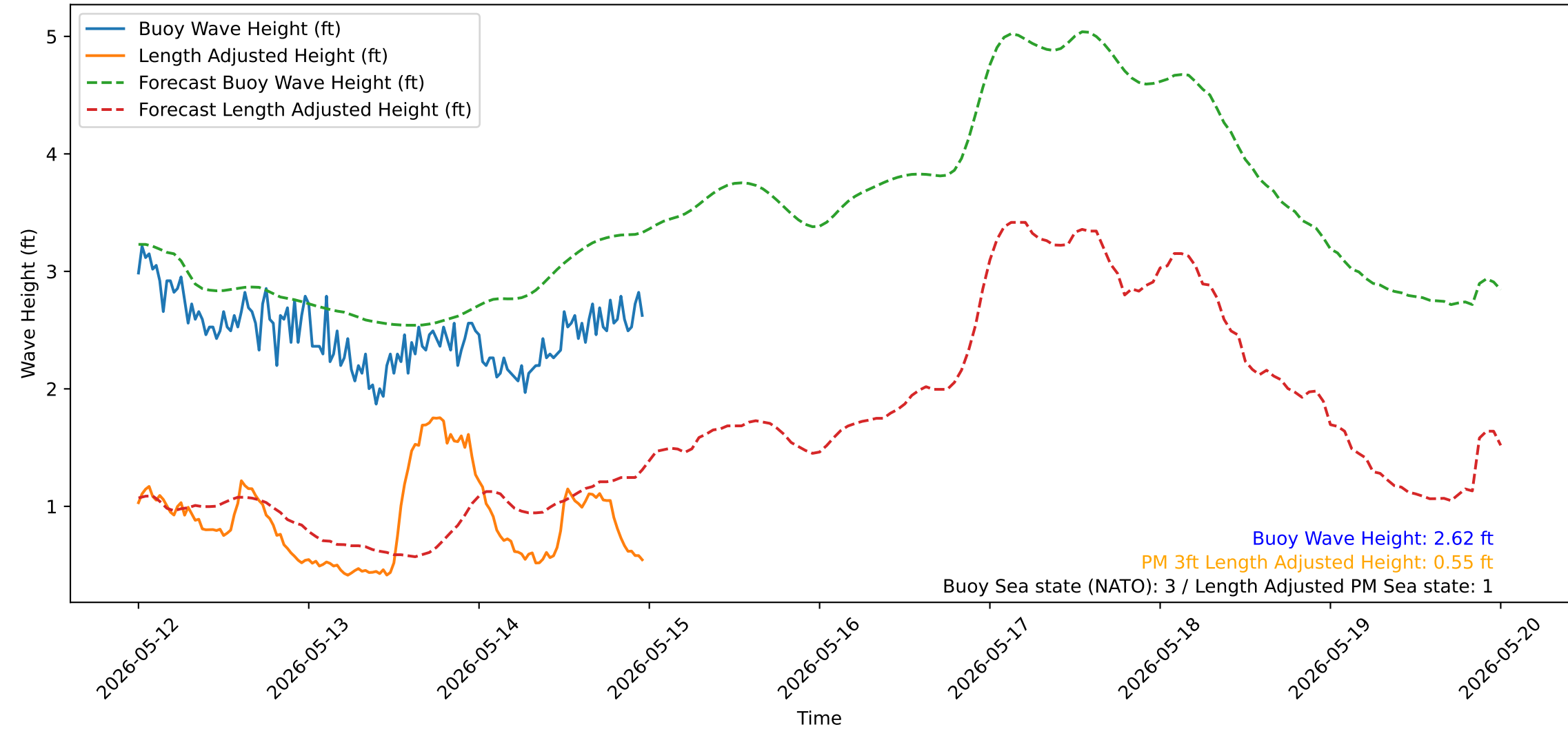
Wave Heights over Time for Red Beach at 2026-05-14 23:50:52
