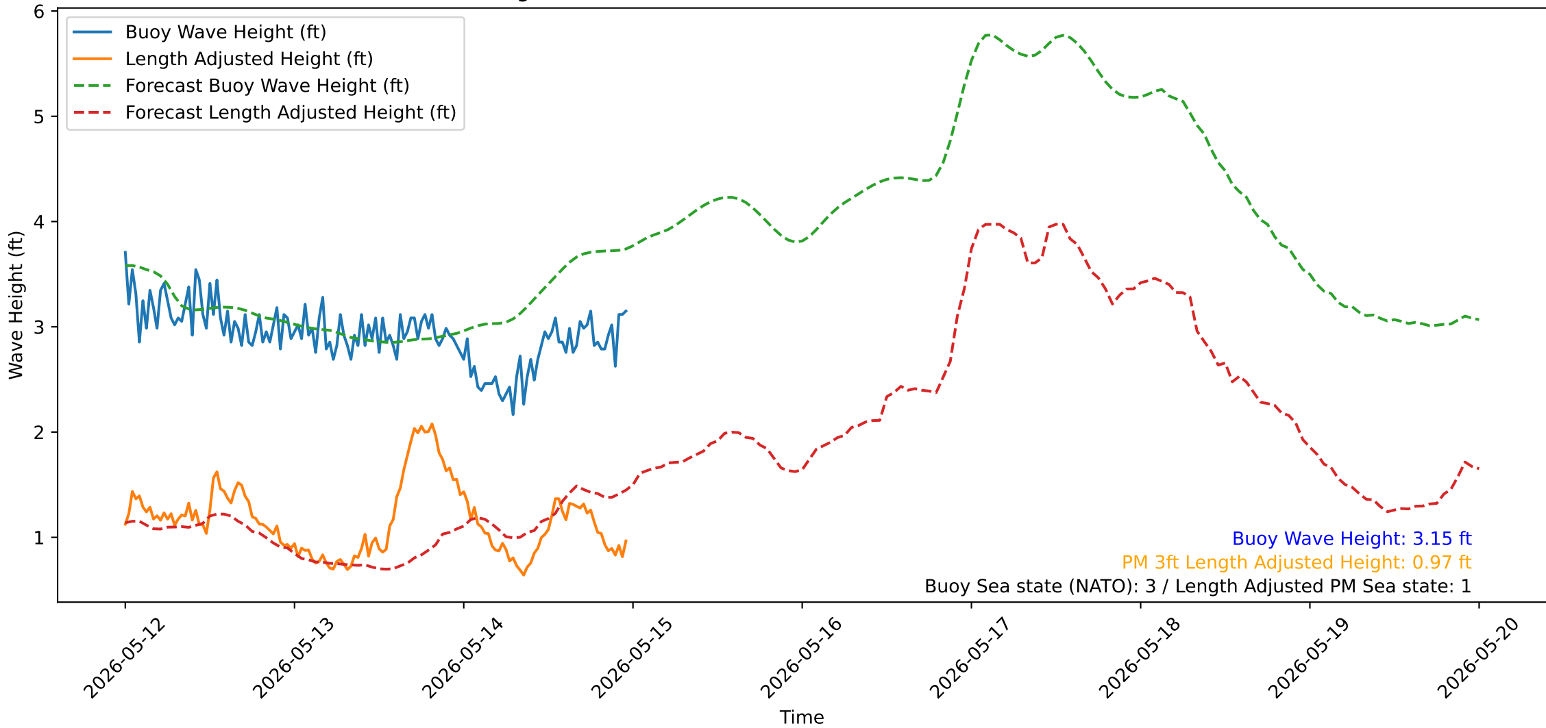
Wave Heights over Time for Oceanside Harbor at 2026-05-14 23:50:31
