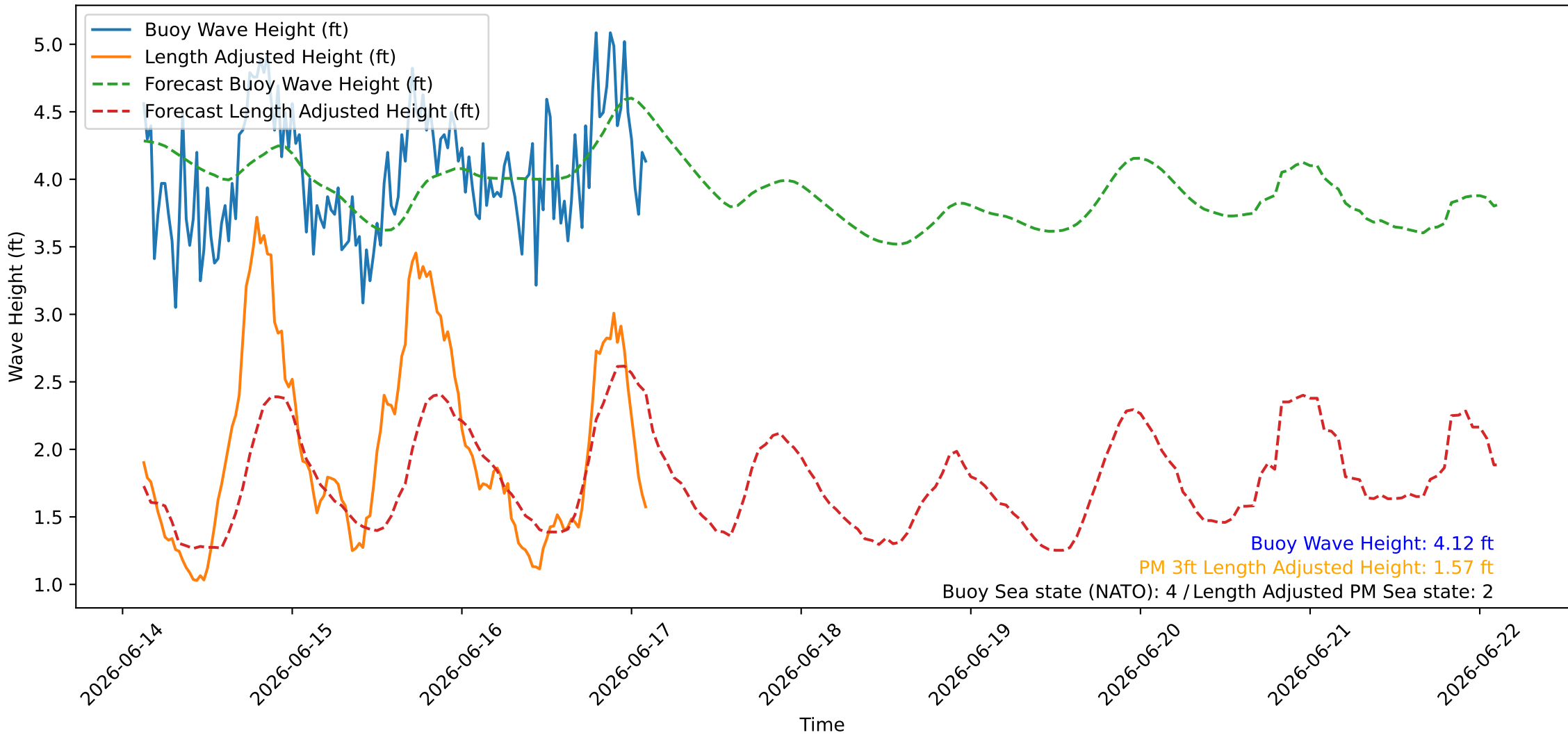
Wave Heights over Time for Green Beach at 2026-06-17 02:51:08
