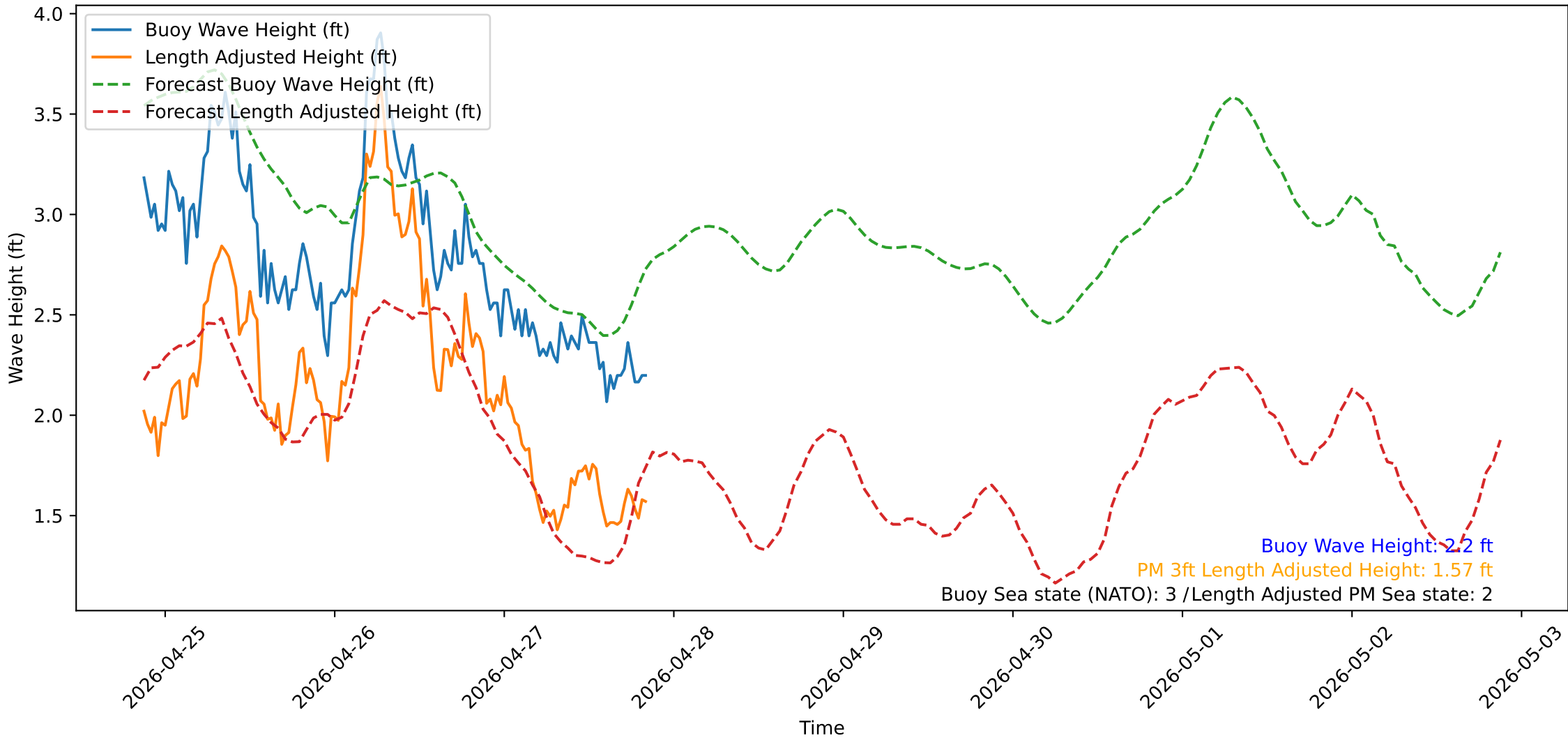
Wave Heights over Time for Oceanside Harbor at 2026-04-27 20:50:31
