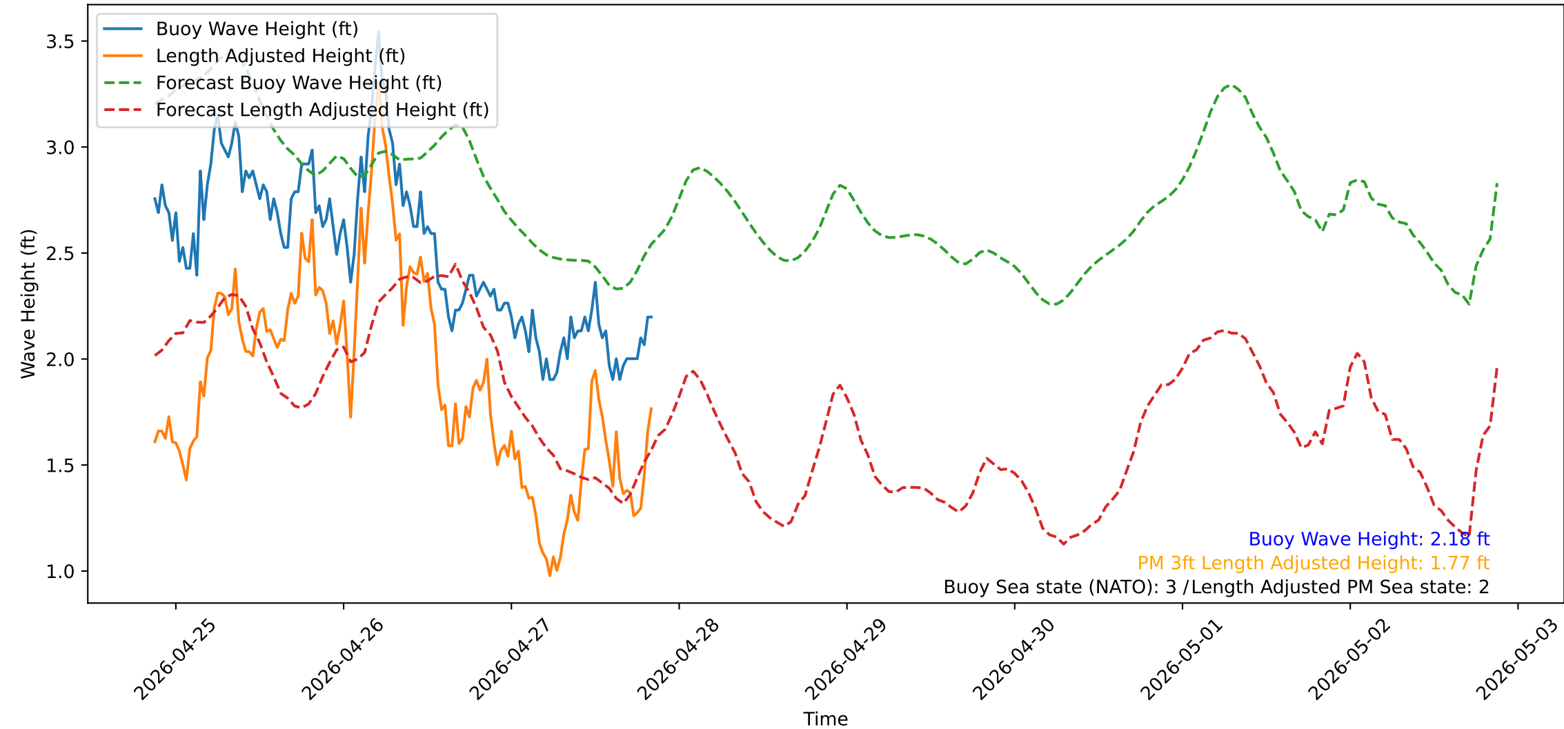
Wave Heights over Time for Red Beach at 2026-04-27 20:50:51
