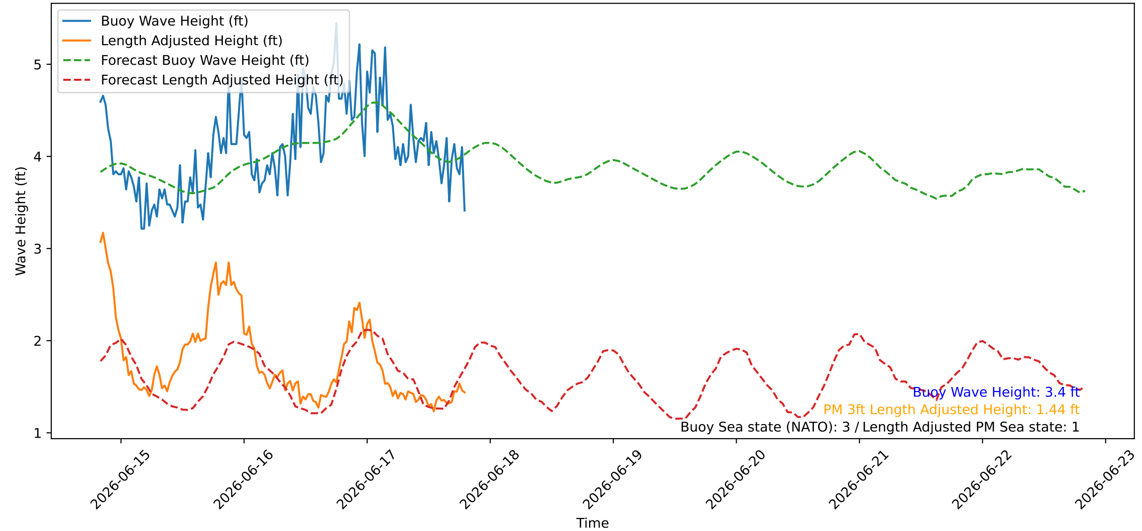
Wave Heights over Time for Oceanside Harbor at 2026-06-17 20:00:27
