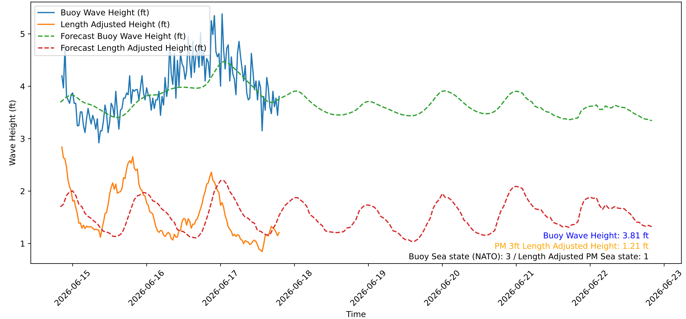
Wave Heights over Time for Red Beach at 2026-06-17 20:00:46
