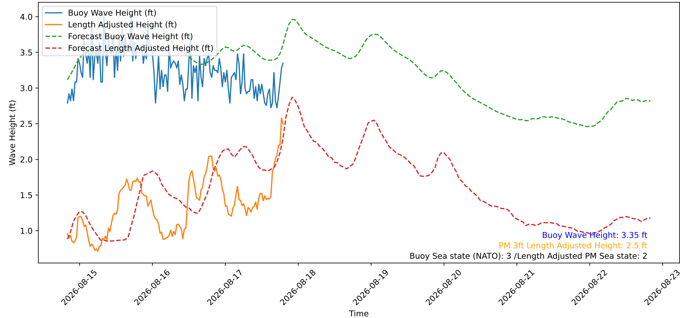
Wave Heights over Time for Red Beach at 2026-08-17 19:40:46
