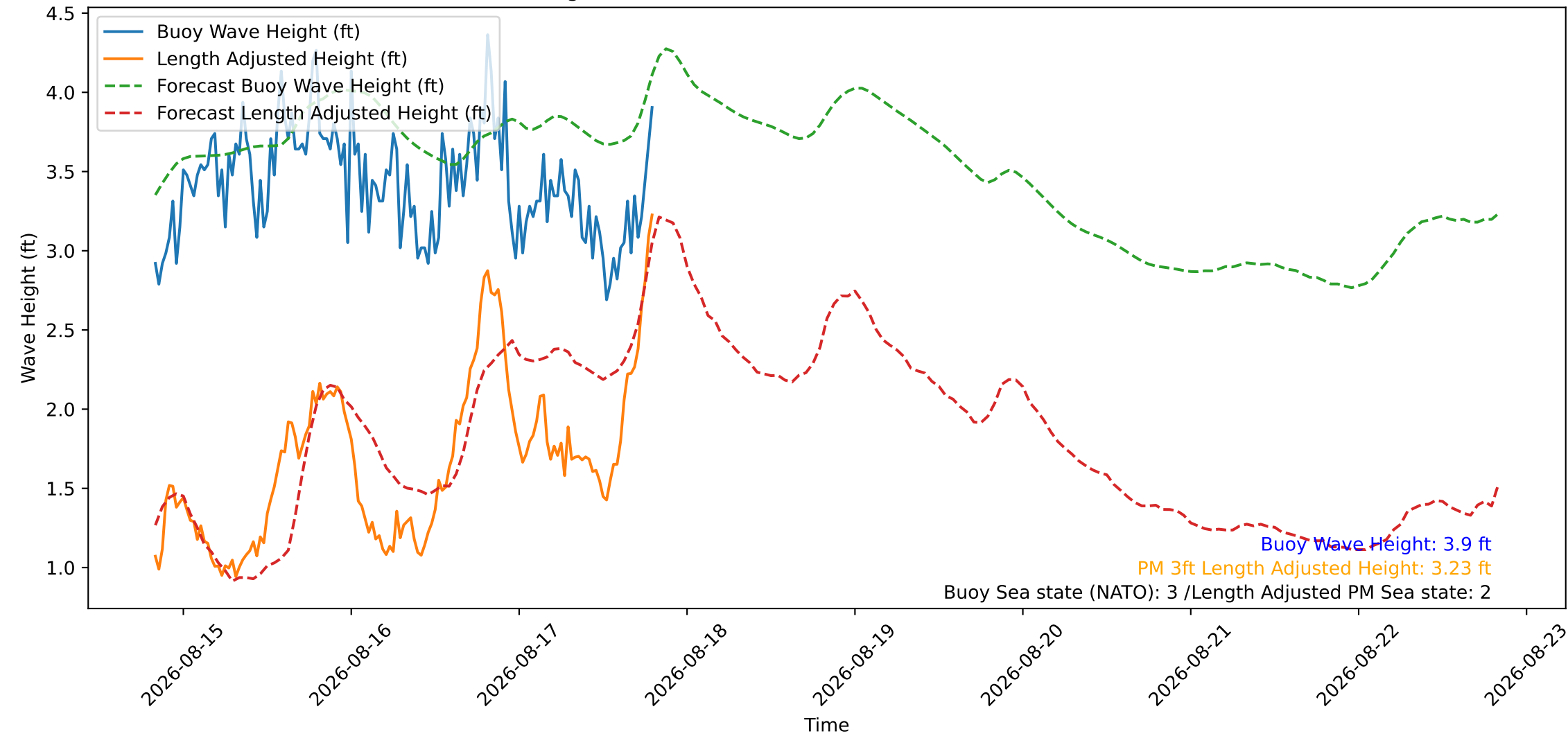
Wave Heights over Time for Green Beach at 2026-08-17 19:41:10
