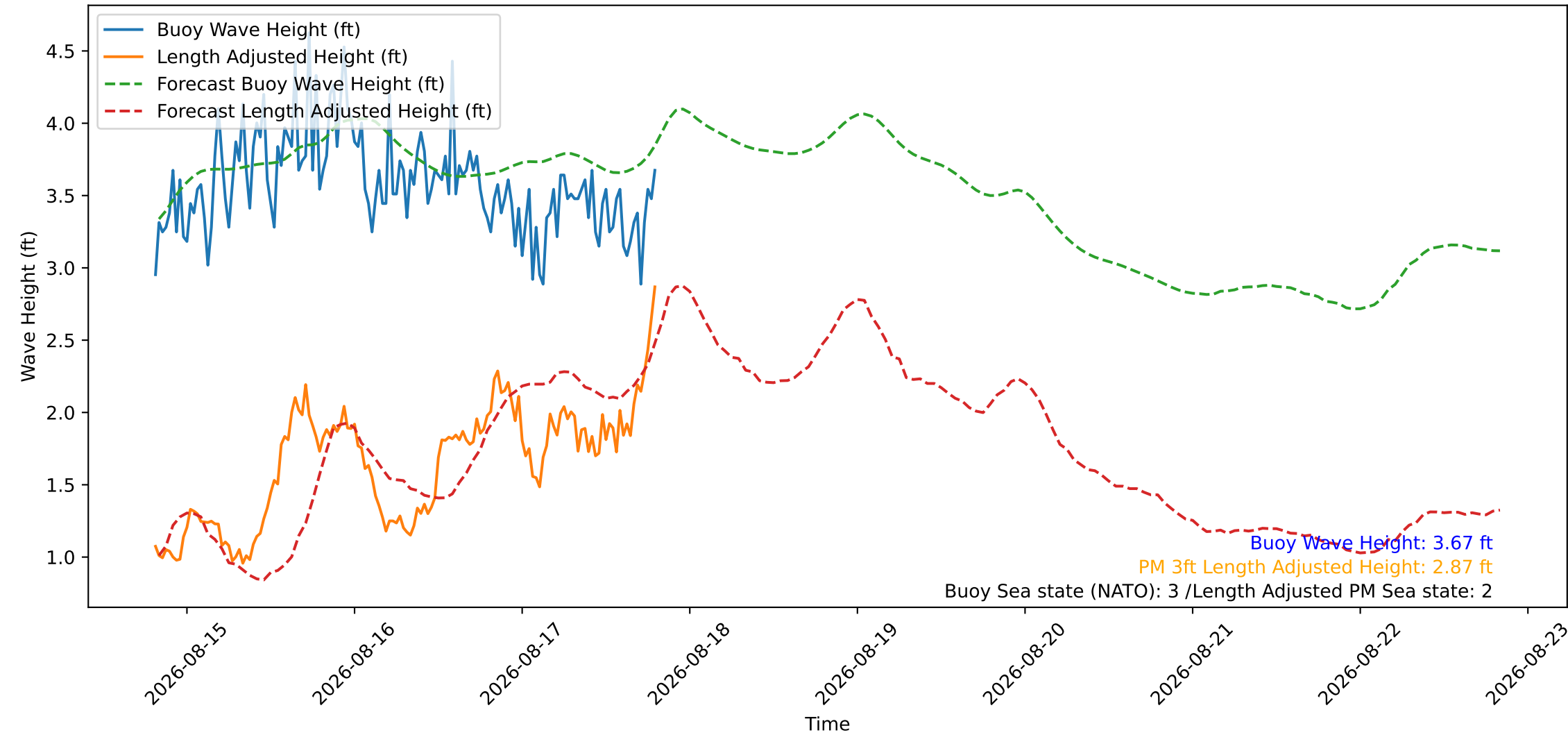
Wave Heights over Time for Oceanside Harbor at 2026-08-17 19:40:26
