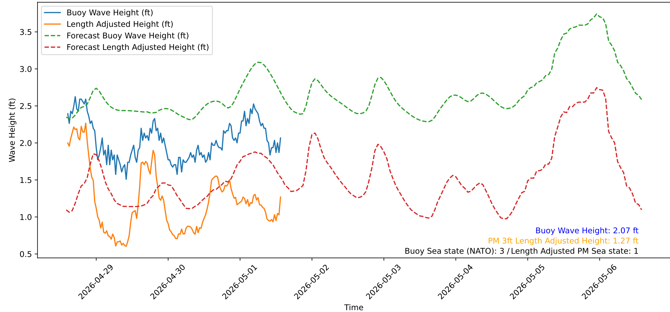
Wave Heights over Time for Red Beach at 2026-05-01 14:20:54
