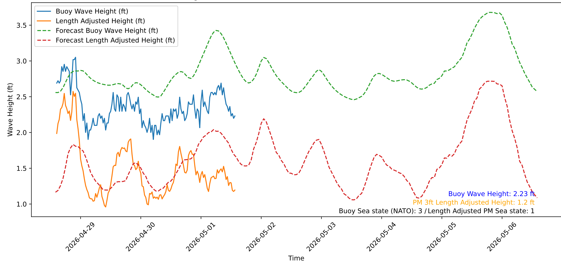
Wave Heights over Time for Oceanside Harbor at 2026-05-01 14:20:31
