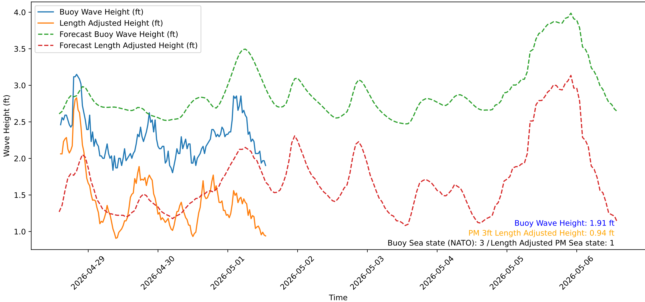
Wave Heights over Time for Green Beach at 2026-05-01 14:21:16
