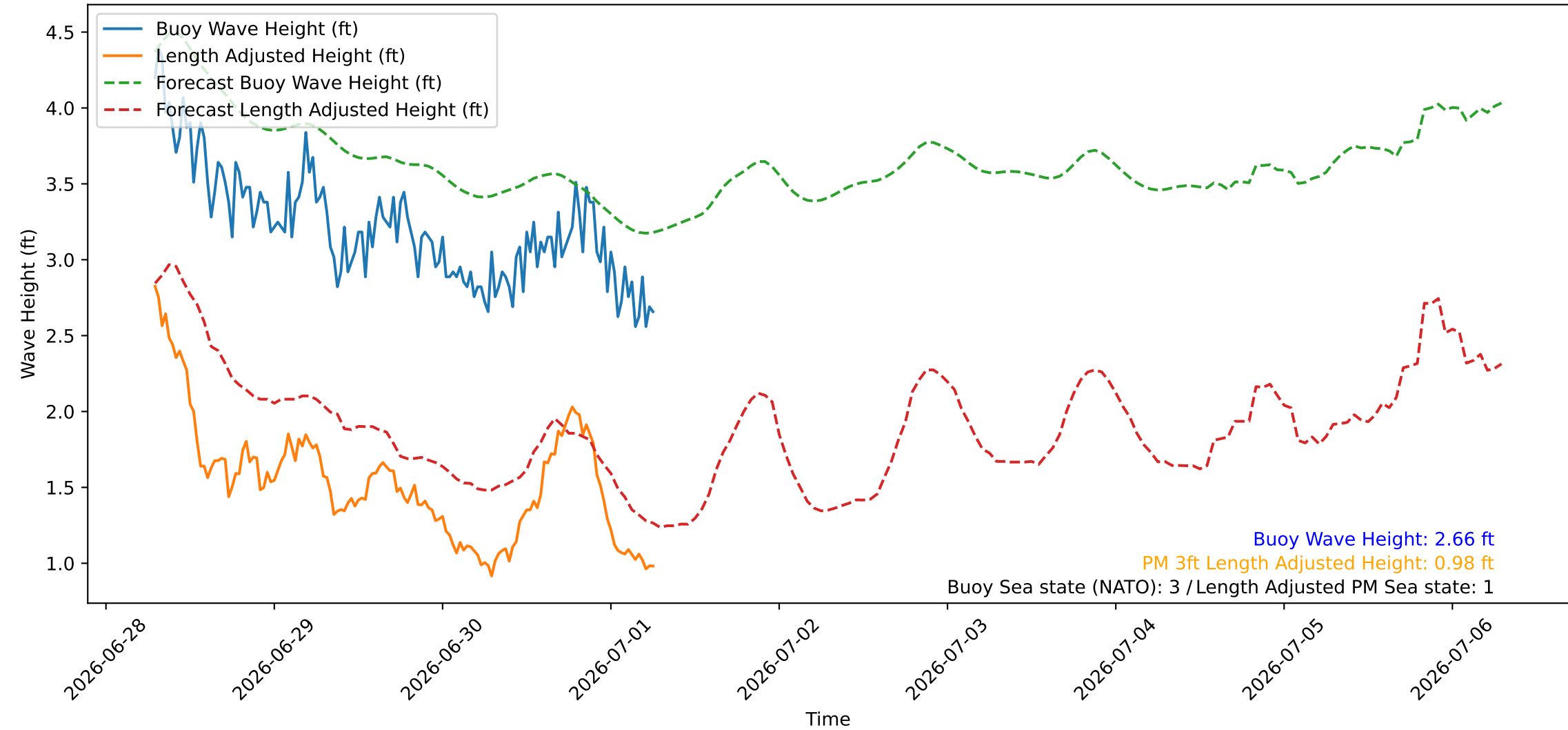
Wave Heights over Time for Green Beach at 2026-07-01 06:51:09
