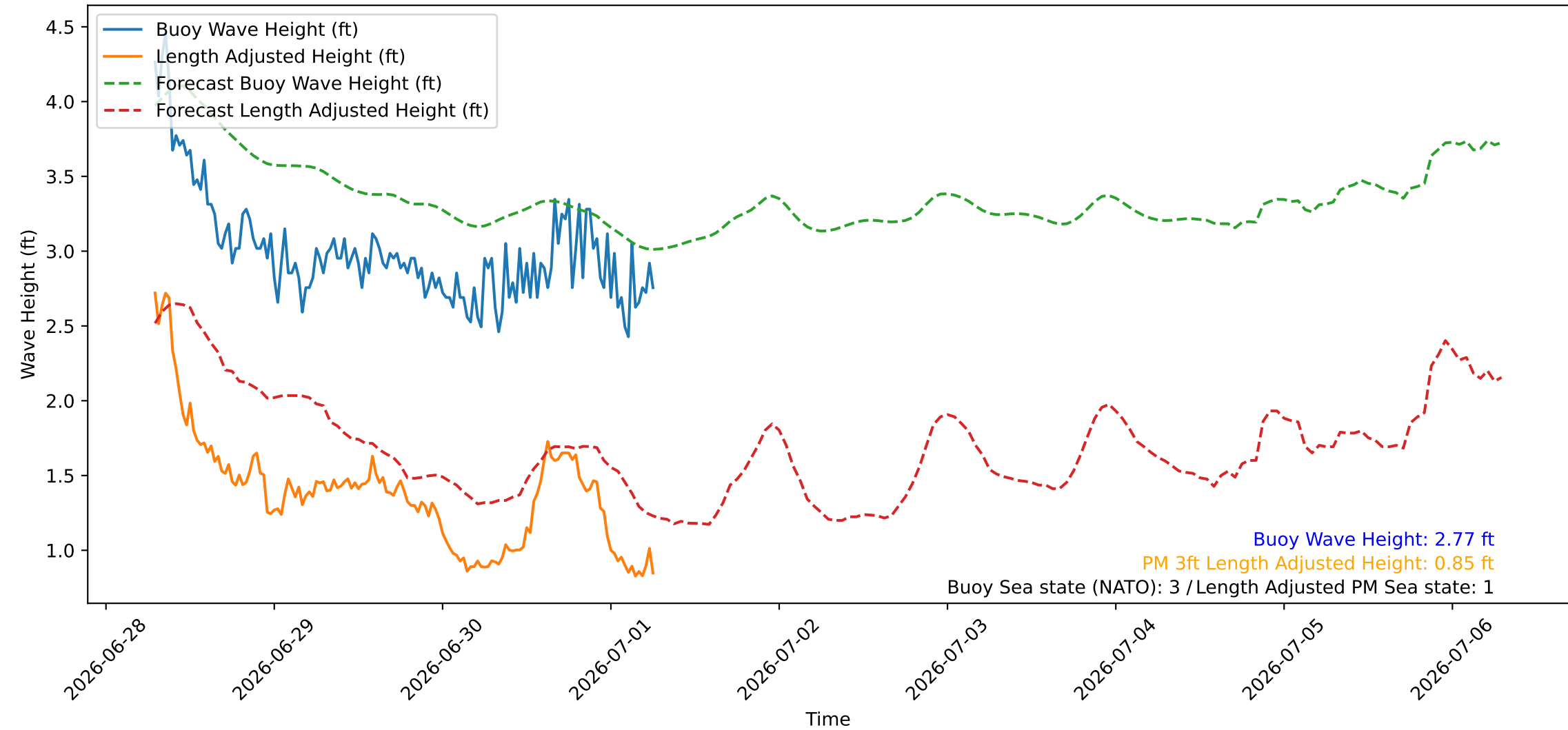
Wave Heights over Time for Red Beach at 2026-07-01 06:50:46
