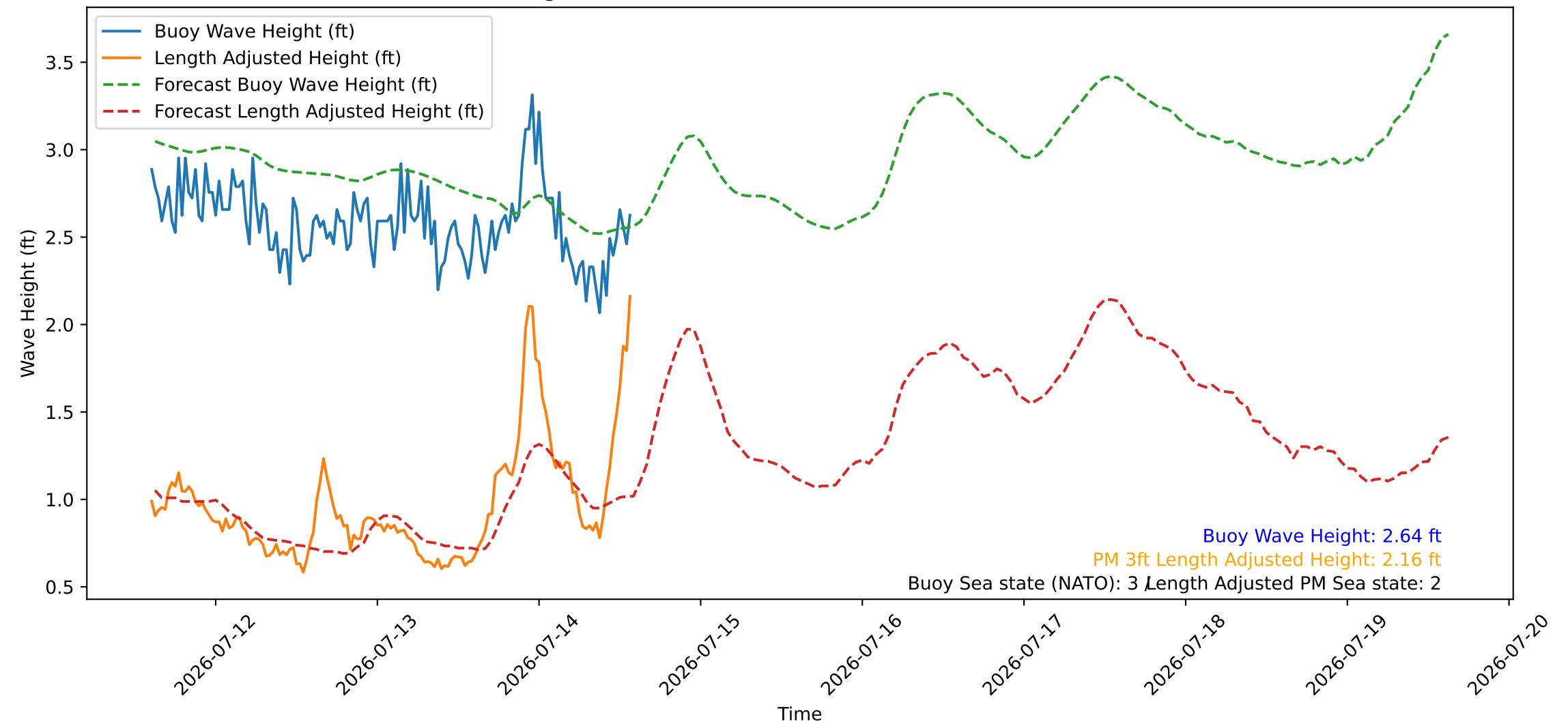
Wave Heights over Time for Green Beach at 2026-07-14 14:31:09
