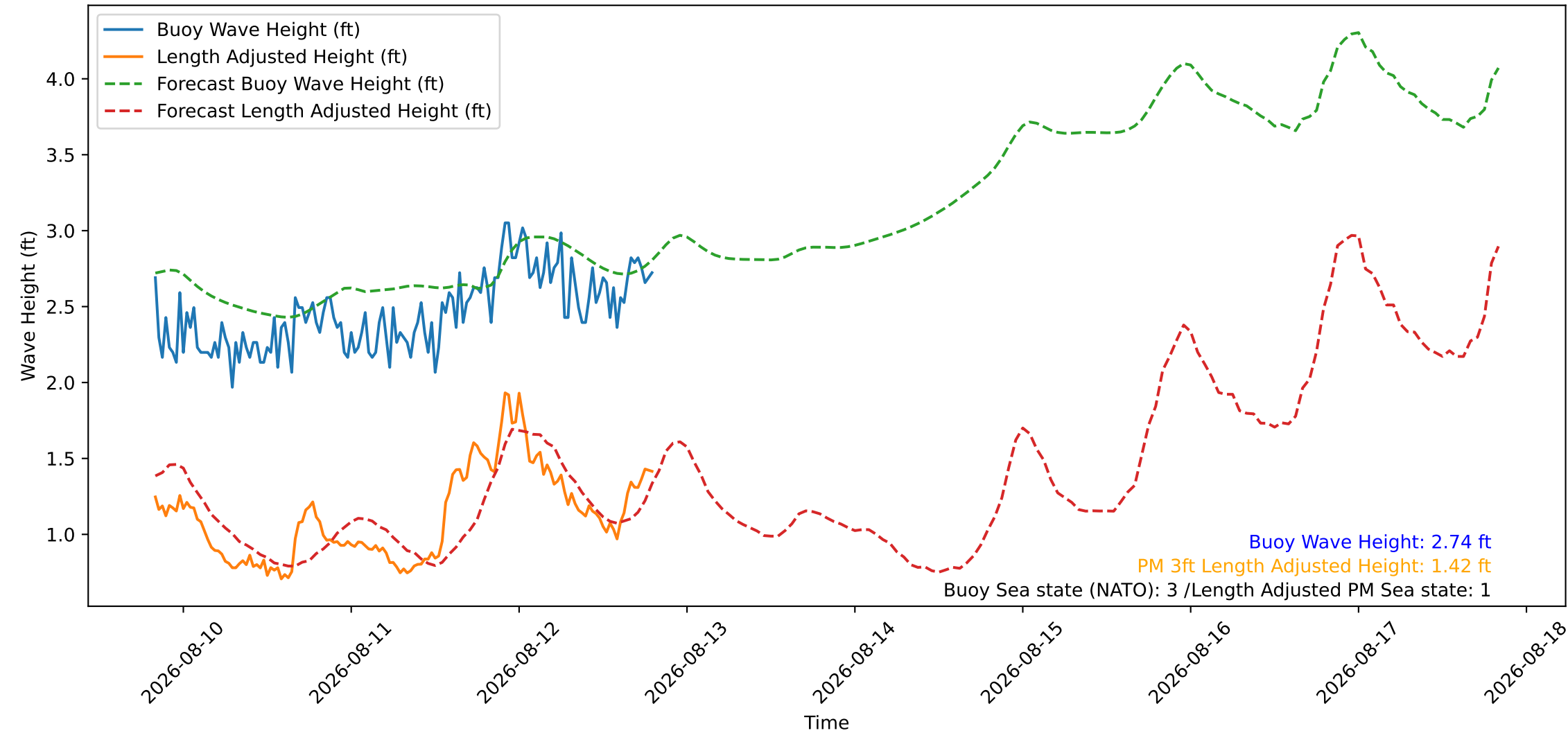
Wave Heights over Time for Oceanside Harbor at 2026-08-12 19:50:27
