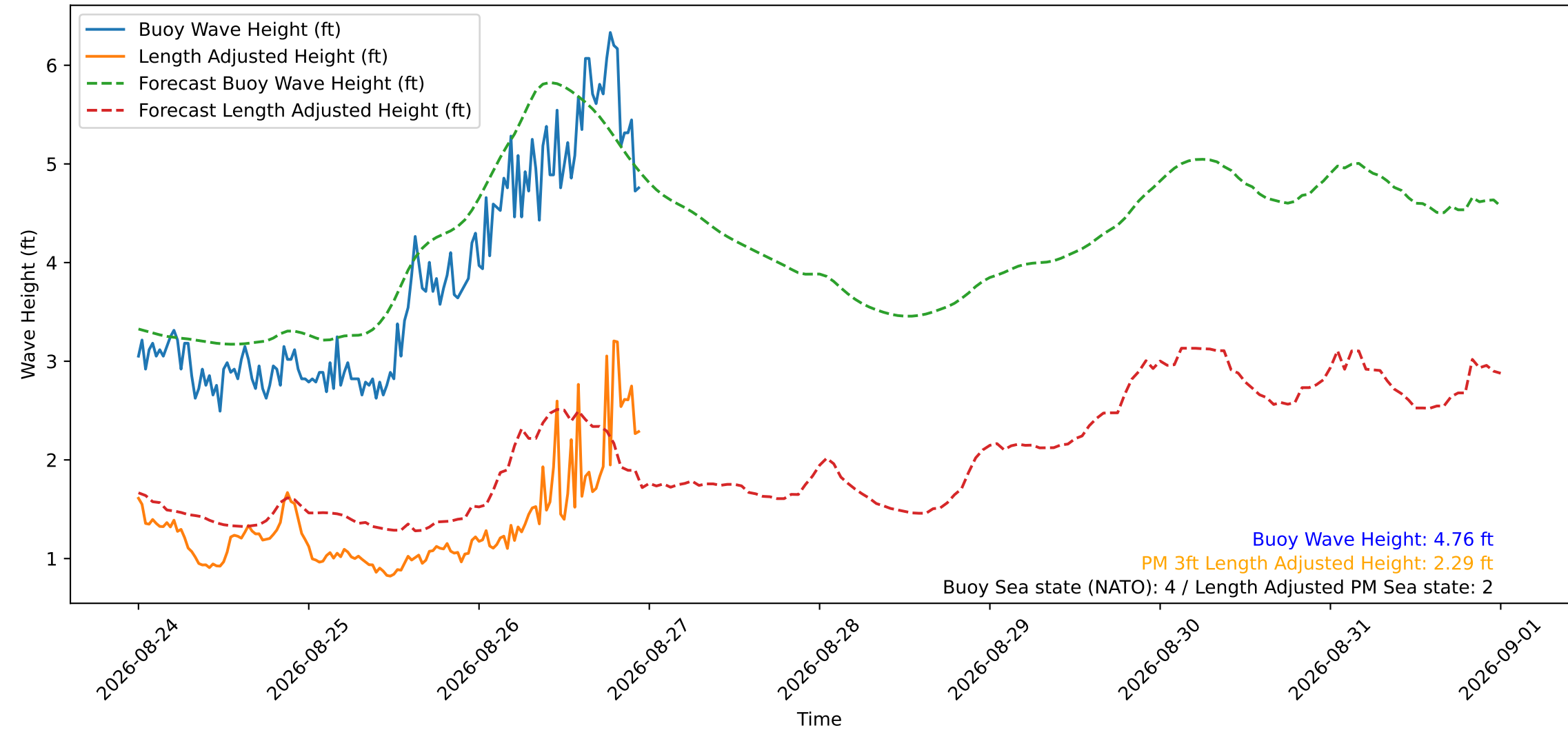
Wave Heights over Time for Green Beach at 2026-08-26 23:31:12
