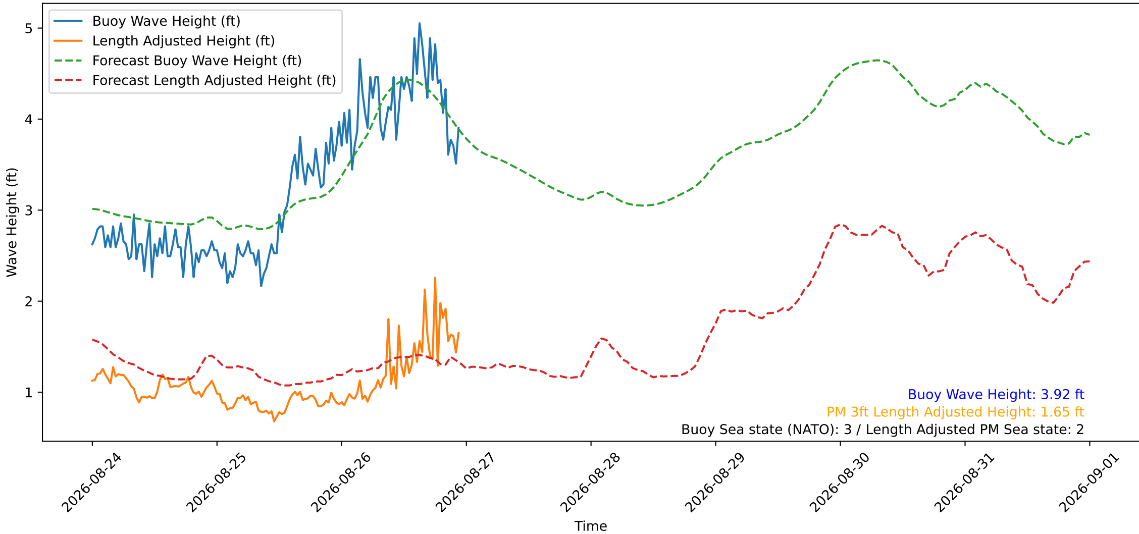
Wave Heights over Time for Red Beach at 2026-08-26 23:30:50
