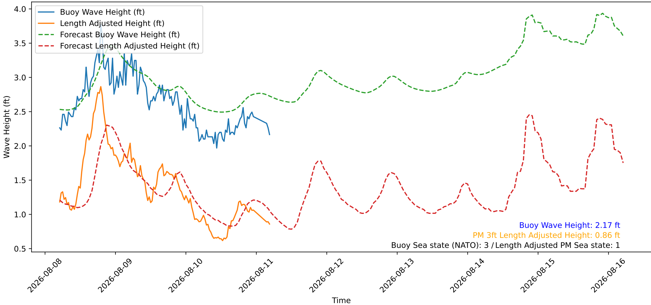
Wave Heights over Time for Green Beach at 2026-08-11 05:11:09
