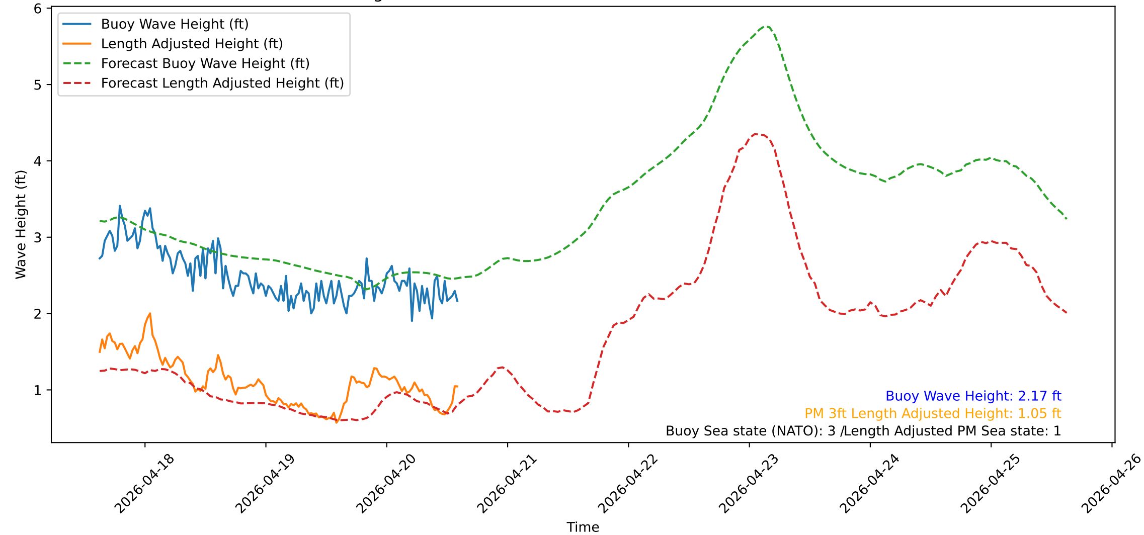
Wave Heights over Time for Oceanside Harbor at 2026-04-20 15:00:31
