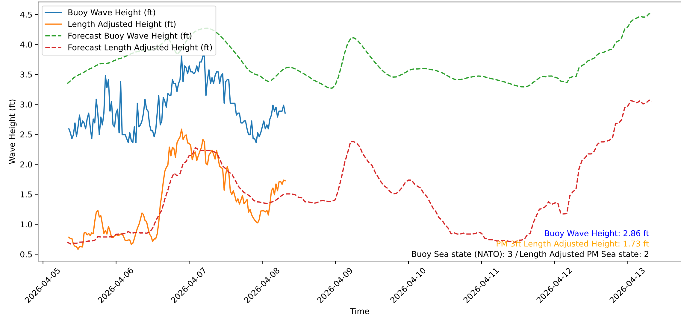
Wave Heights over Time for Green Beach at 2026-04-08 08:21:10
