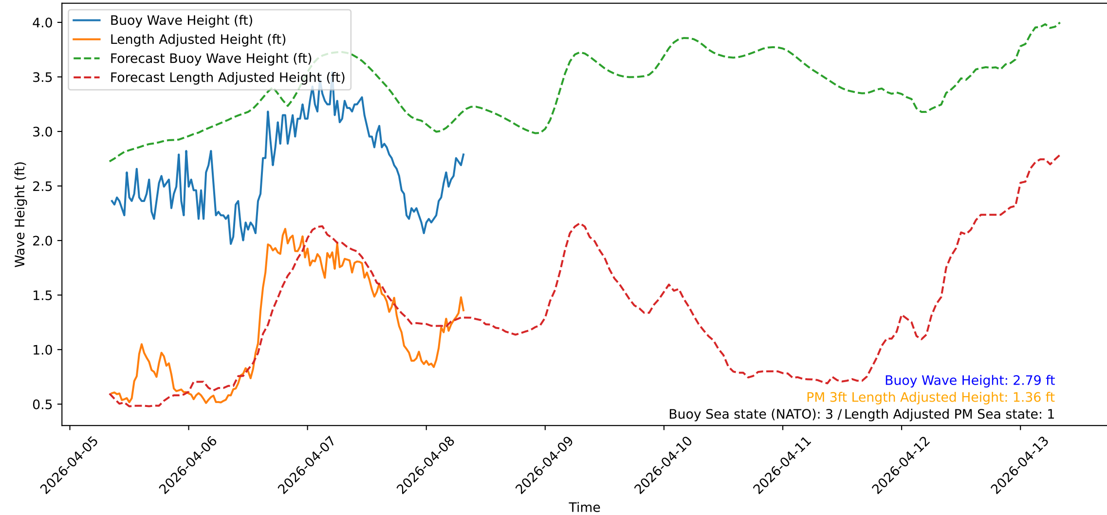
Wave Heights over Time for Red Beach at 2026-04-08 08:20:48
