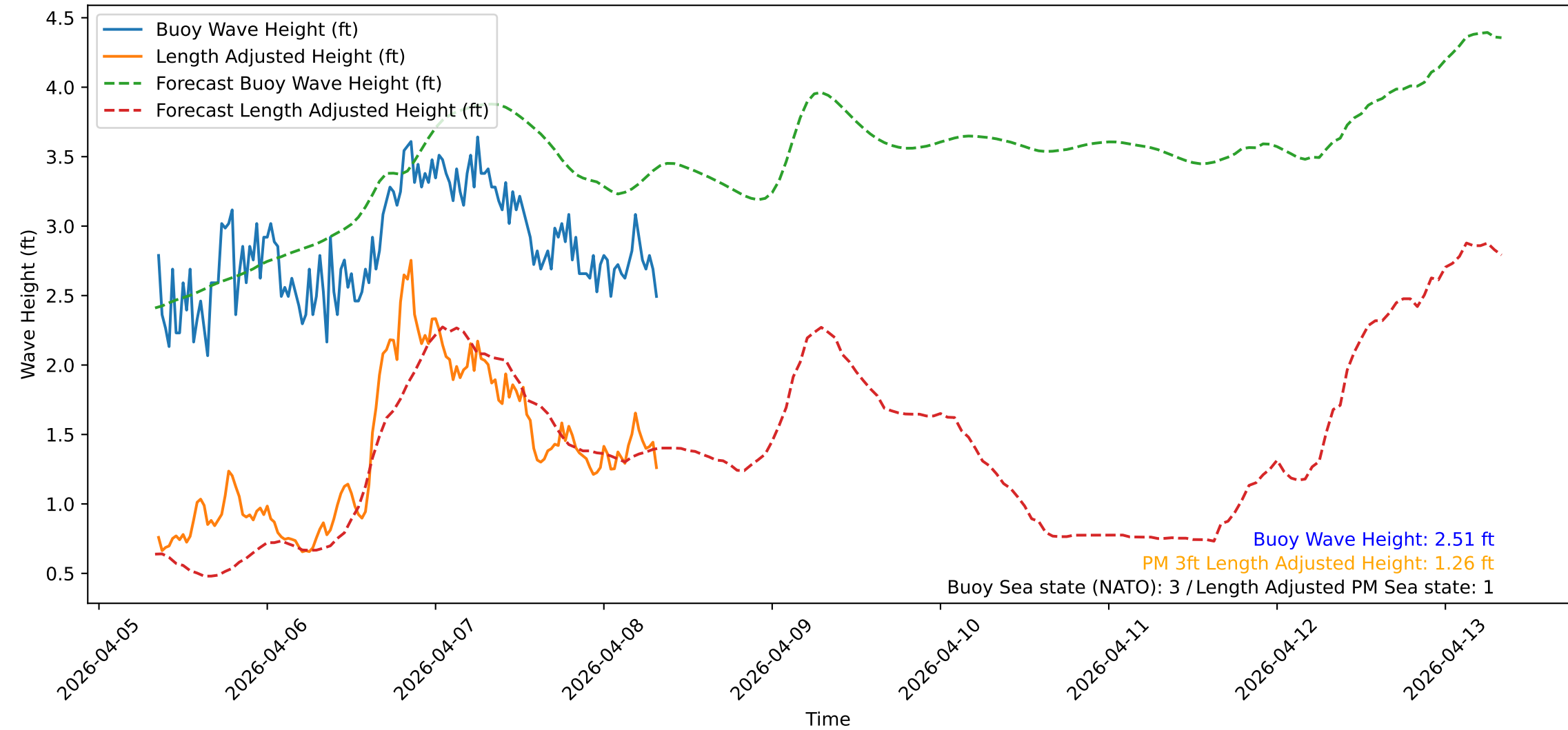
Wave Heights over Time for Oceanside Harbor at 2026-04-08 08:20:32
