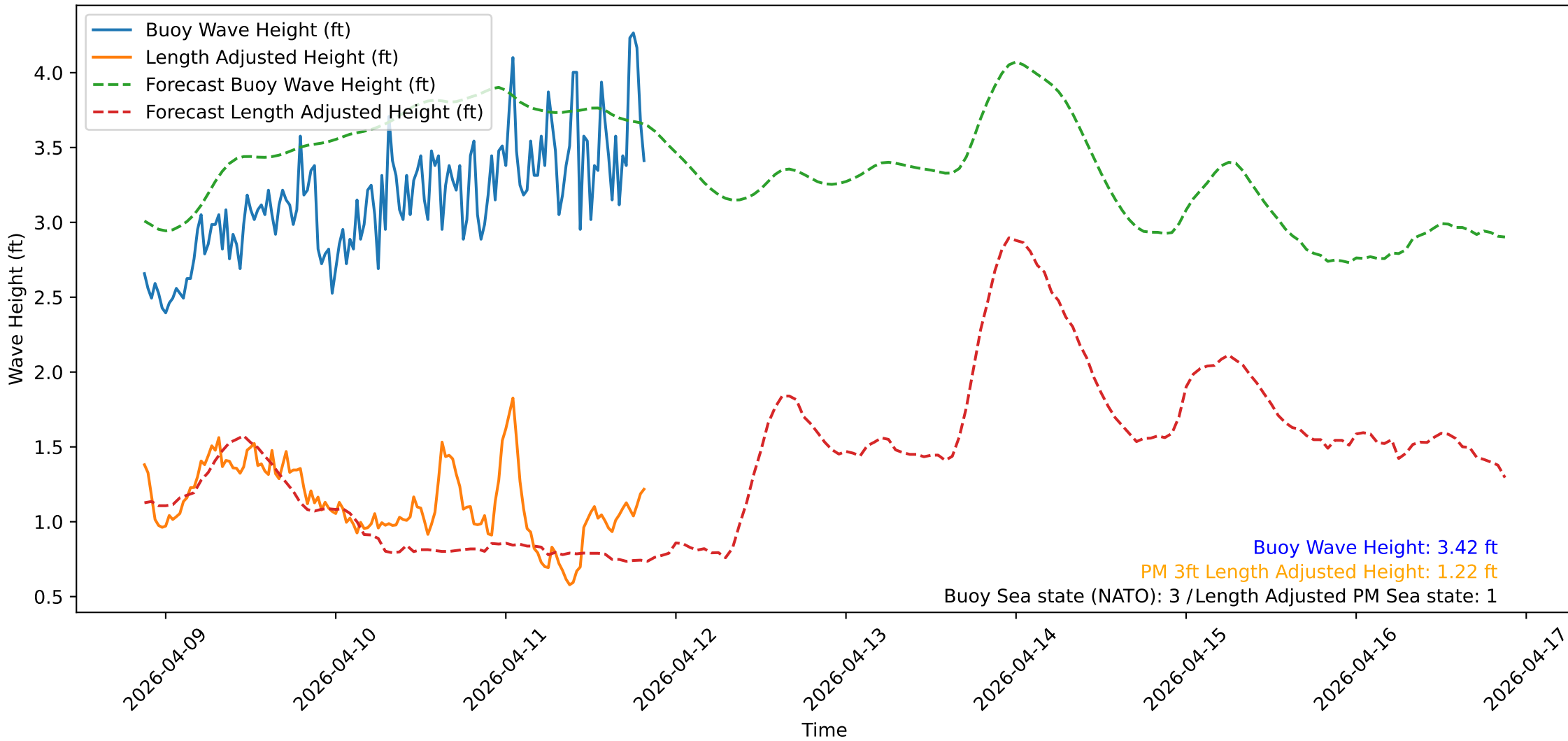
Wave Heights over Time for Red Beach at 2026-04-11 20:50:52
