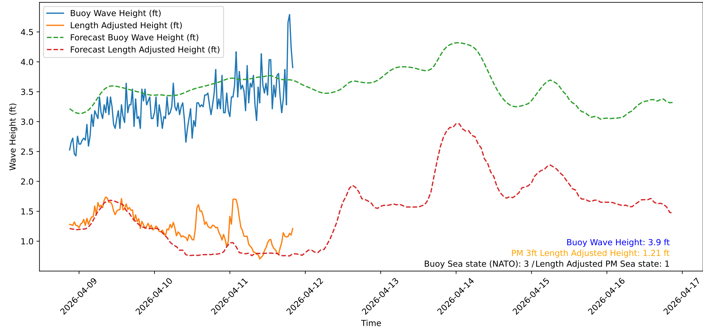
Wave Heights over Time for Oceanside Harbor at 2026-04-11 20:50:31
