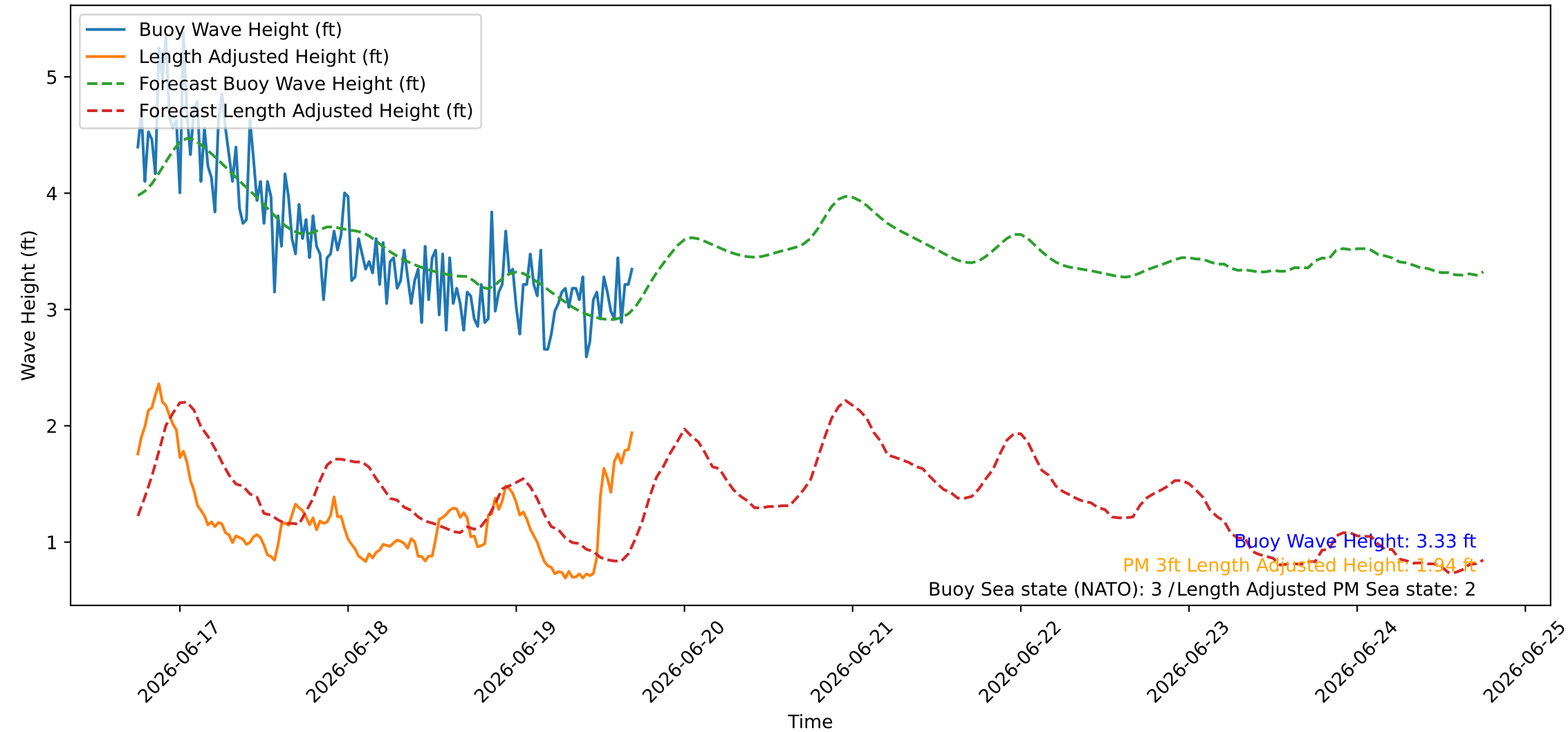
Wave Heights over Time for Red Beach at 2026-06-19 17:30:44
