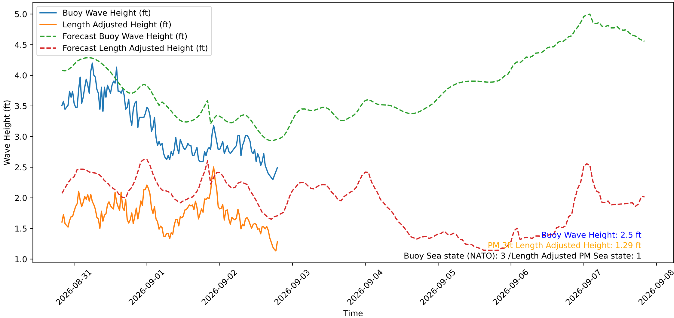
Wave Heights over Time for Red Beach at 2026-09-02 19:40:50
