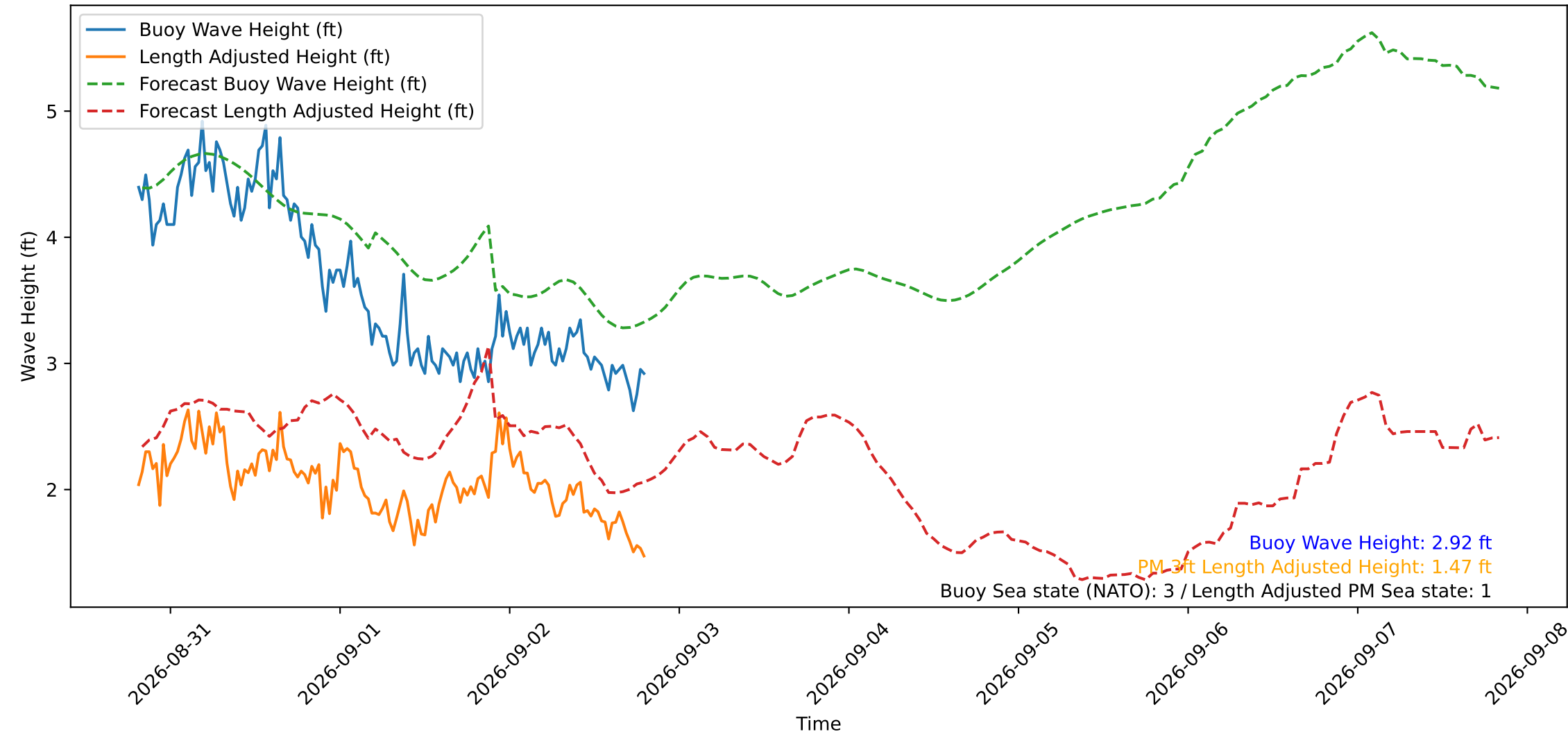
Wave Heights over Time for Oceanside Harbor at 2026-09-02 19:40:30
