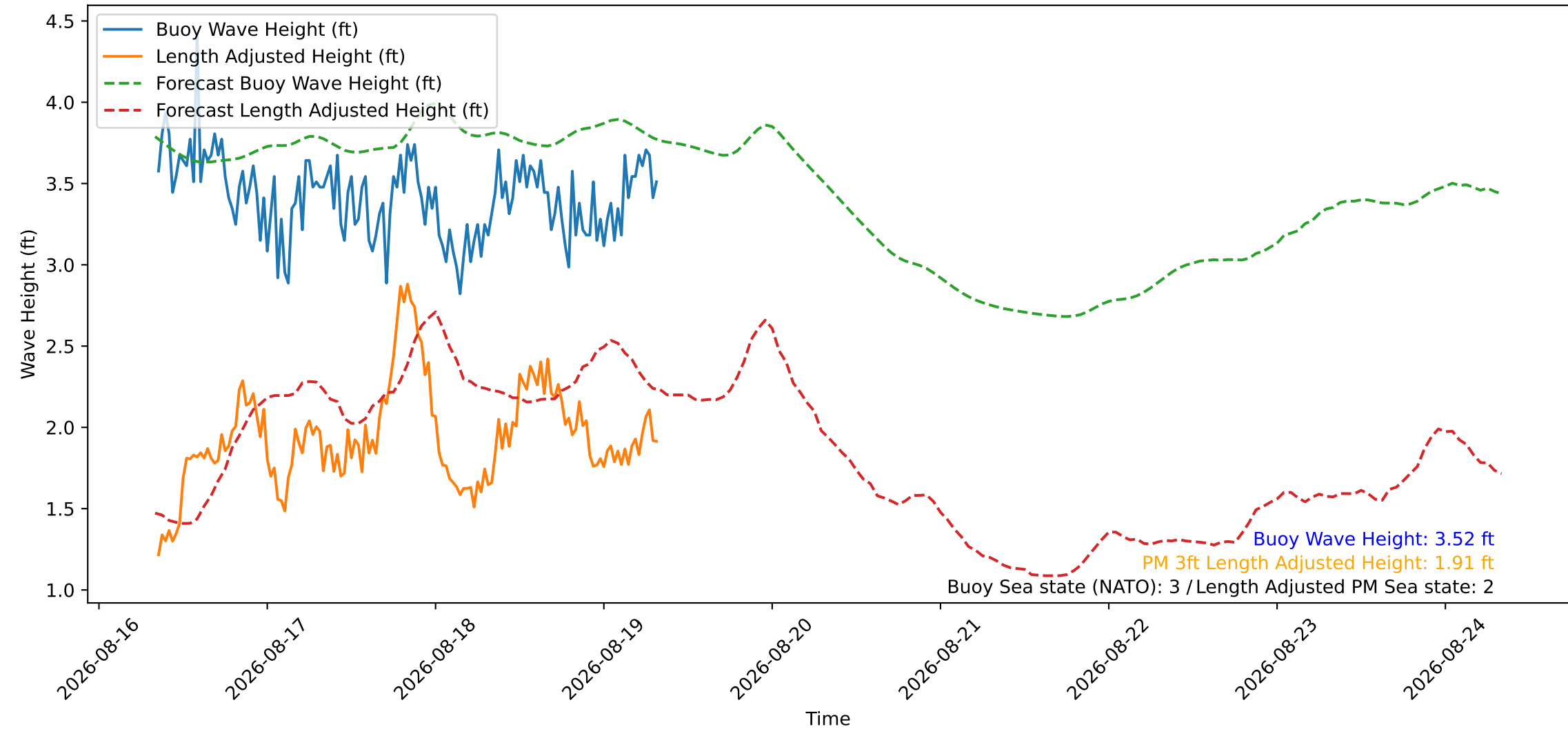
Wave Heights over Time for Oceanside Harbor at 2026-08-19 08:20:27
