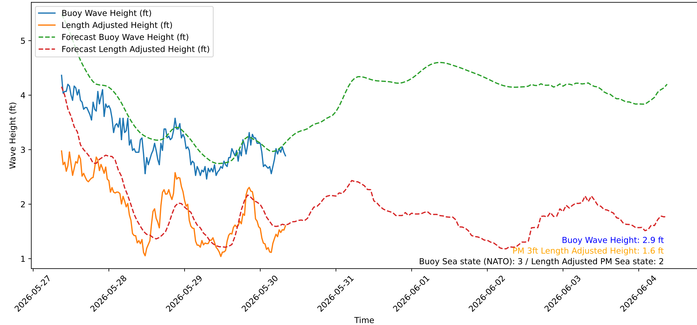
Wave Heights over Time for Green Beach at 2026-05-30 09:01:05
