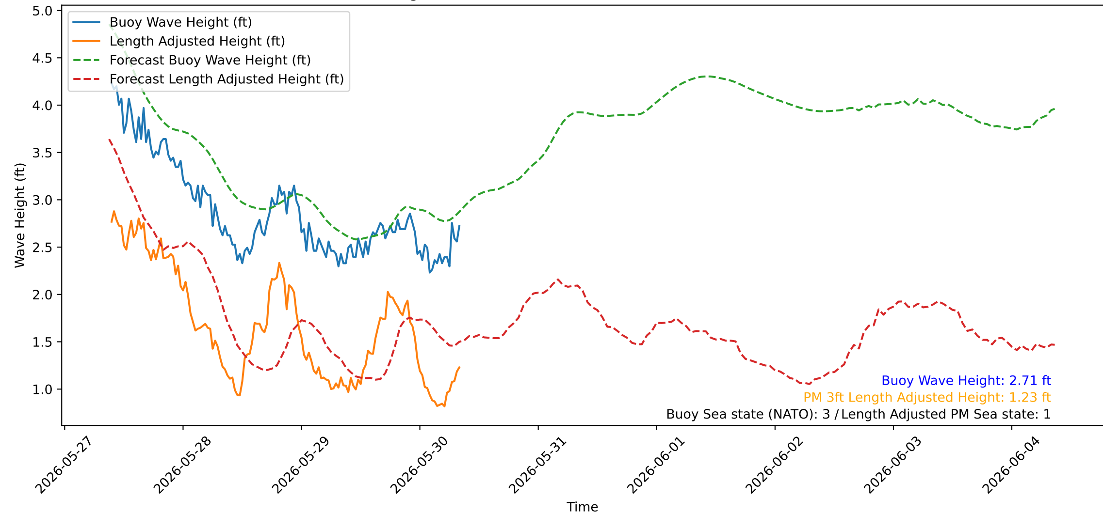
Wave Heights over Time for Red Beach at 2026-05-30 09:00:43
