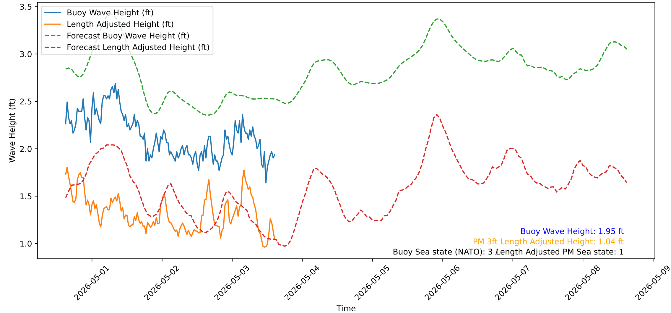
Wave Heights over Time for Oceanside Harbor at 2026-05-03 15:10:31
