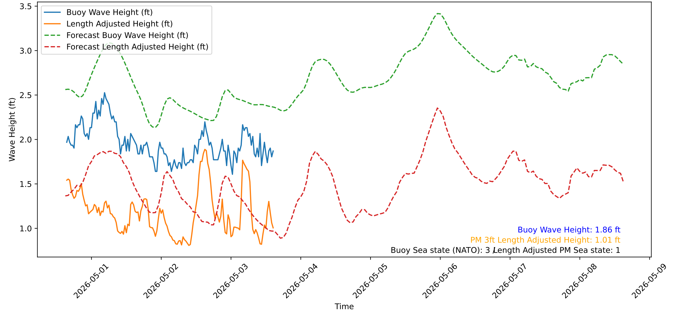
Wave Heights over Time for Red Beach at 2026-05-03 15:10:50
