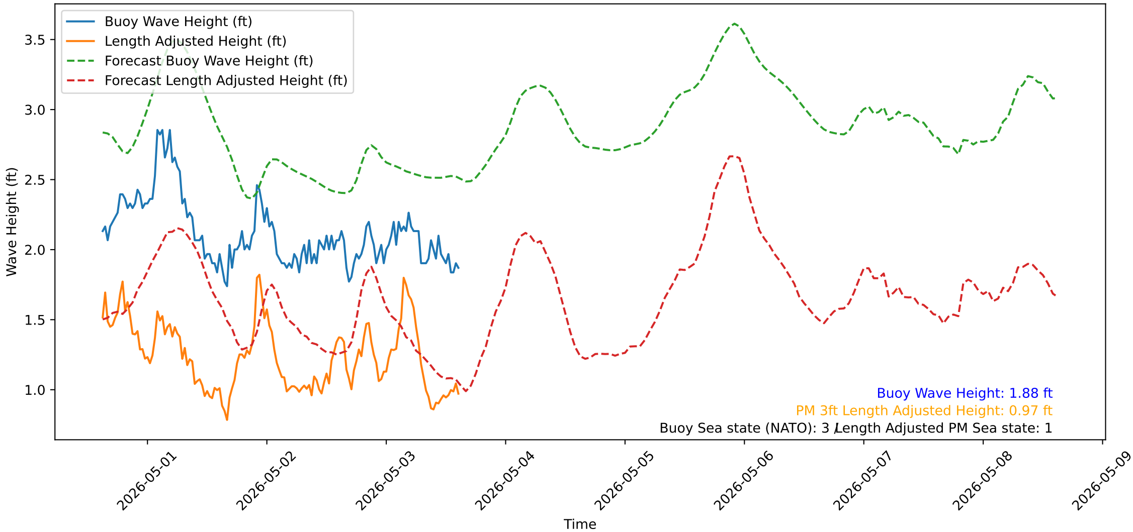
Wave Heights over Time for Green Beach at 2026-05-03 15:11:12
