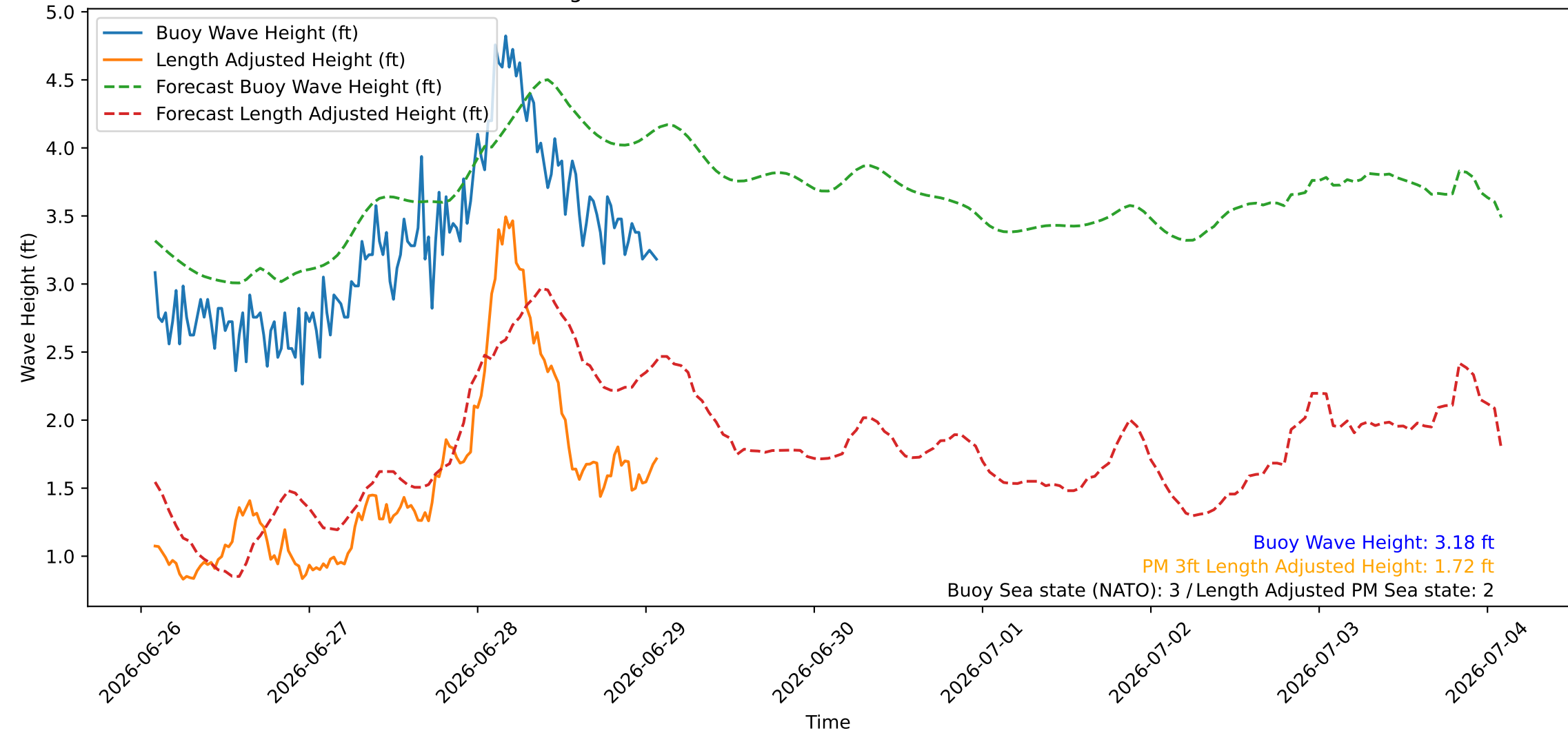
Wave Heights over Time for Green Beach at 2026-06-29 02:11:07
