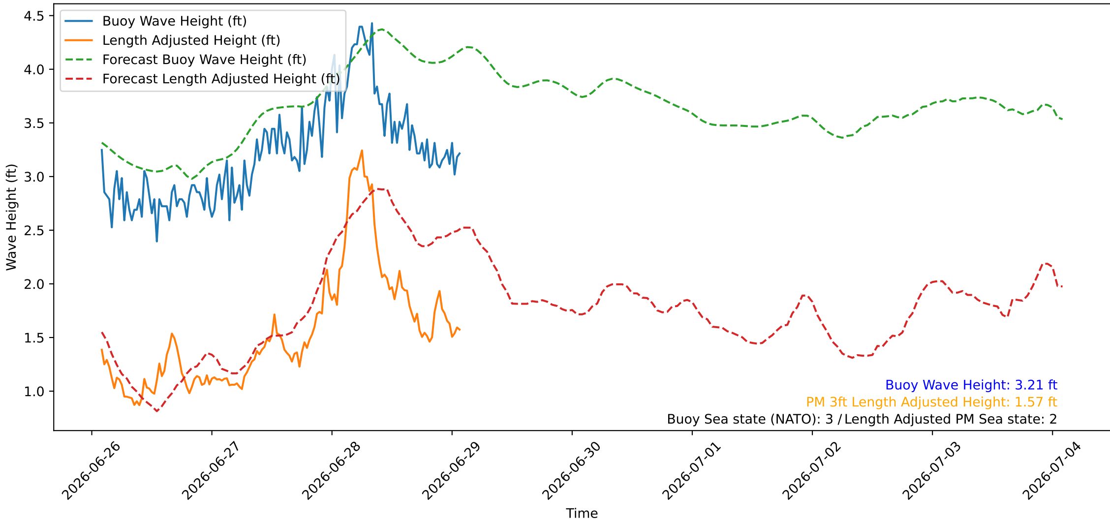
Wave Heights over Time for Oceanside Harbor at 2026-06-29 02:10:26
