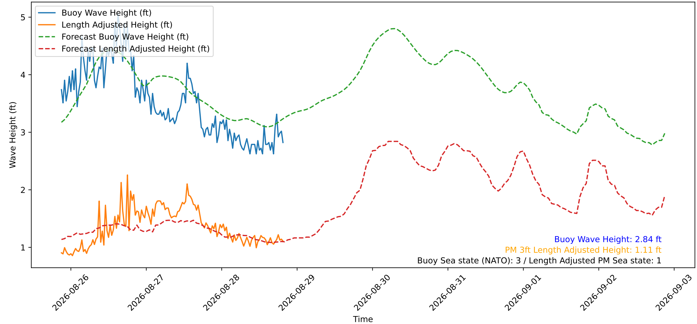
Wave Heights over Time for Red Beach at 2026-08-28 20:30:50
