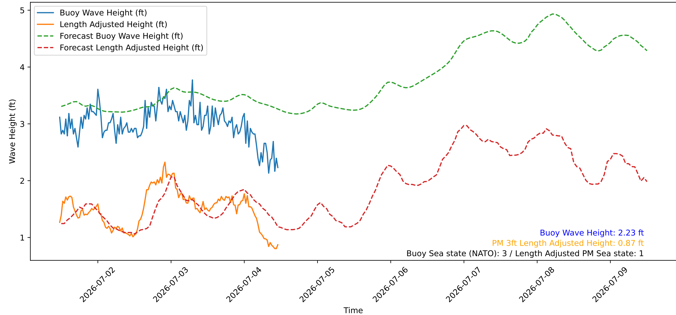
Wave Heights over Time for Oceanside Harbor at 2026-07-04 11:30:26
