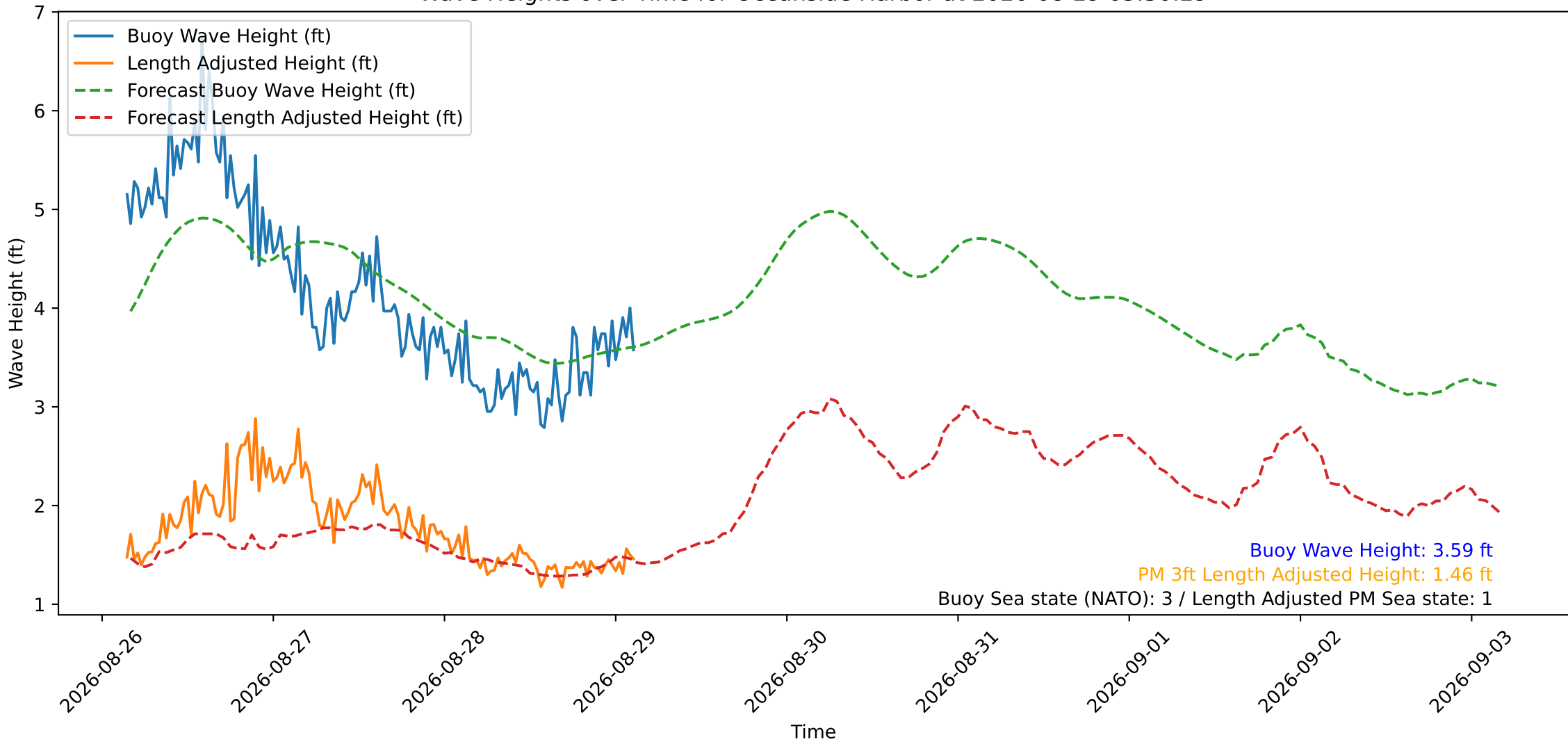
Wave Heights over Time for Oceanside Harbor at 2026-08-29 03:30:29
