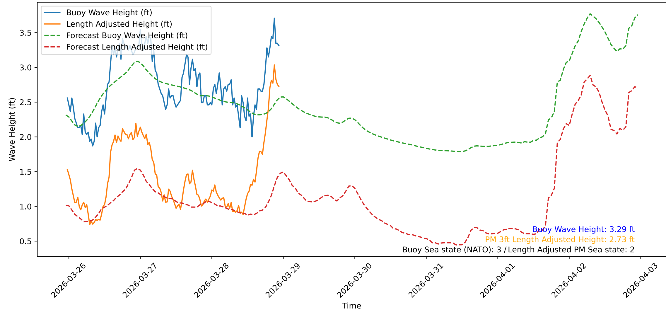
Wave Heights over Time for Green Beach at 2026-03-28 23:21:10
