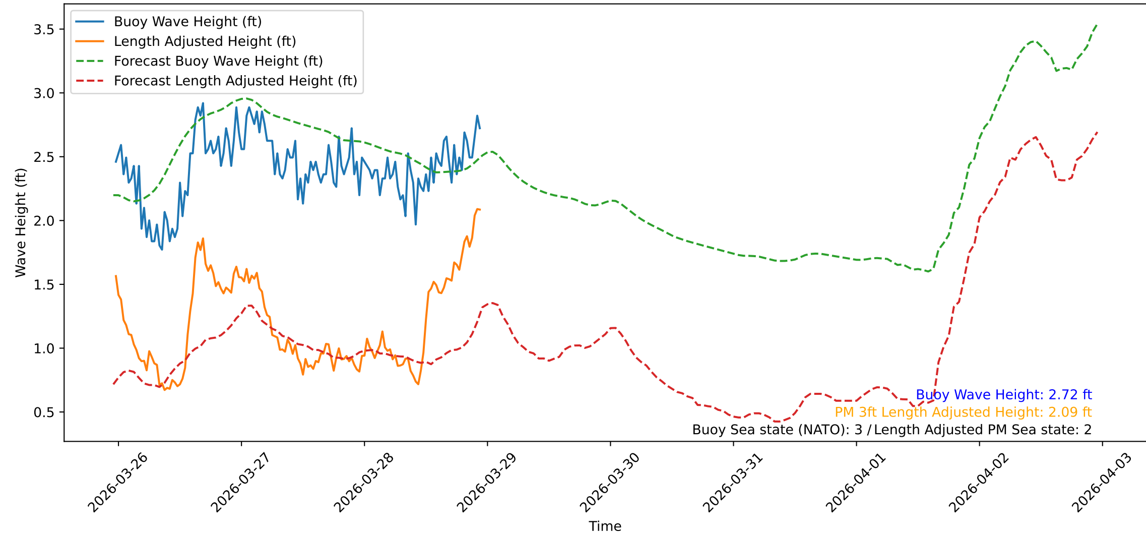
Wave Heights over Time for Oceanside Harbor at 2026-03-28 23:20:31
