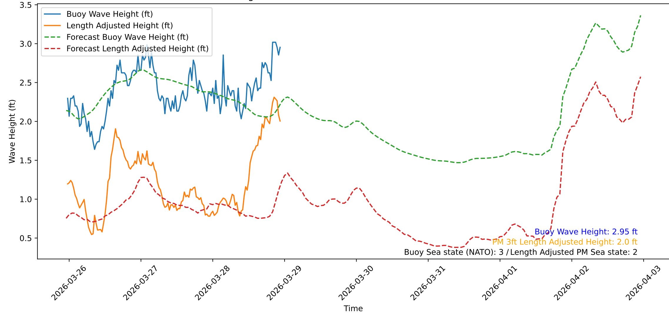
Wave Heights over Time for Red Beach at 2026-03-28 23:20:48
