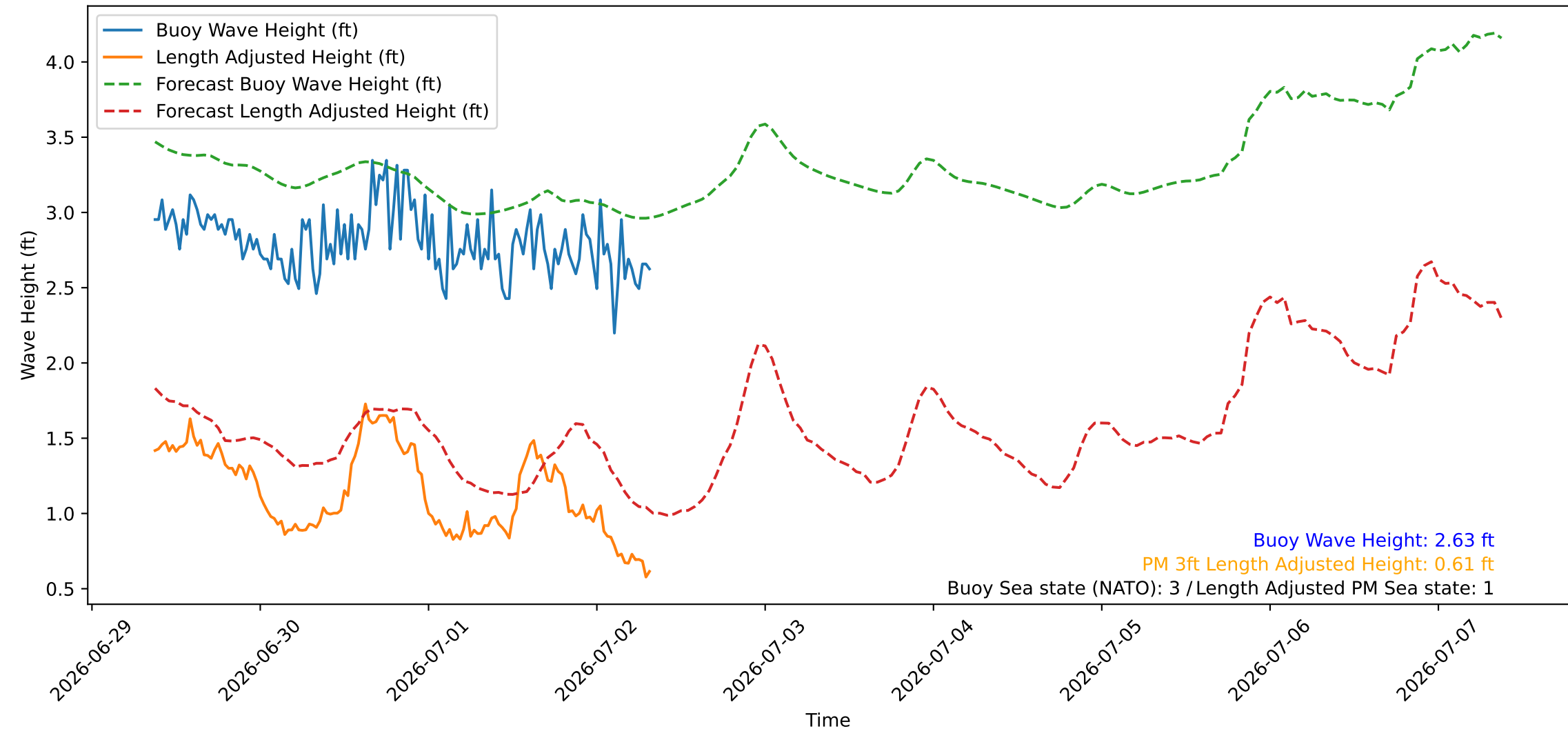
Wave Heights over Time for Red Beach at 2026-07-02 08:30:46
