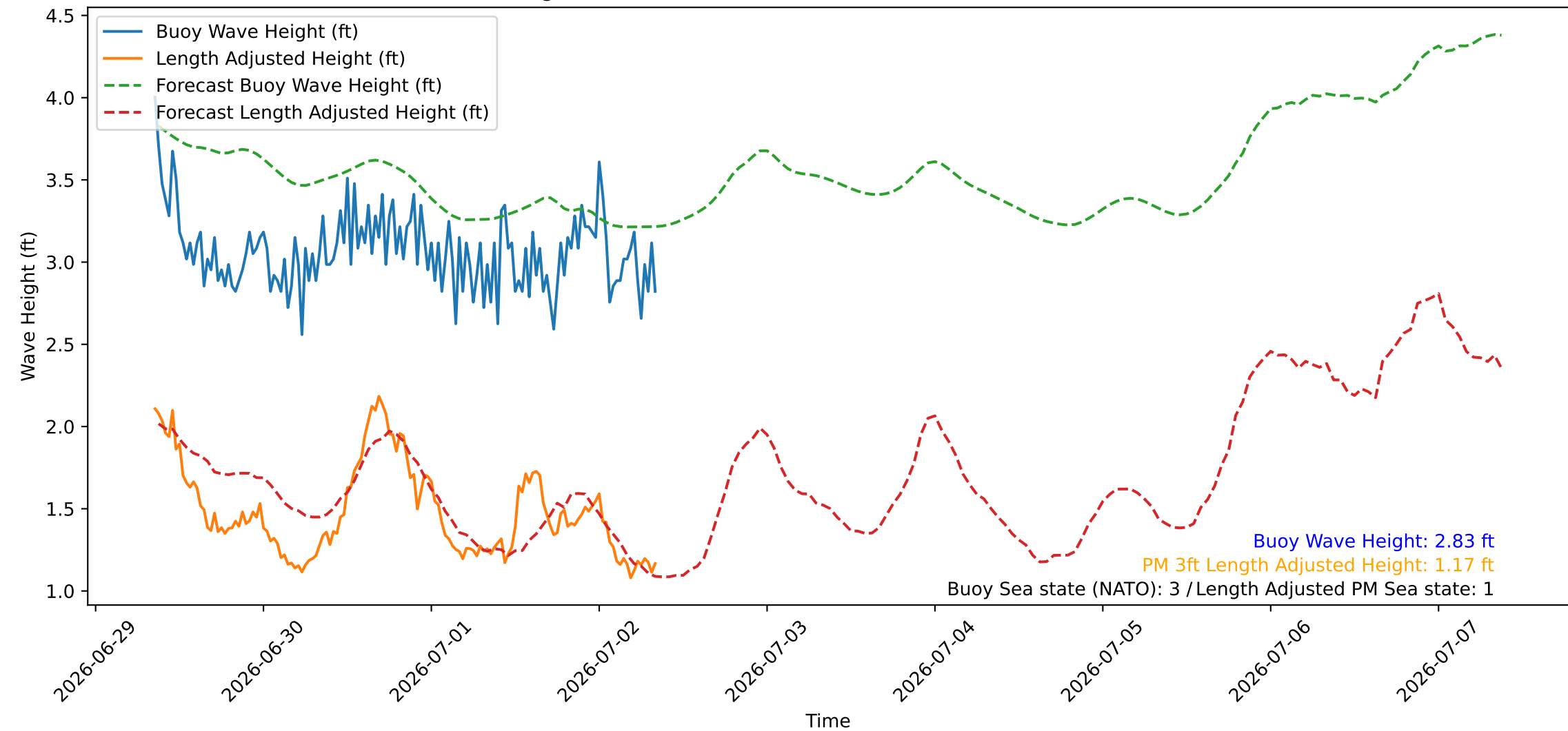
Wave Heights over Time for Oceanside Harbor at 2026-07-02 08:30:26
