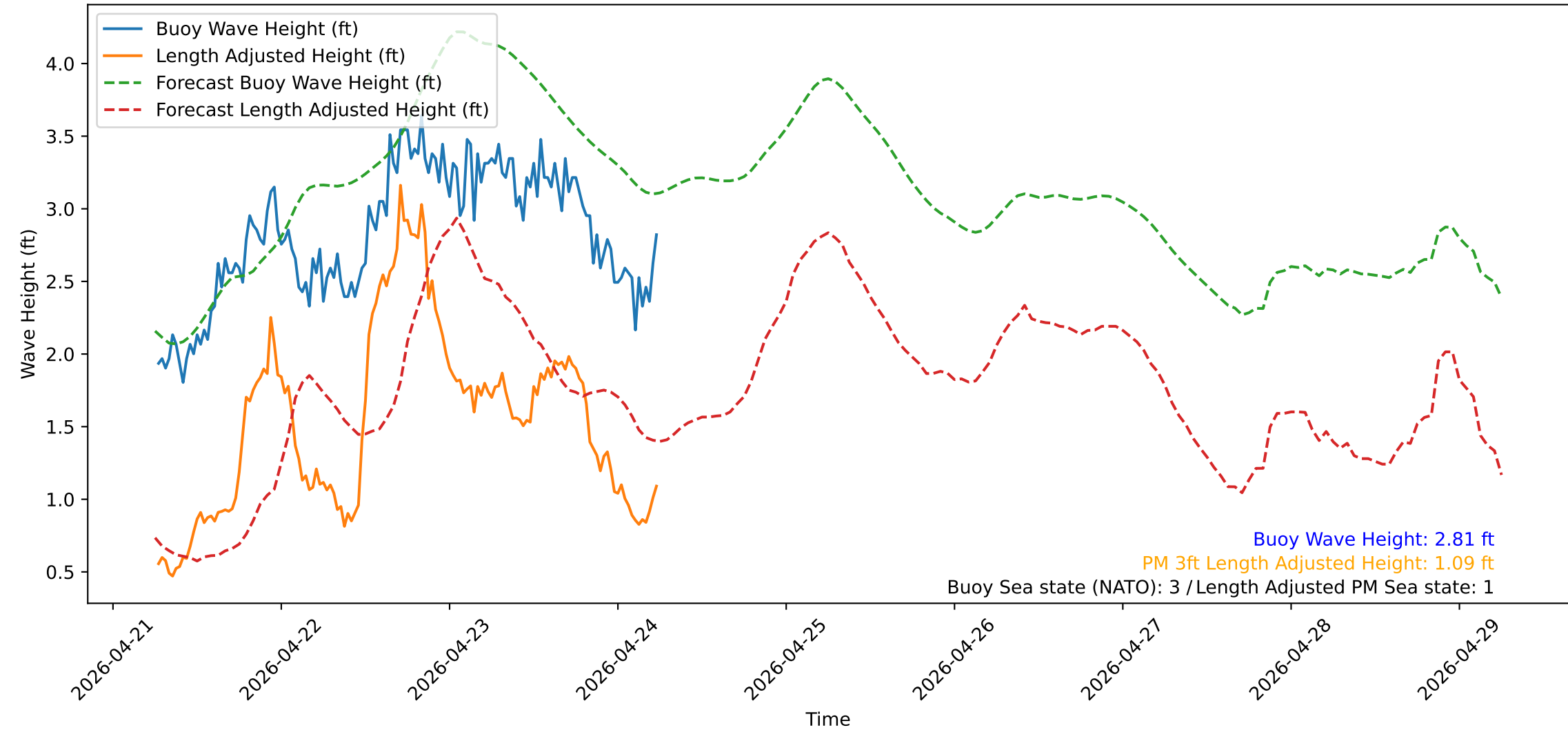
Wave Heights over Time for Red Beach at 2026-04-24 06:10:50
