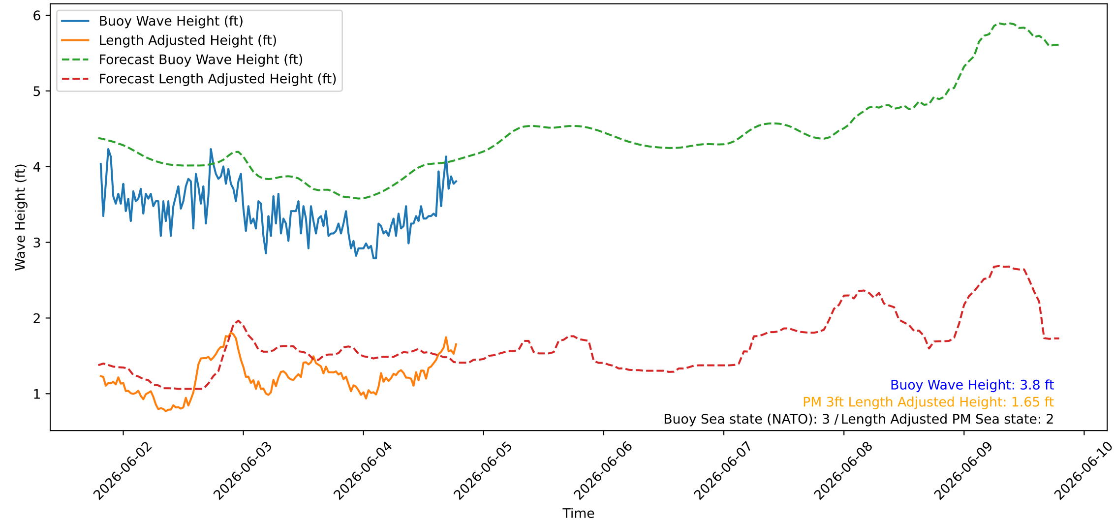
Wave Heights over Time for Green Beach at 2026-06-04 19:21:08
