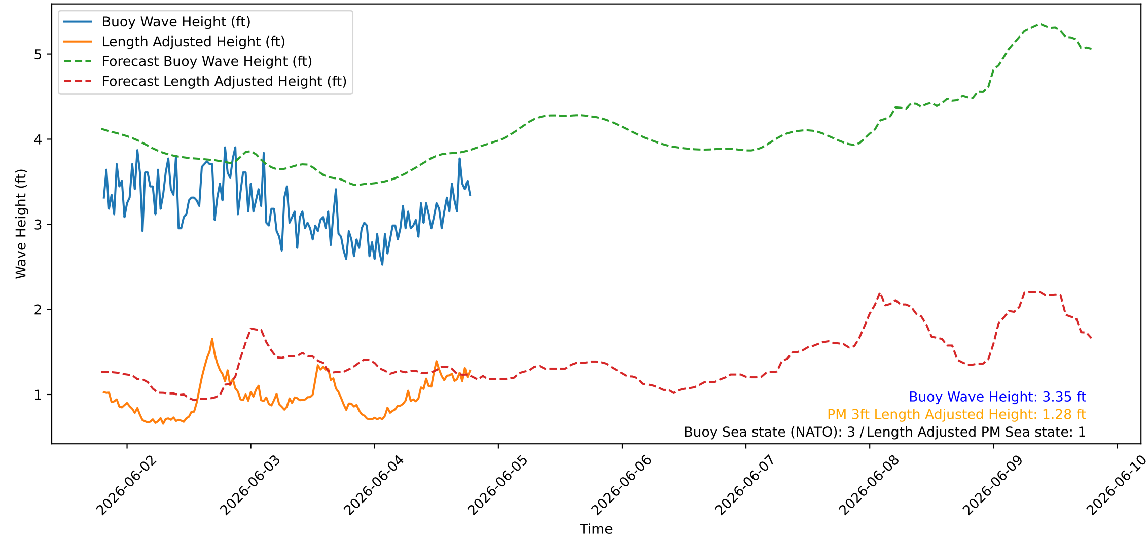
Wave Heights over Time for Red Beach at 2026-06-04 19:20:46
