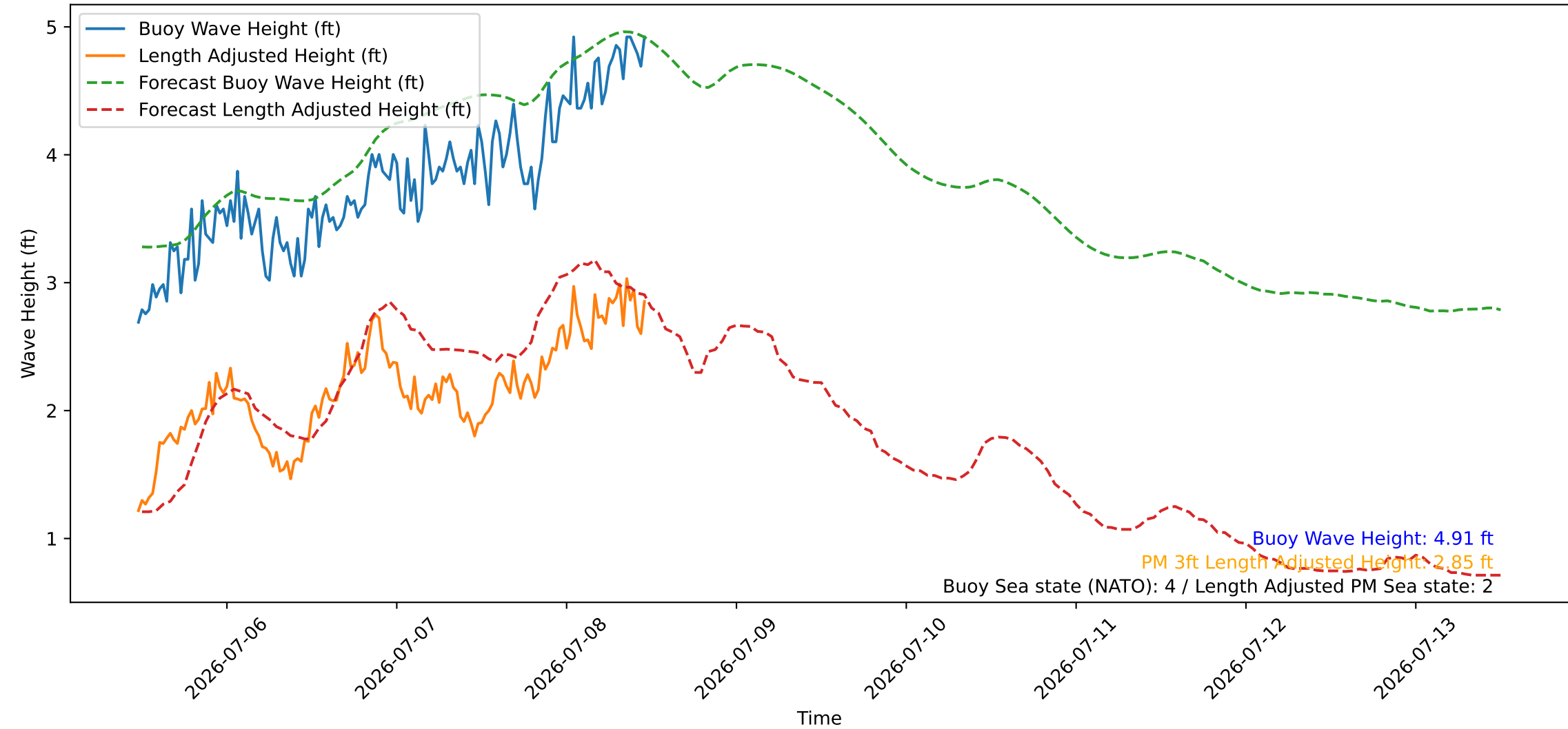
Wave Heights over Time for Oceanside Harbor at 2026-07-08 11:30:27
