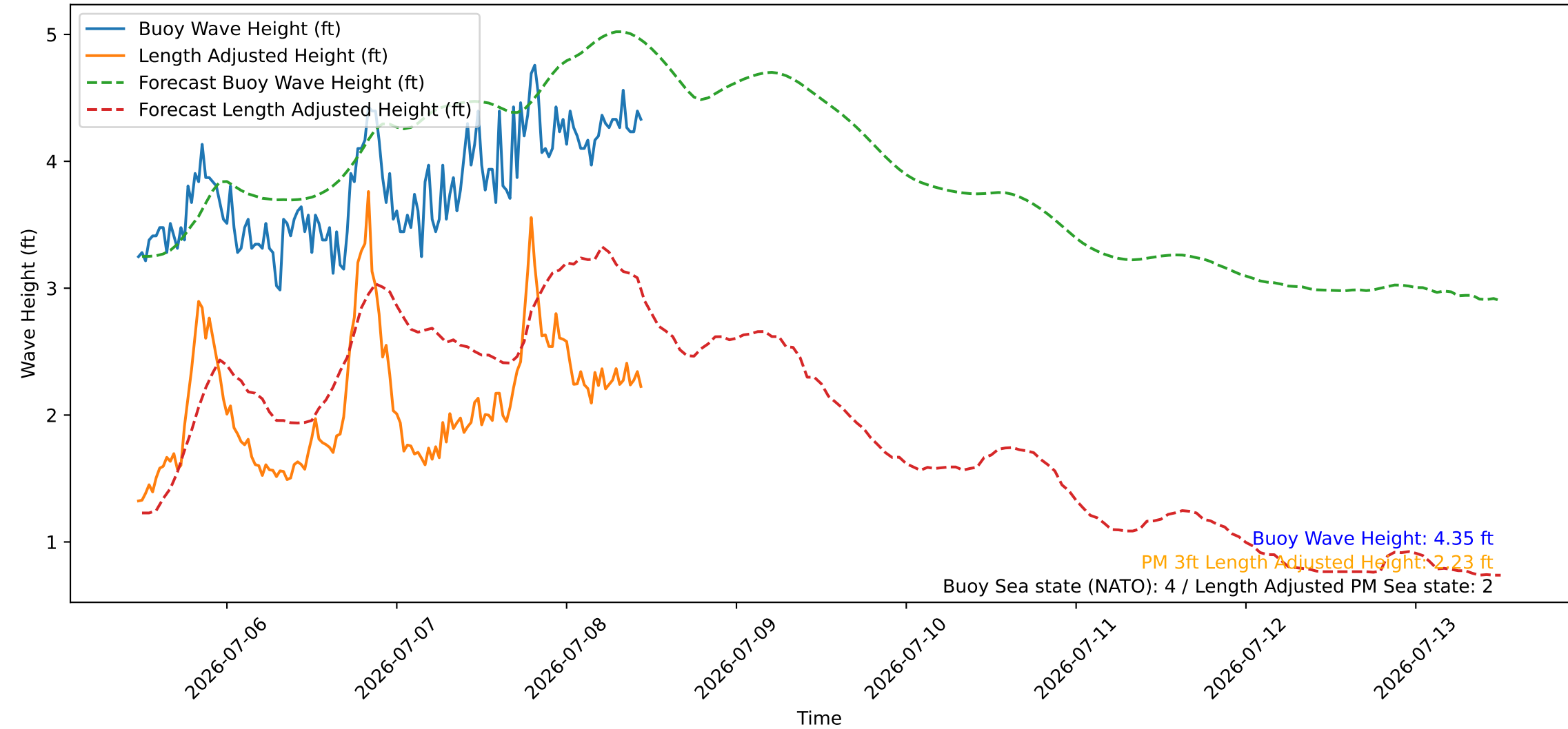
Wave Heights over Time for Green Beach at 2026-07-08 11:31:09
