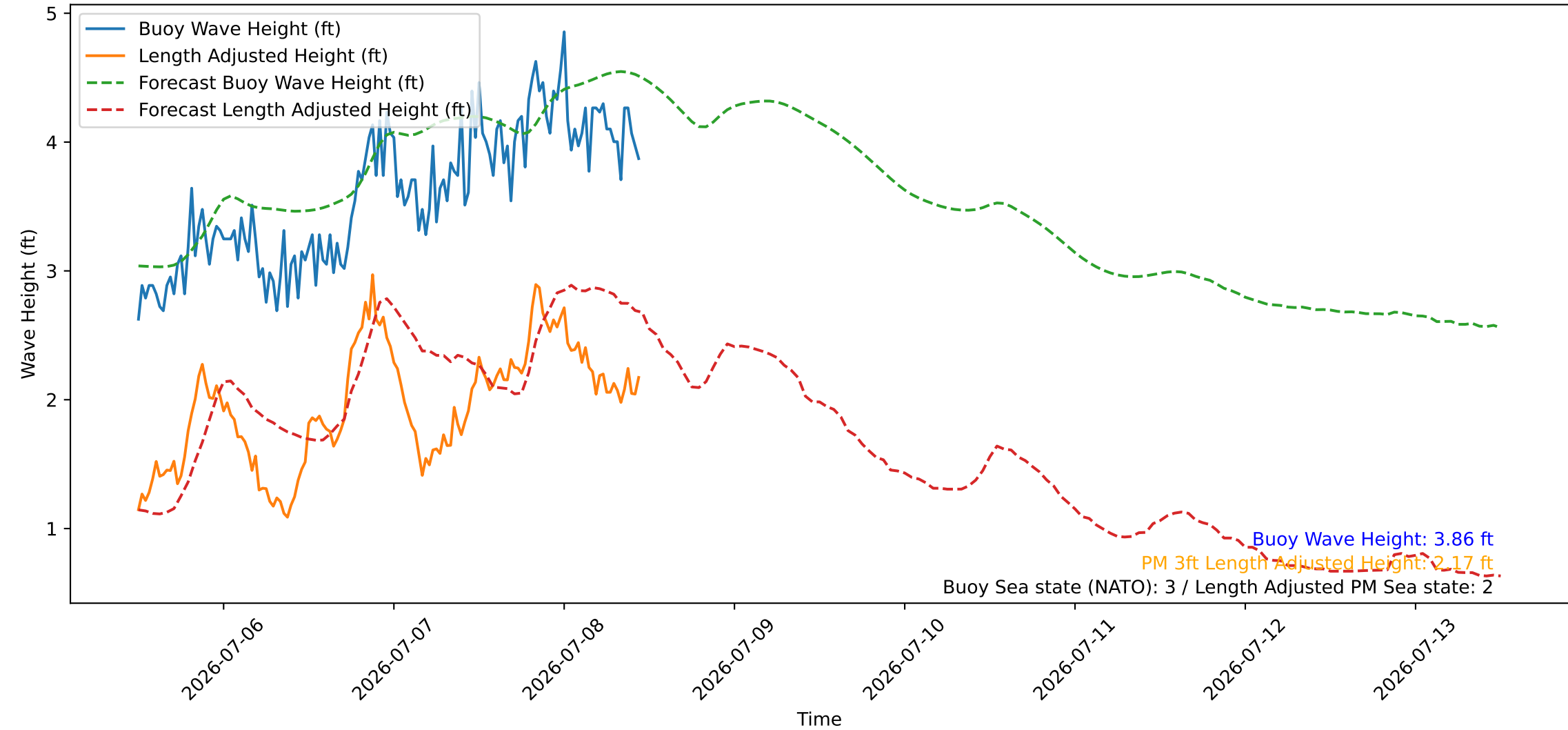
Wave Heights over Time for Red Beach at 2026-07-08 11:30:47
