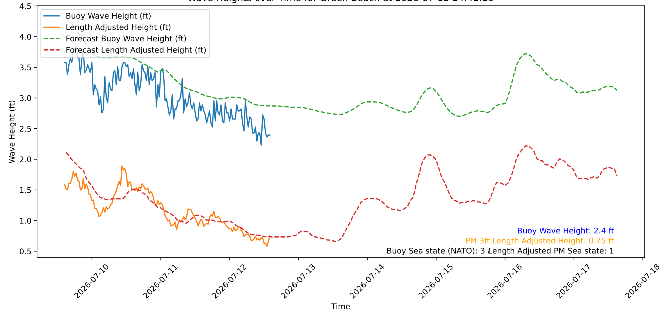
Wave Heights over Time for Green Beach at 2026-07-12 14:41:10
