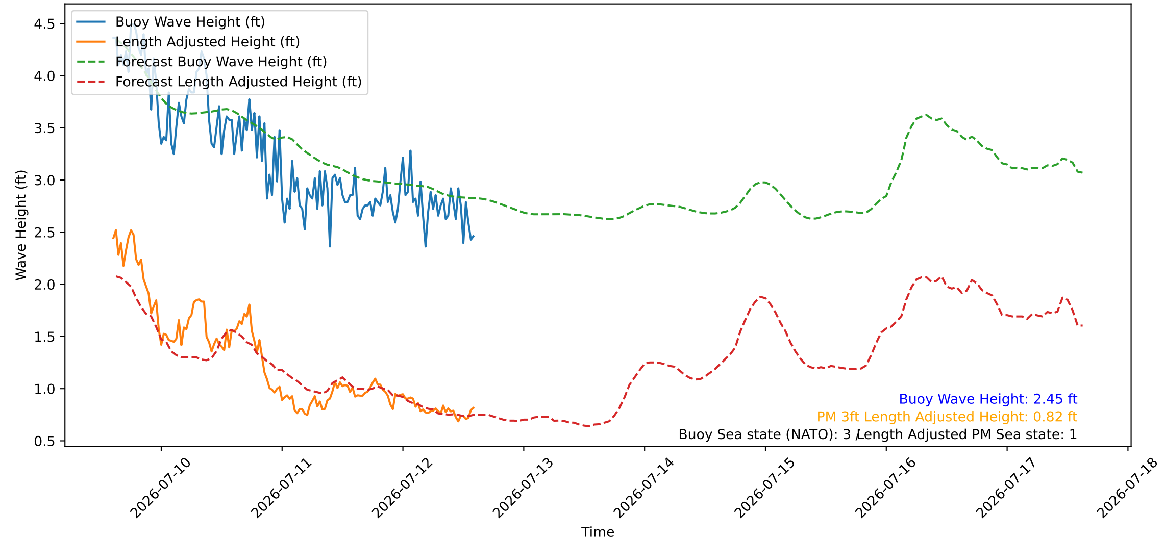
Wave Heights over Time for Oceanside Harbor at 2026-07-12 14:40:26
