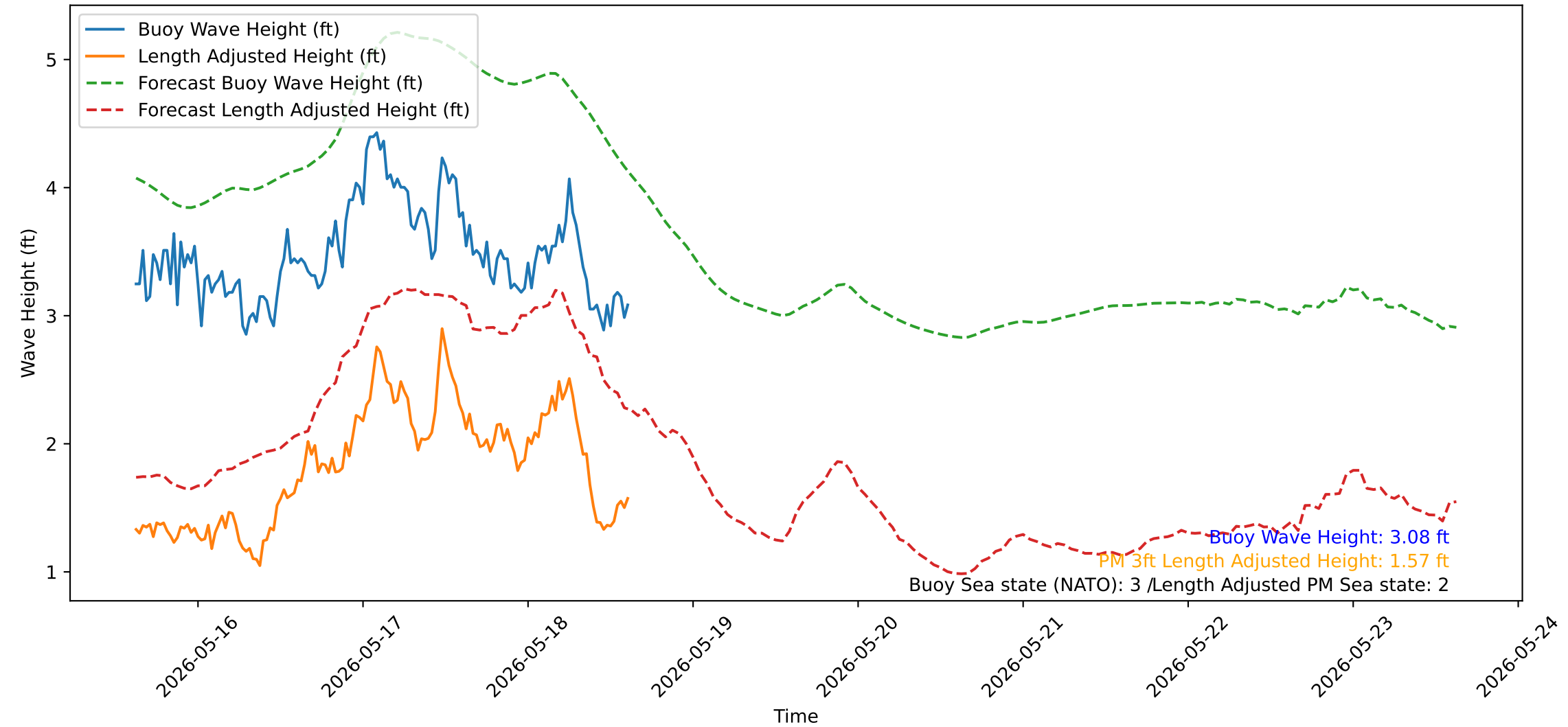
Wave Heights over Time for Green Beach at 2026-05-18 15:11:14
