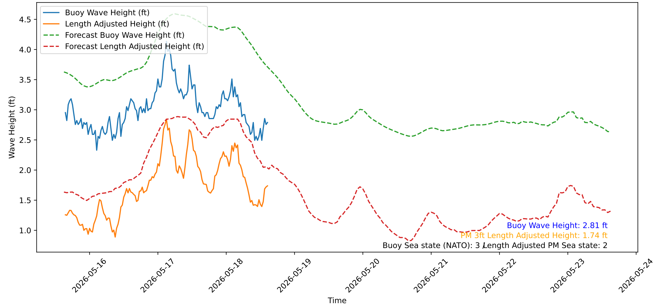
Wave Heights over Time for Red Beach at 2026-05-18 15:10:51
