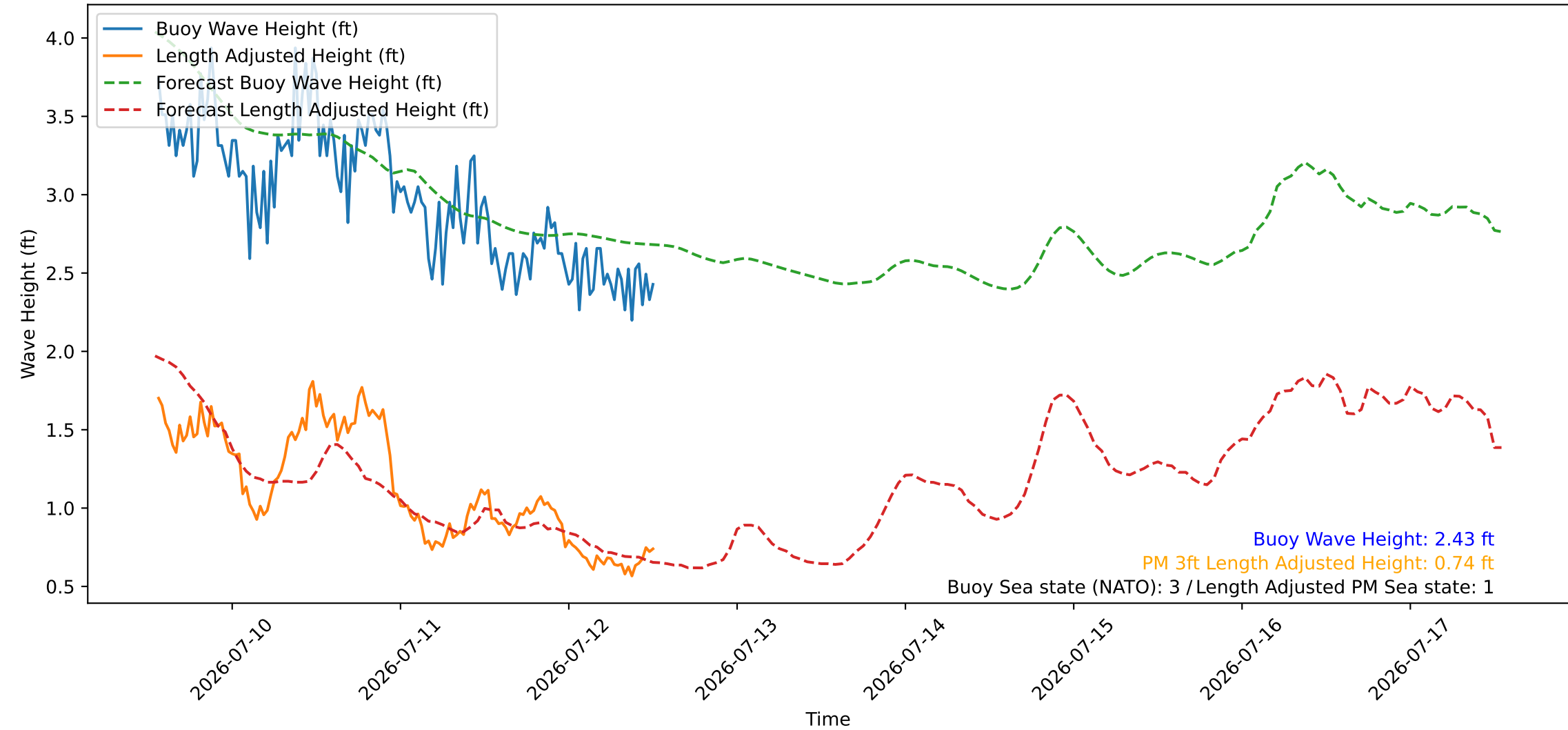
Wave Heights over Time for Red Beach at 2026-07-12 13:00:46
