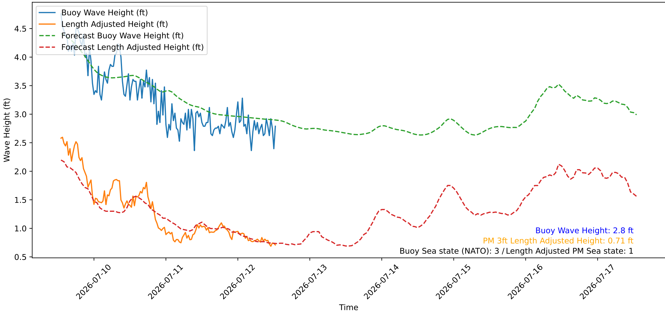
Wave Heights over Time for Oceanside Harbor at 2026-07-12 13:00:26
