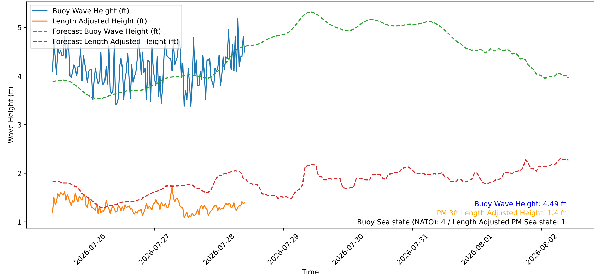
Wave Heights over Time for Green Beach at 2026-07-28 10:11:08
