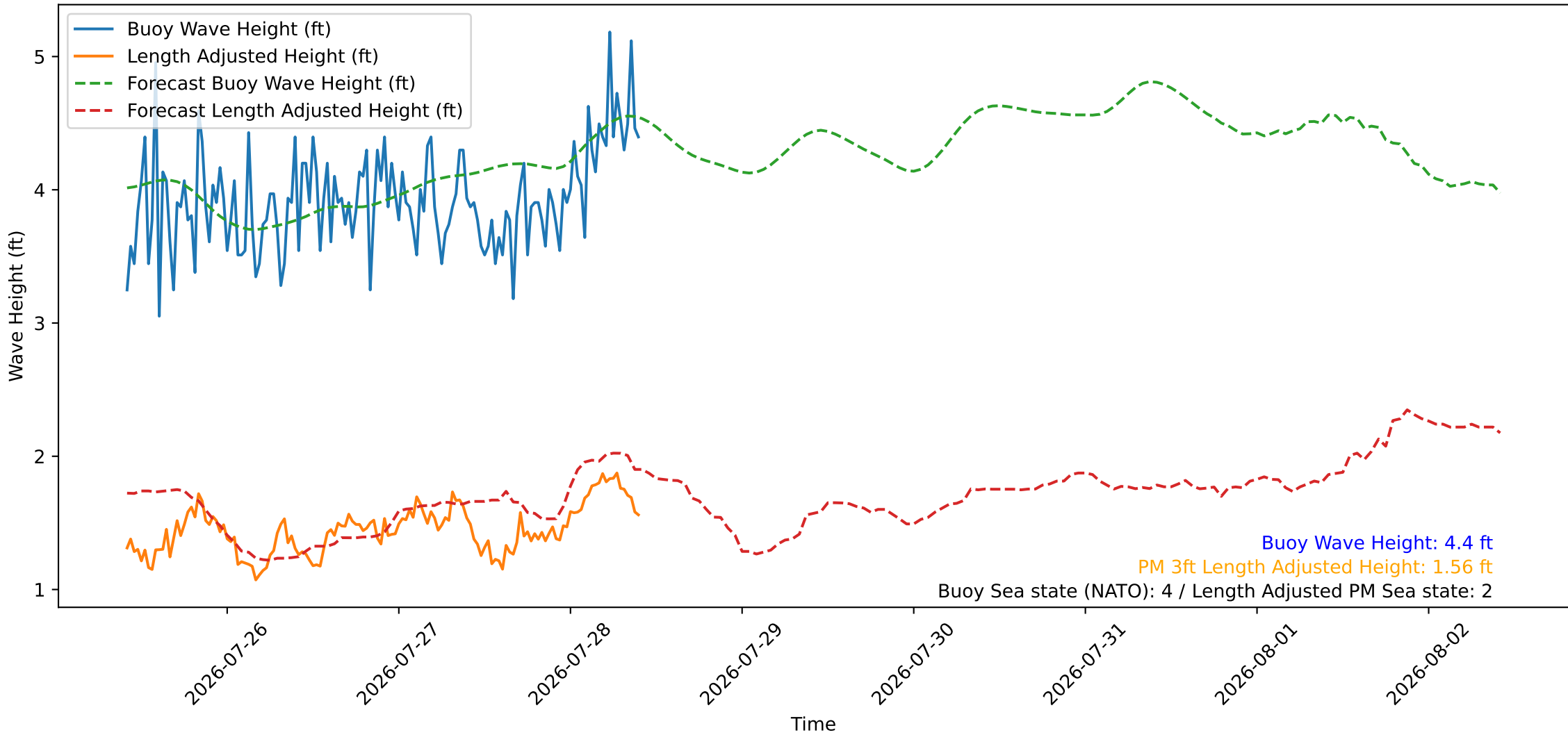
Wave Heights over Time for Oceanside Harbor at 2026-07-28 10:10:26
